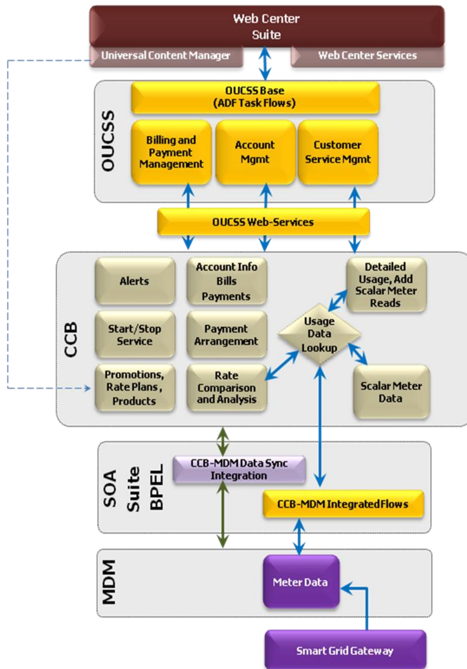
OUCSS Architecture diagram with CCB-MDM integrated flows
