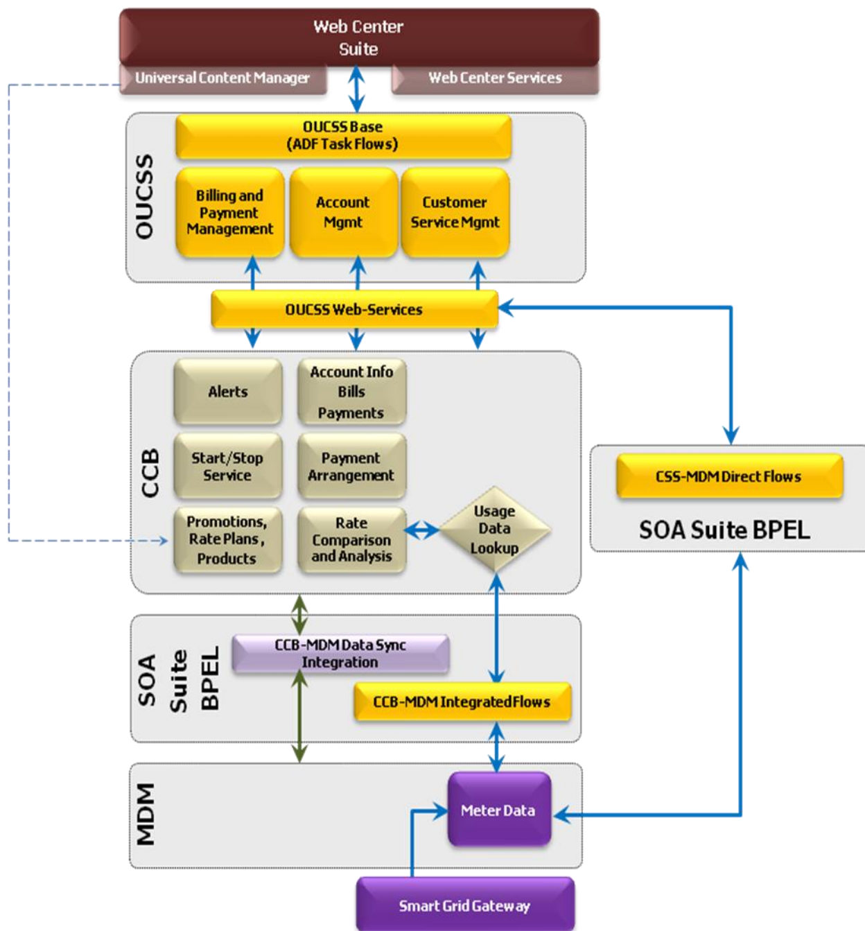
OUCSS Architecture diagram with CSS-MDM direct flows
