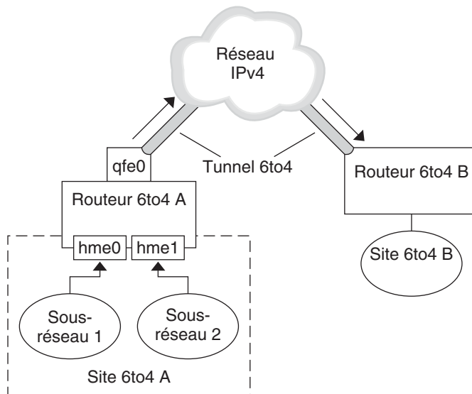
FIGURE 11-6 Tunnel entre deux sites 6to4
