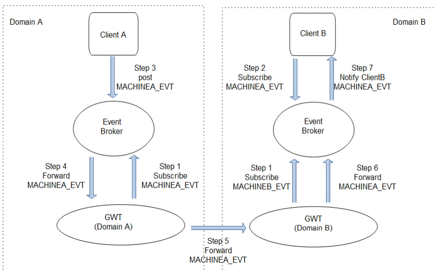
Figure 6-2 Cross Domain Event Overall Flow
