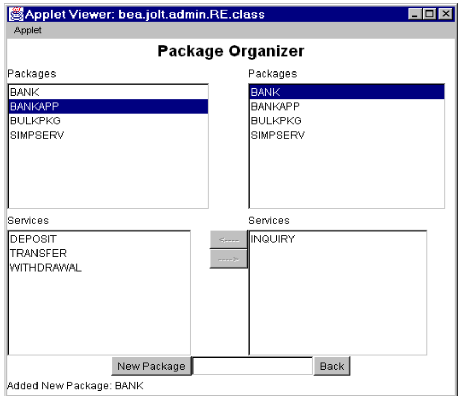
Figure 4-15 Example of a Moved Service
