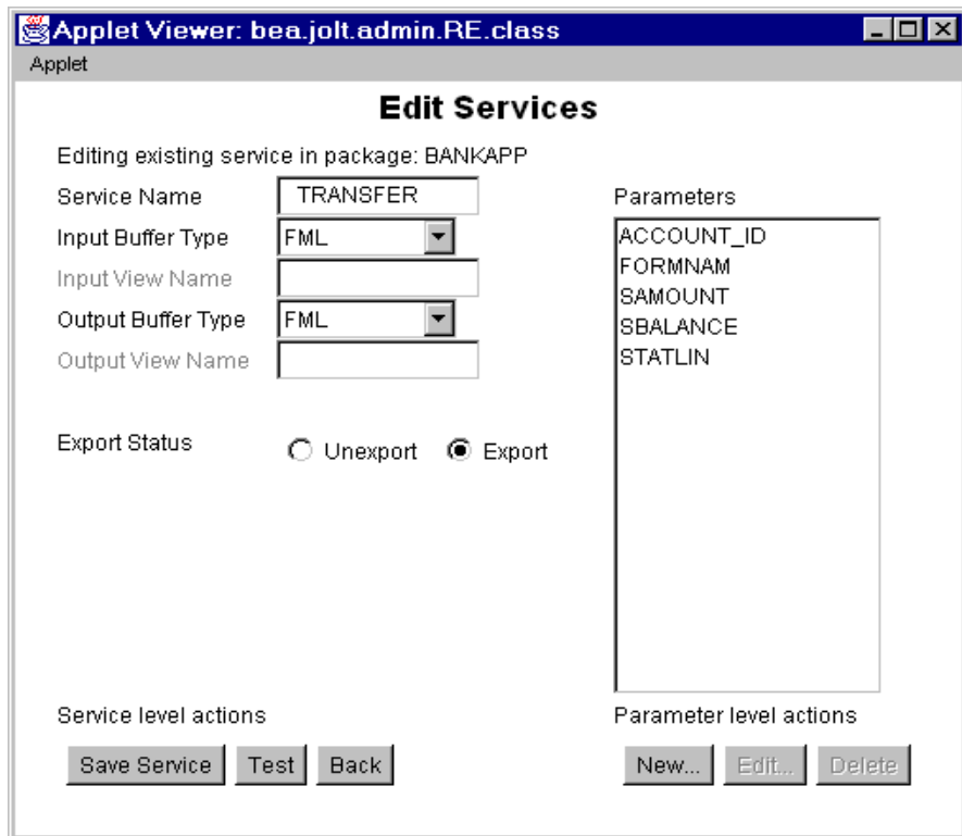
Figure 4-16 Edit Services Window
