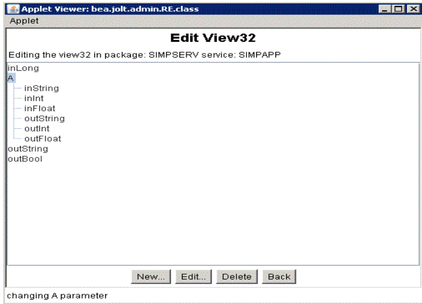
Figure 4-13 Edit View32 Window
