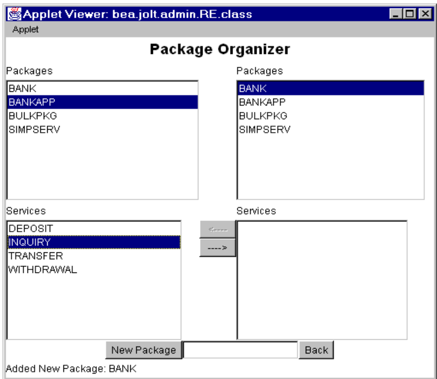
Figure 4-14 Package Organizer Window
