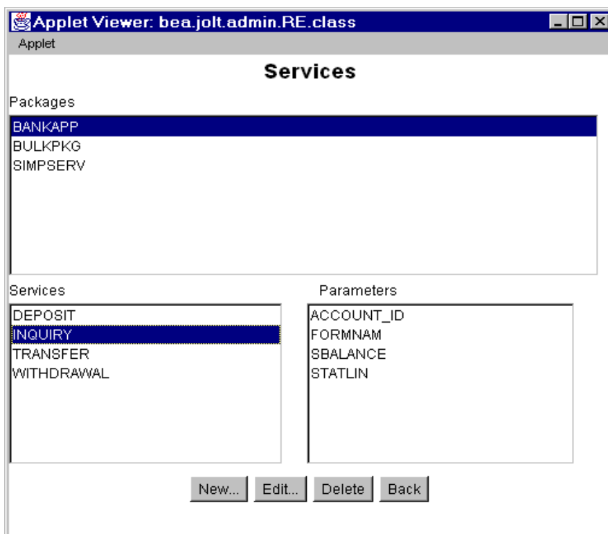
Figure 4-7 Sample Services Window with Parameters List
