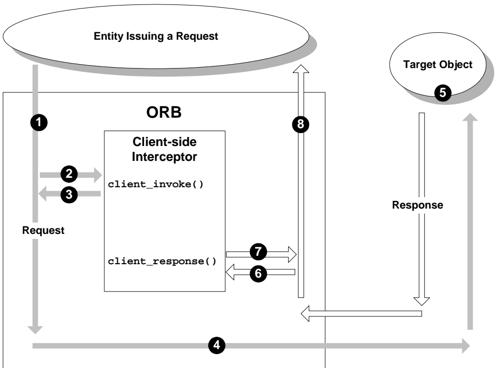
Figure 1-1 Client-side Interceptor
