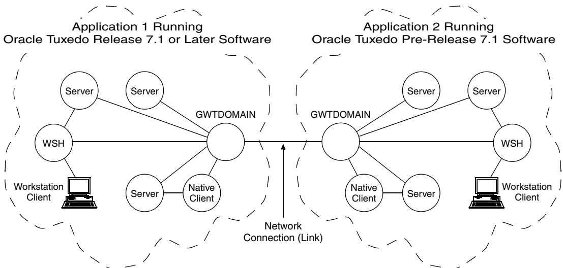
Figure 1-12 Inter-Domain Interoperability
