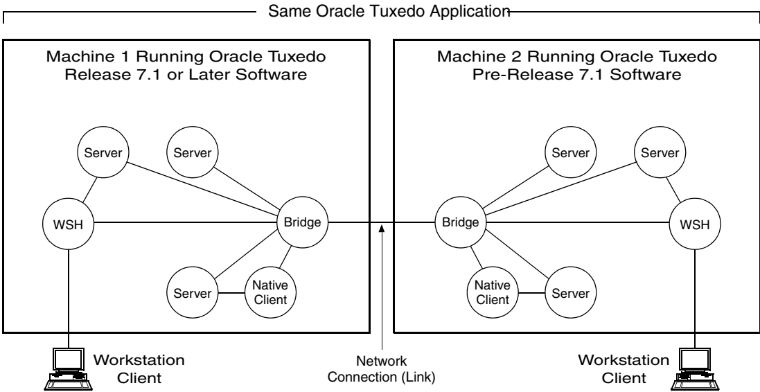
Figure 1-13 Intra-Domain Interoperability
