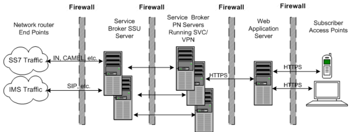
Figure 2–5 Service Broker SVC/VPN Security Overview
