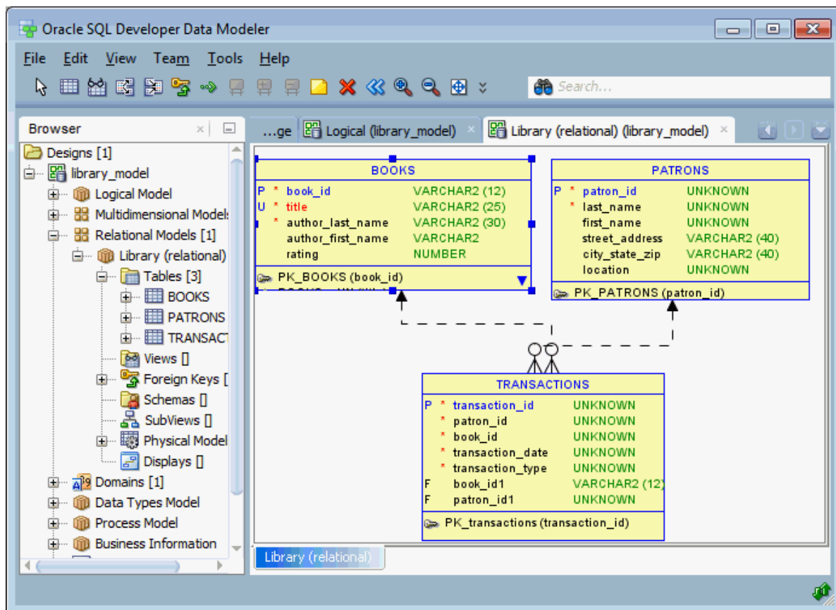
Figure 1-1 SQL Developer Data Modeler Main Window
