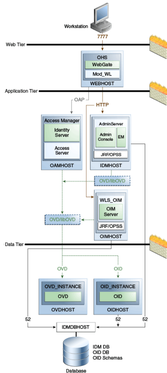
Figure 1–1 Basic Integration Topology with One Administration Server
