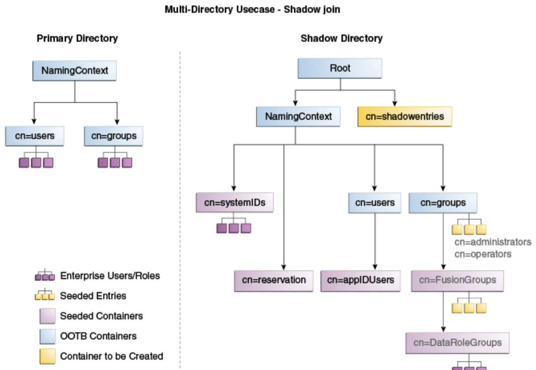
Figure 6-1 Directory Structure
