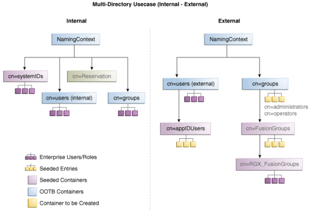
Figure 6-4 Directory Structure
