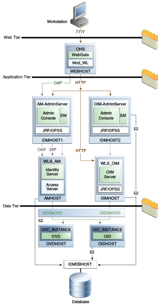
Figure 1–2 Basic Integration Topology with Two Administration Servers
