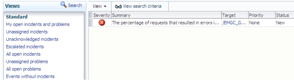
Figure 13 Incident Manager
