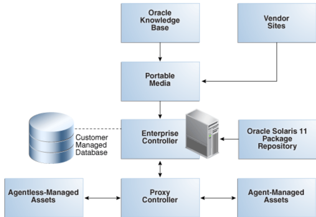
Figure 2–4 Enterprise Controller in Disconnected Mode
