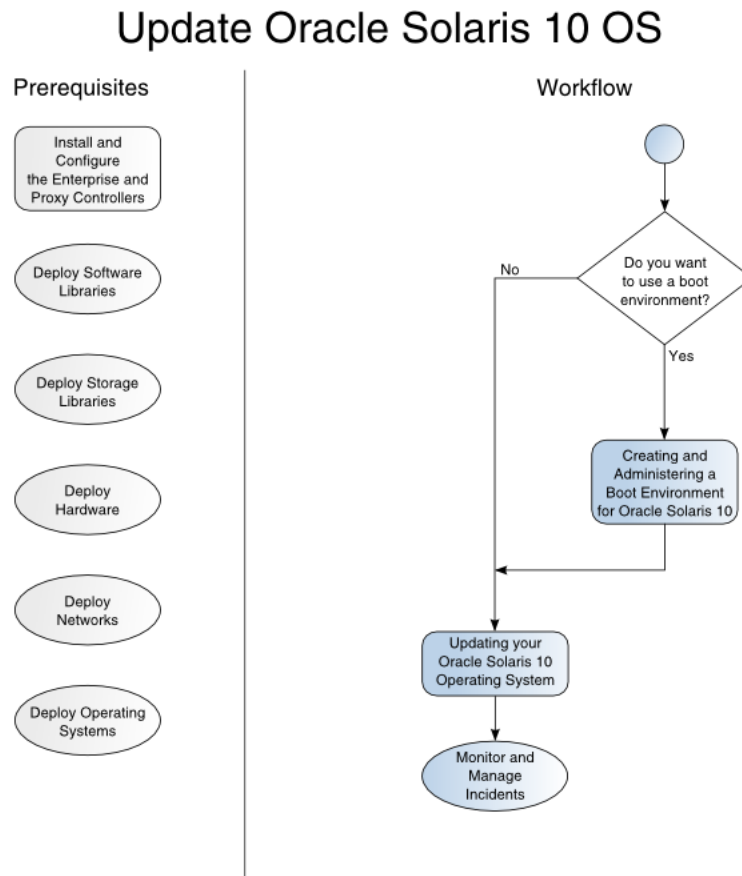
Figure 1 Update Oracle Solaris 10 OS Workflow
