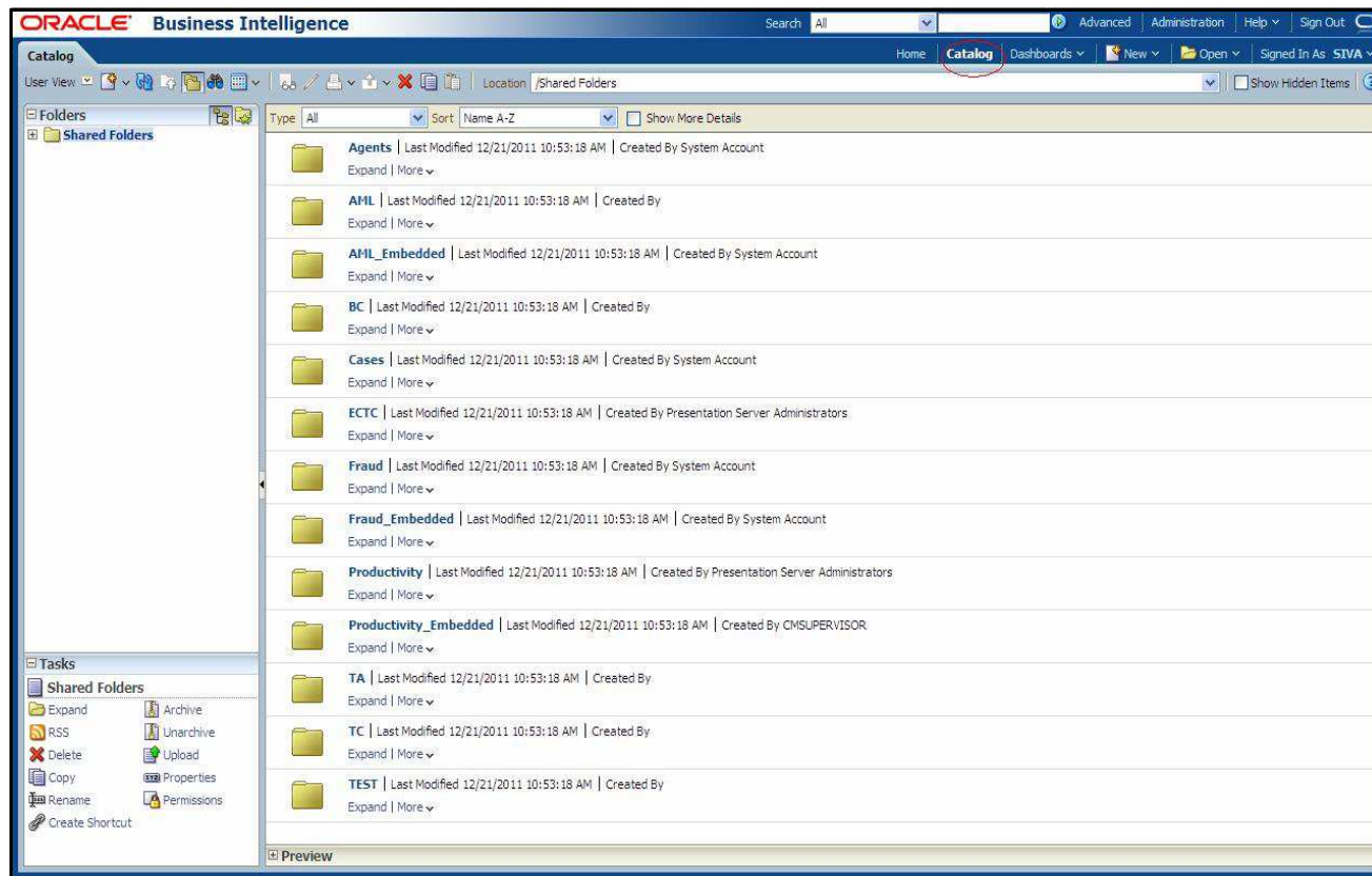
Figure 6. Shared Folder
