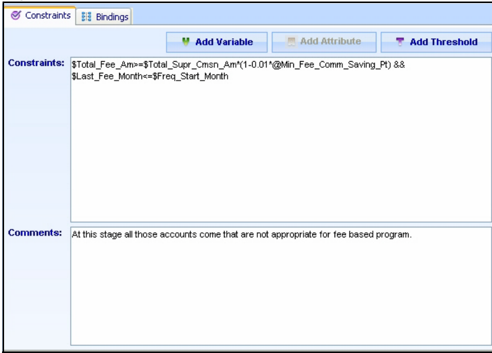
Figure 50. Edit Rule Dialog Box—Constraints Tab
