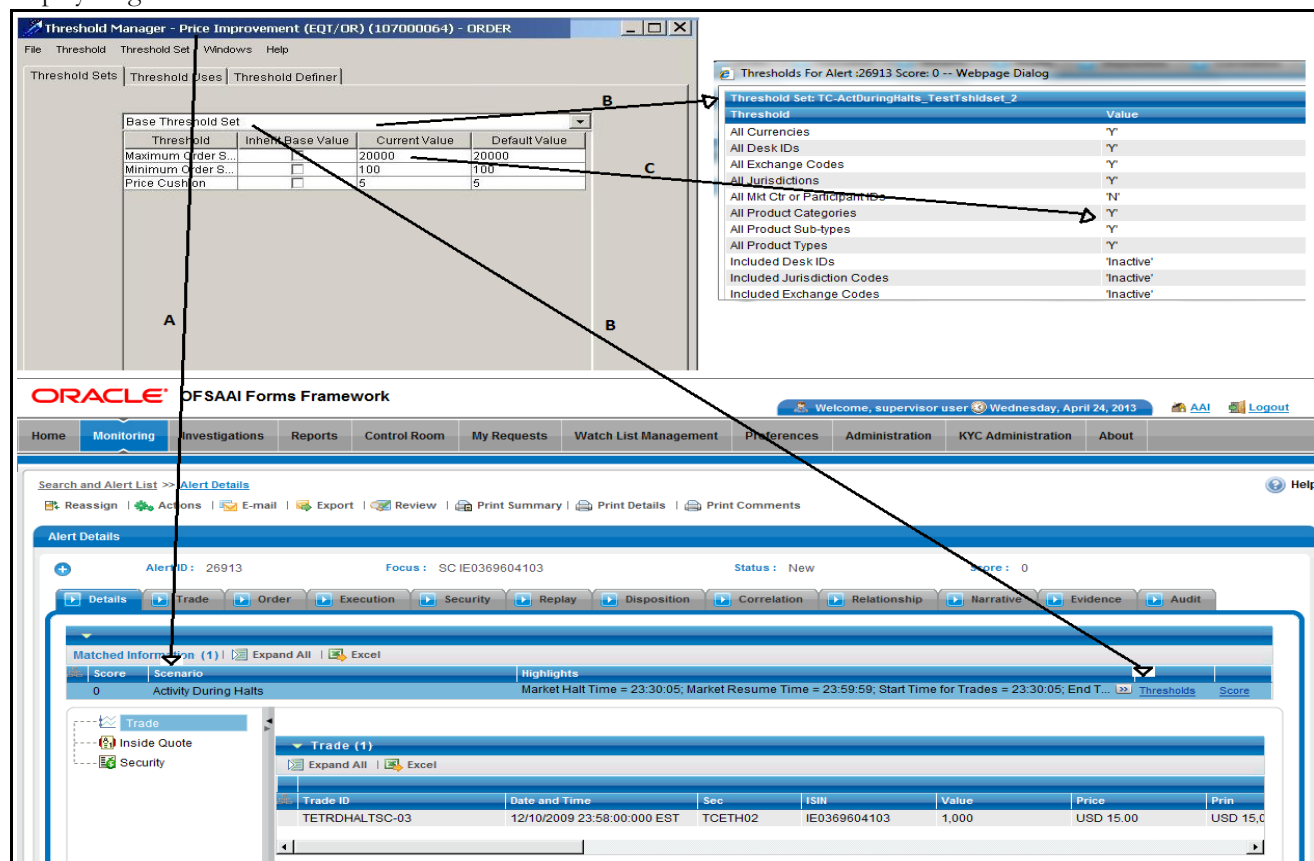
Figure 74. UI Mapping Sample - Threshold Sets Tab to Alert Details
