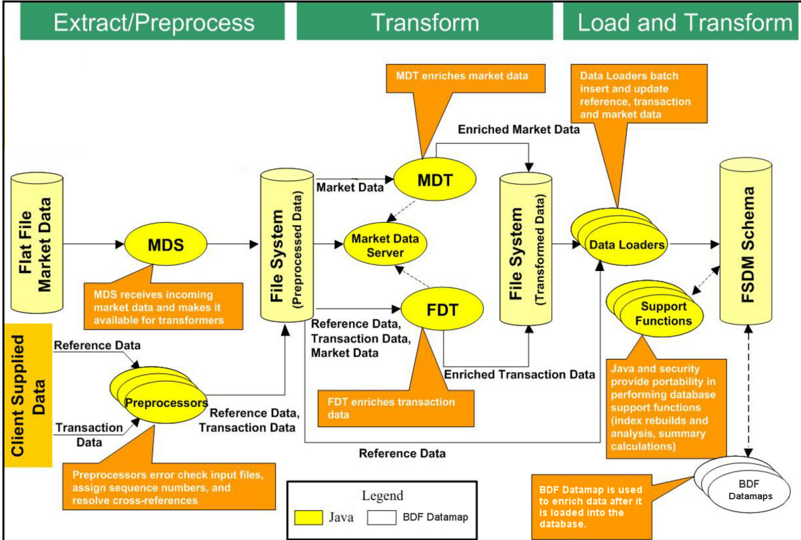
Figure 10. Data Ingestion Subsystem Components Workflow
