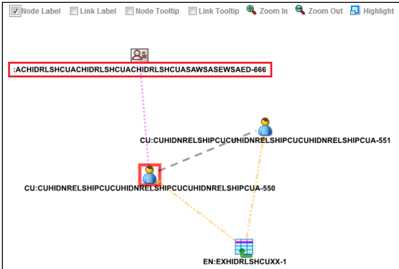
Figure 22. Network Graph
