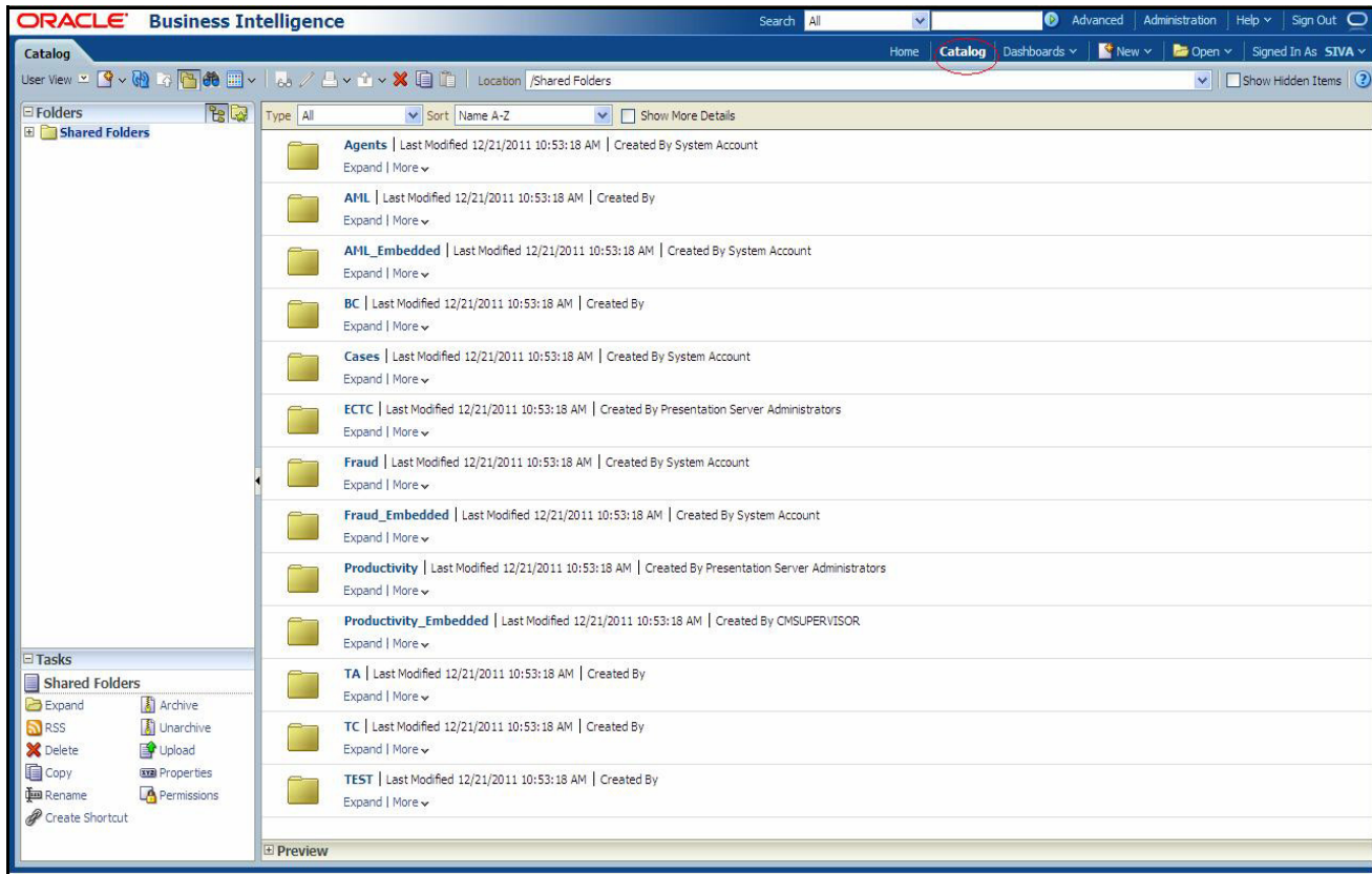
Figure 6. Shared Folder
