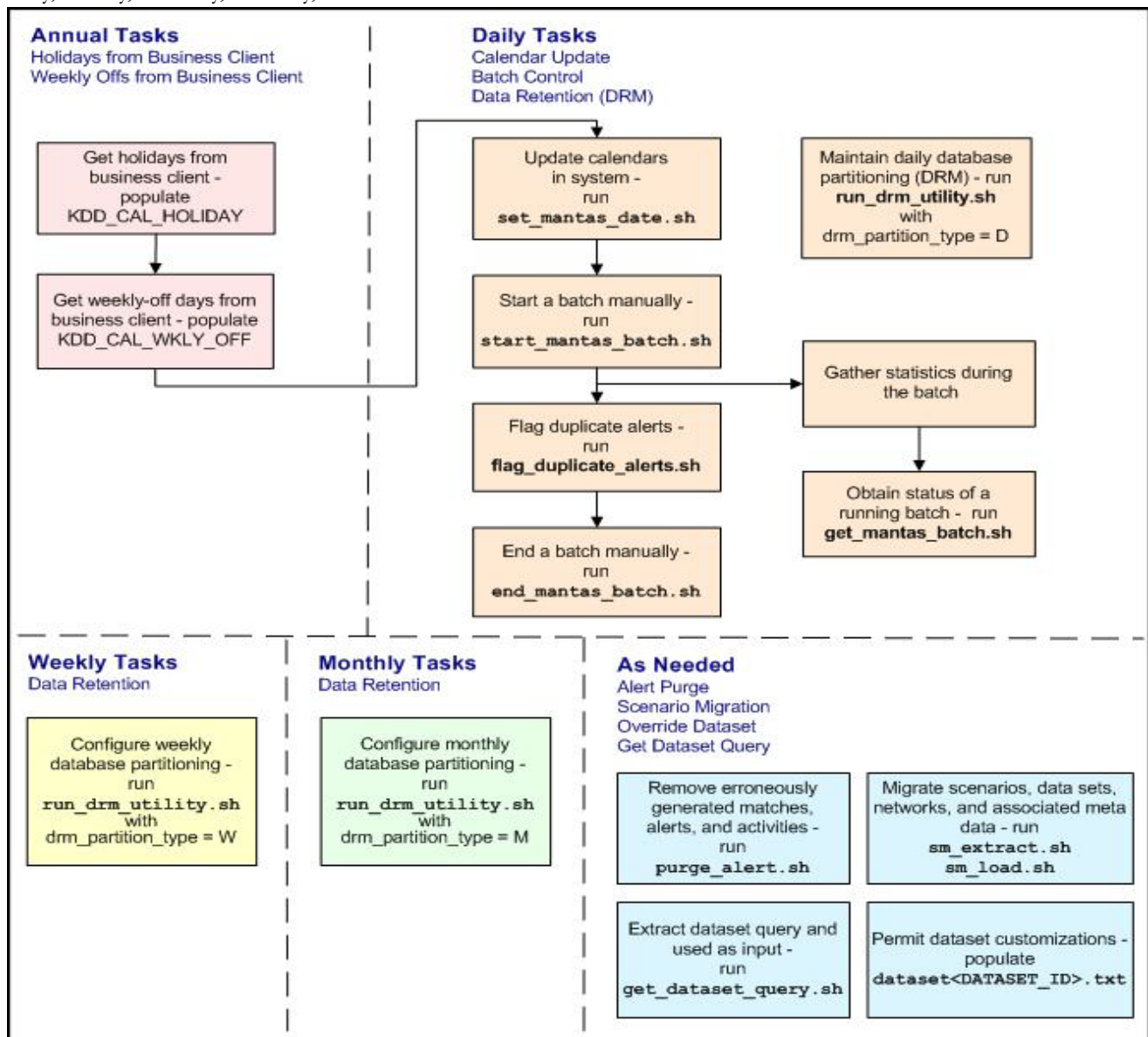
Figure 25. Managing Database Activities with Utilities
