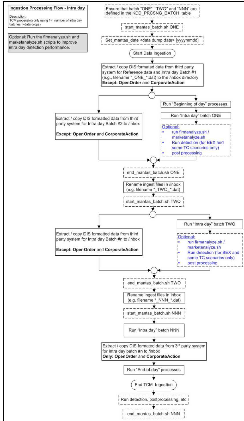
Figure 20. Intra-Day Data Ingestion Processing
