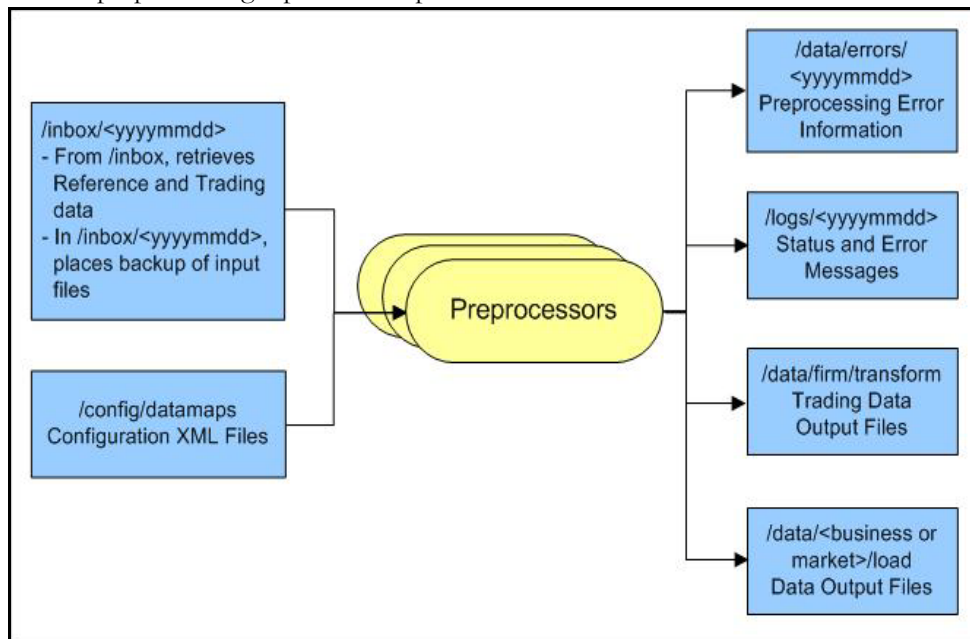
Figure 14. Preprocessing Input and Output Directories
