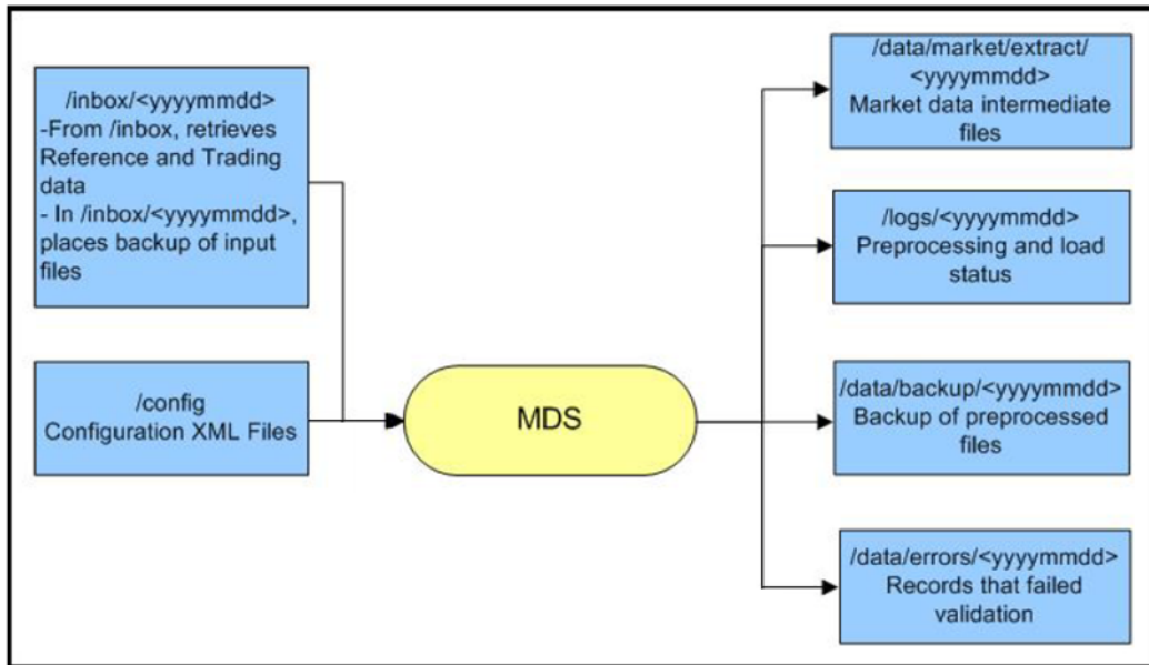
Figure 16. runMDS.sh Input and Output Directories
