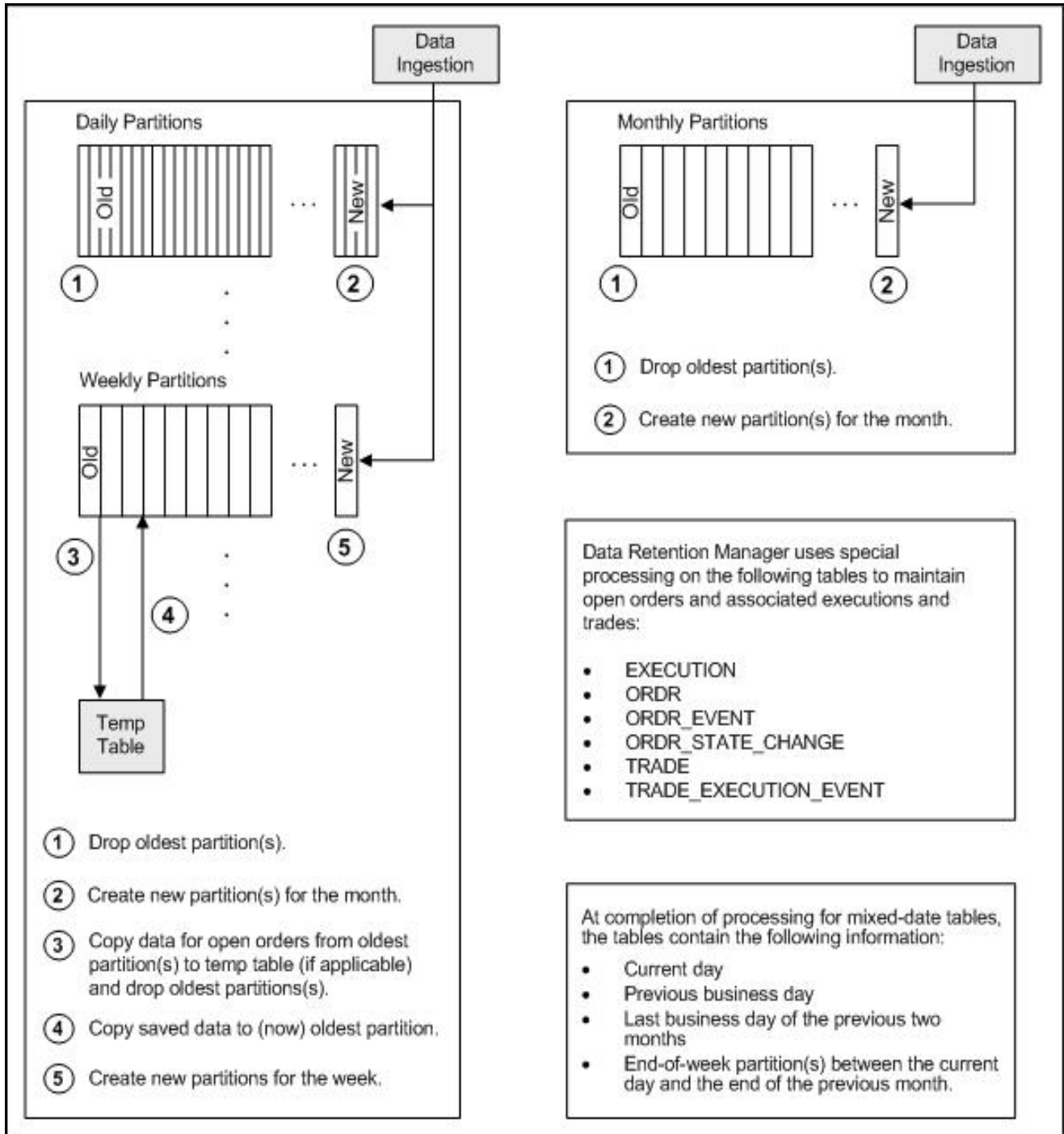
Figure 35. Database Partitioning Process
