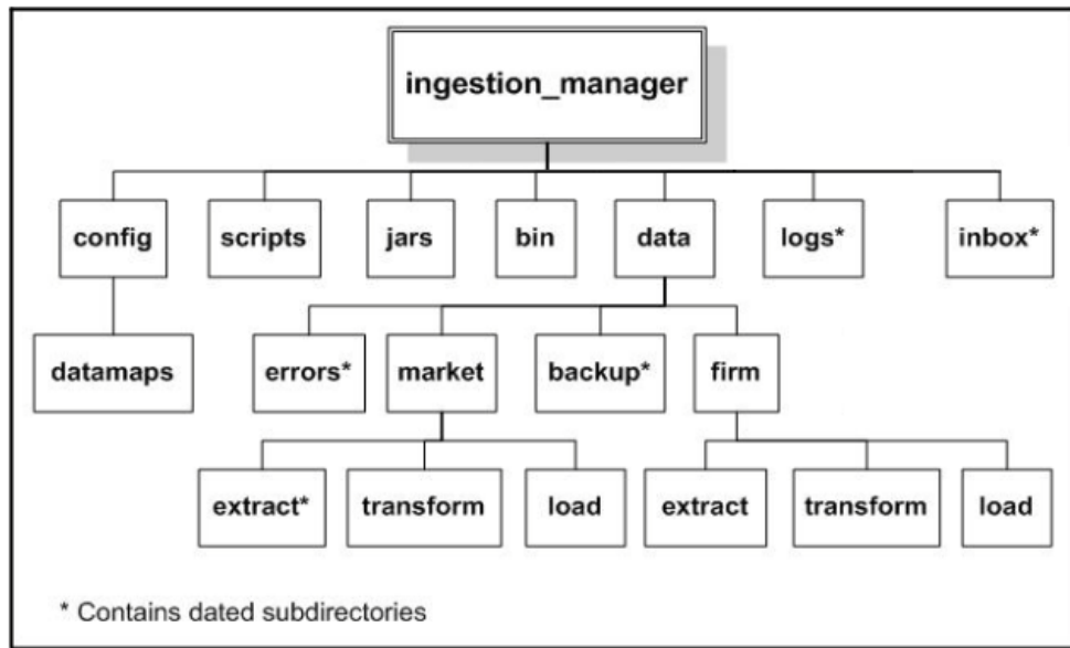
Figure 21. Data Ingestion Subsystem Directory Structure
