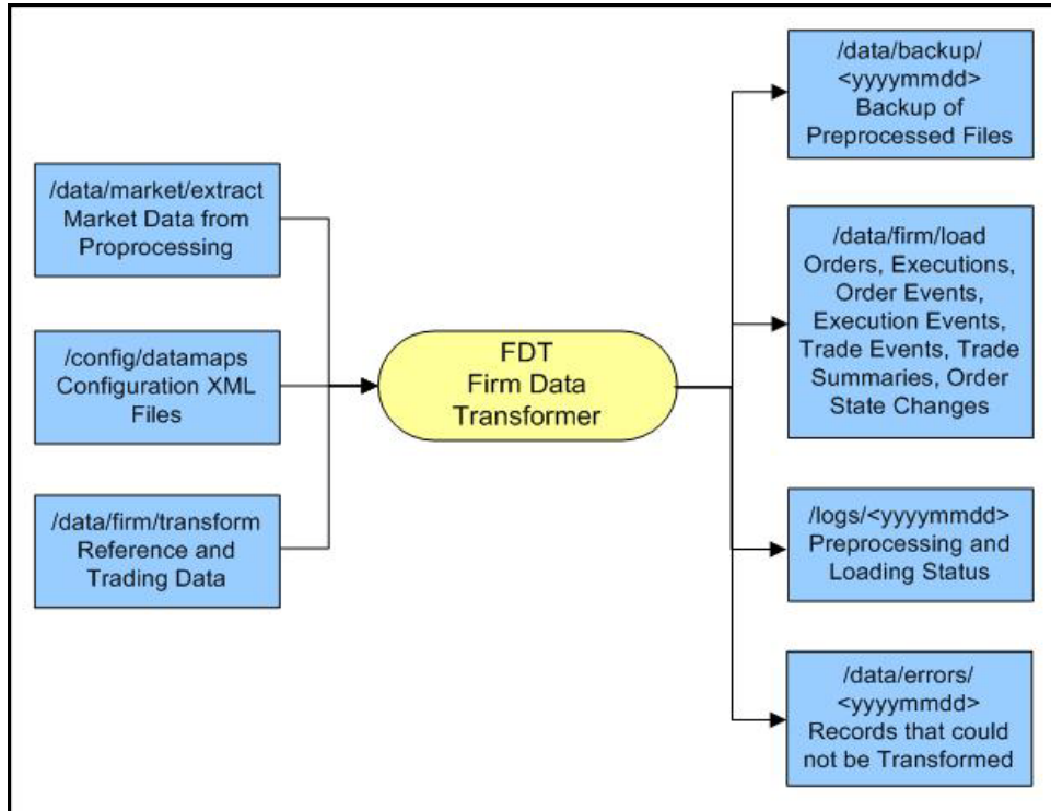
Figure 17. Firm Data Transformer (FDT) Processing
