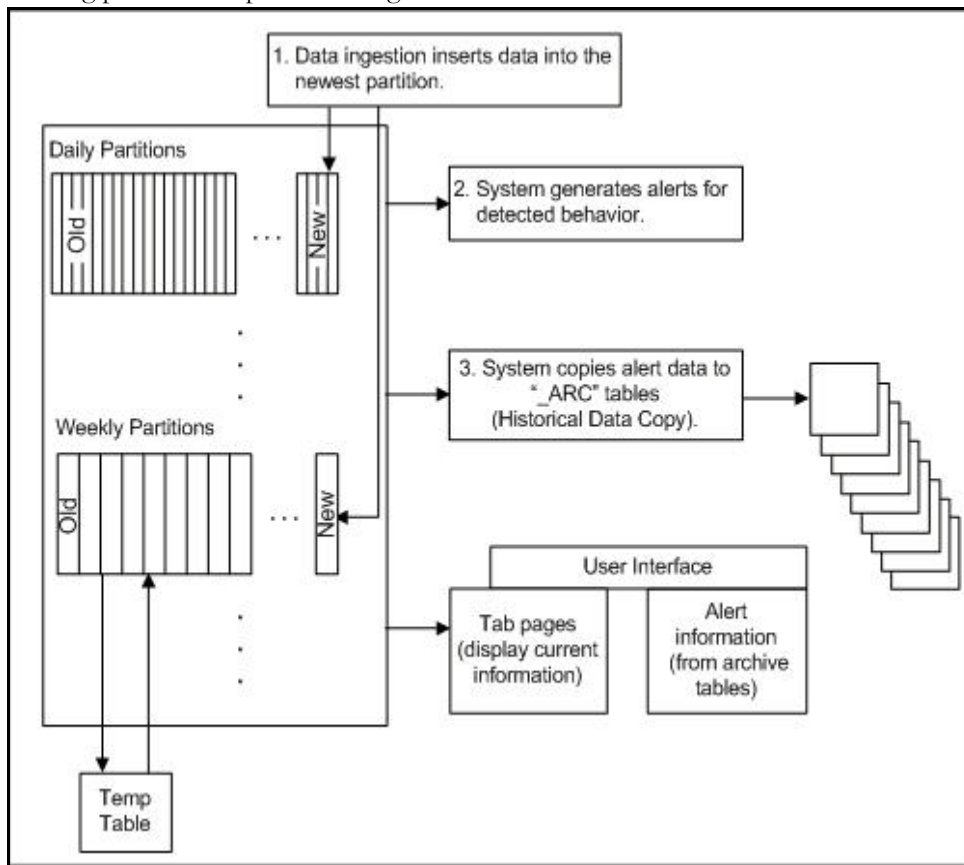
Figure 22. Database Archiving Process
