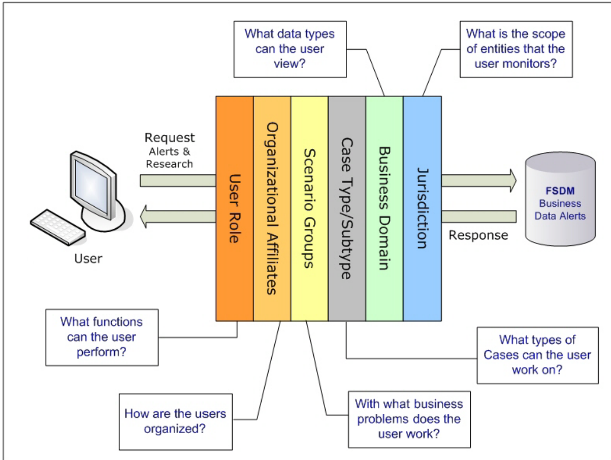
Figure 2. OFSECM User Authorization Model
