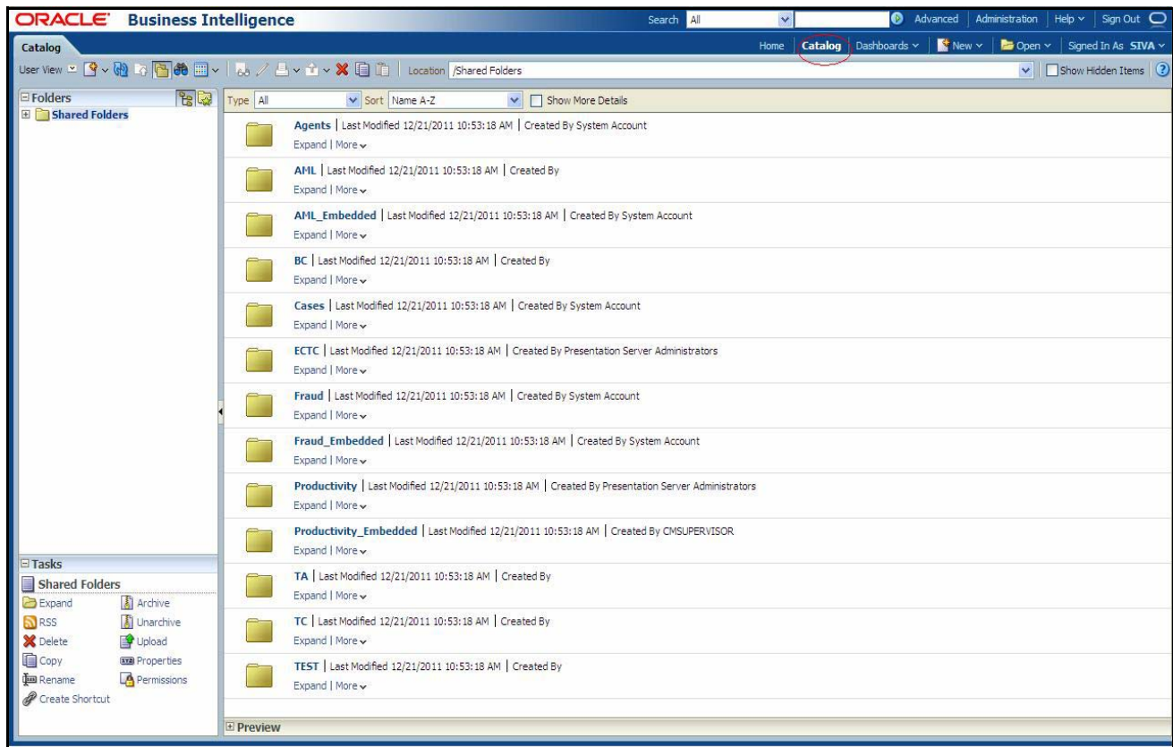
Figure 6. Shared Folder
