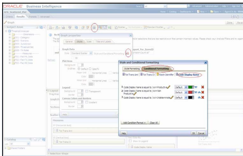
Figure 10. Conditional Formatting
