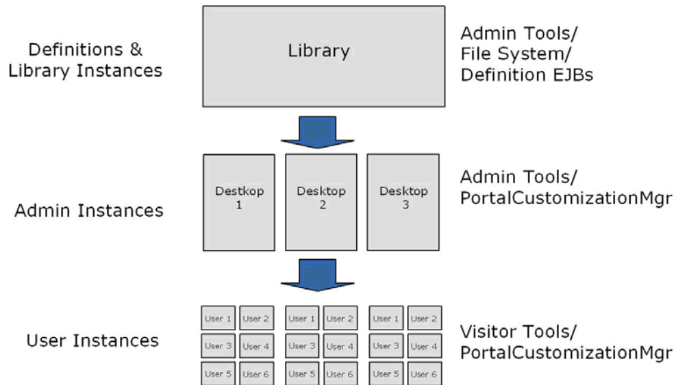
Figure 11–4 Scoping Hierarchy
