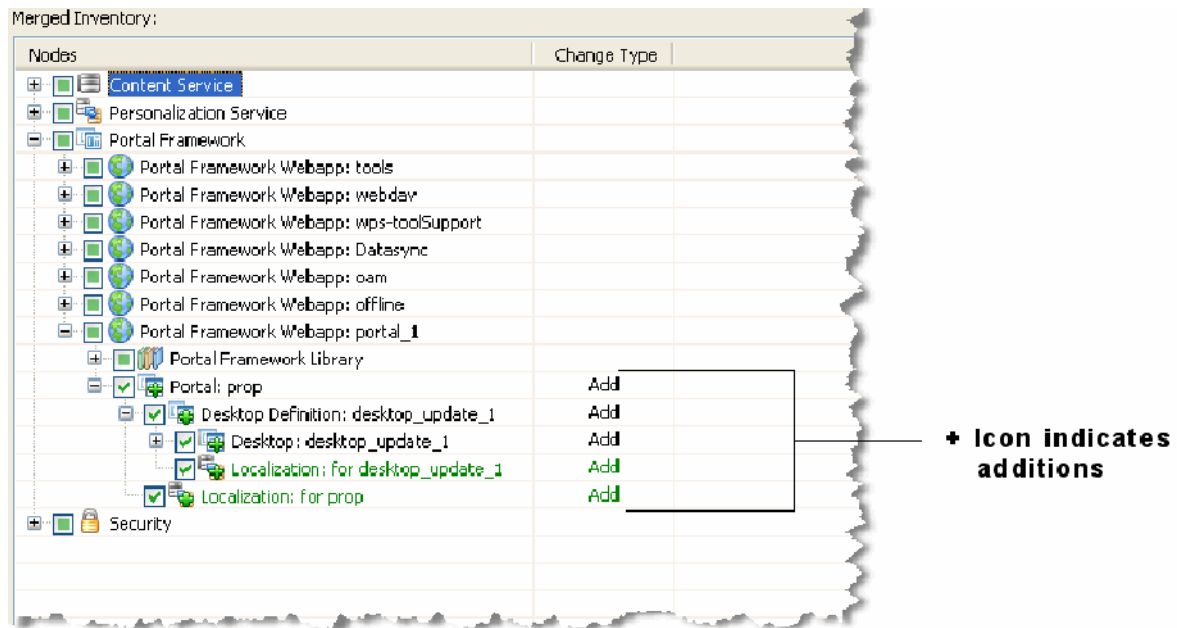
Figure 7–12 Expanded Inventory
