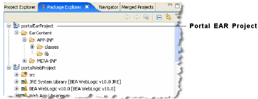
Figure 11–9 Application Name
