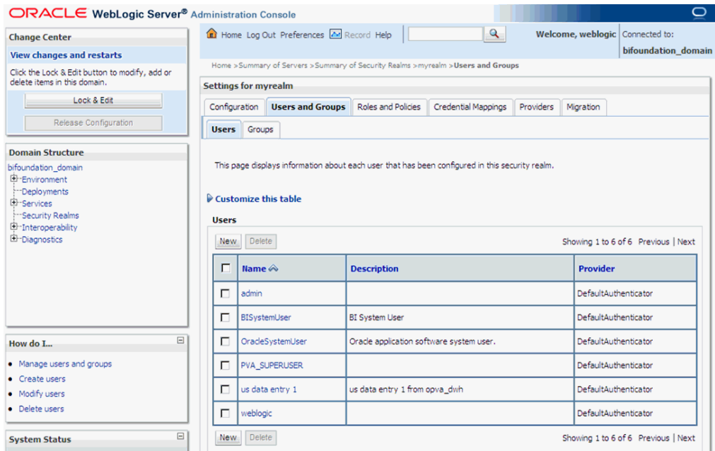
Figure 2–35 myrealm Settings: Users and Groups tab
