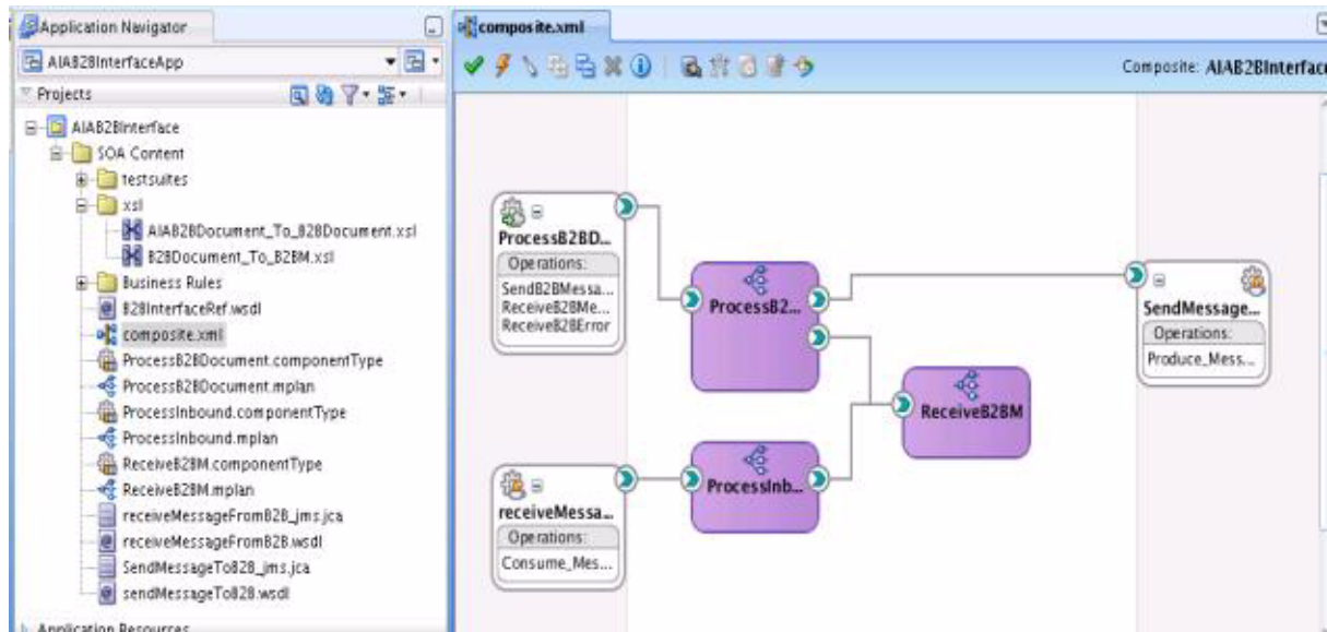
Figure 22–5 composite.xml in Oracle JDeveloper
