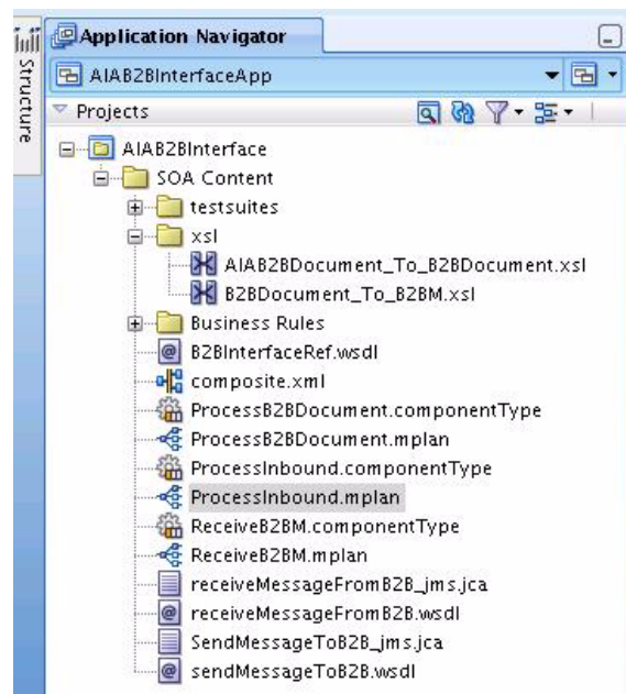
Figure 22–8 ProcessInbound.mplan
