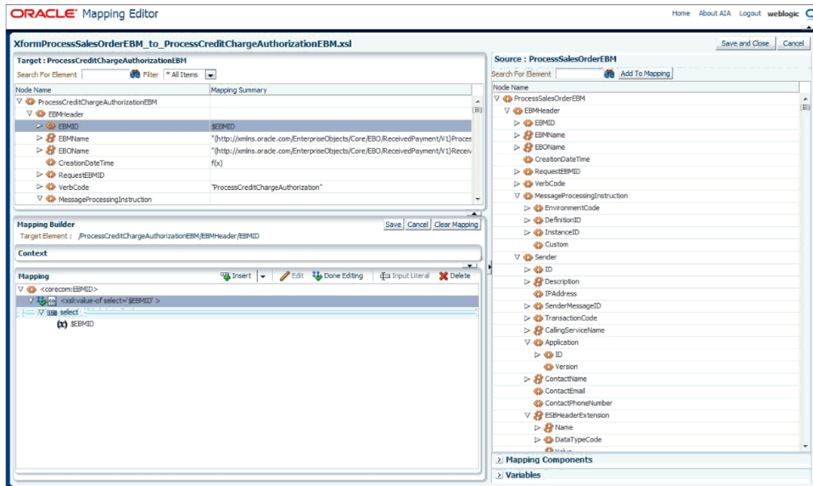
Figure 33–2 Mapping Editor Screen
