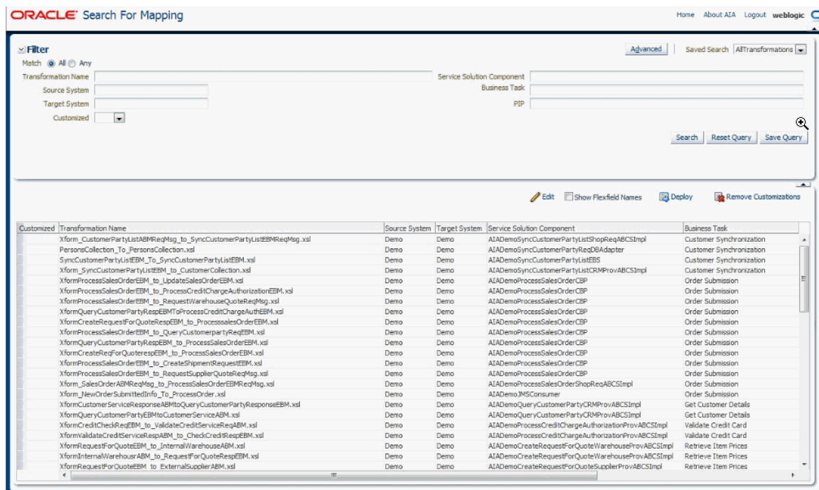
Figure 33–1 Search for Mappings
