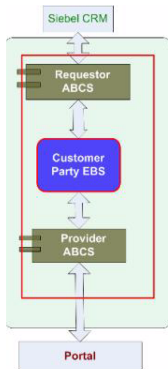
Figure 17-11 Transaction Boundary
