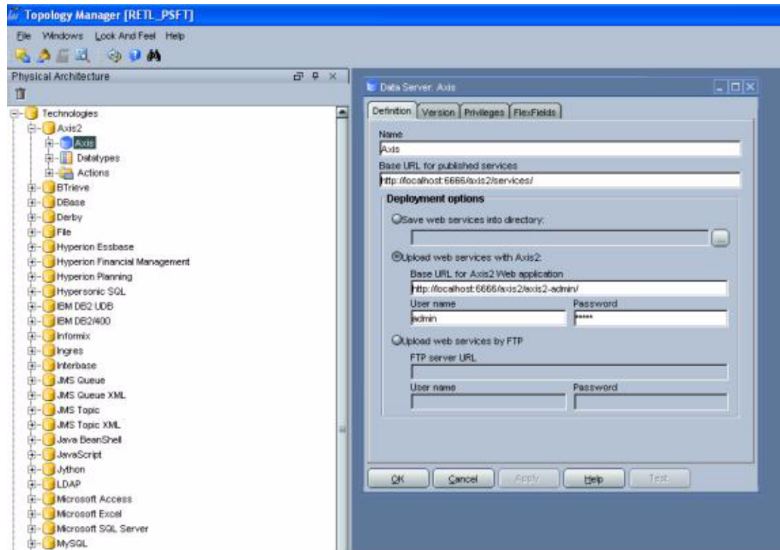
Figure 25–22 Topology Configuration
