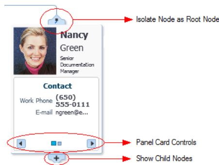
Figure 31–7 Node Controls
