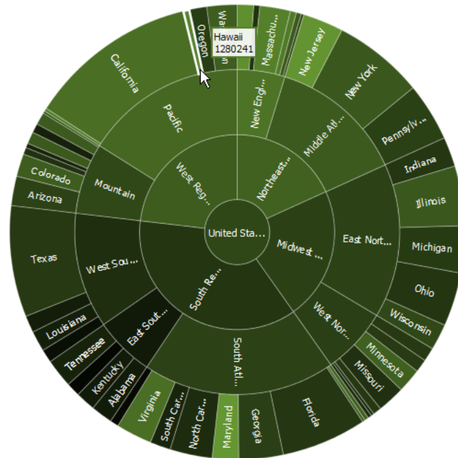
Figure 30–34 Sunburst Tooltip
