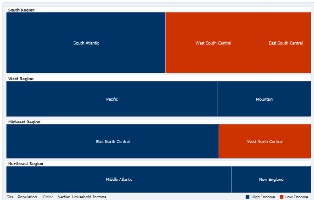
Figure 30–19 Sorted Treemap
