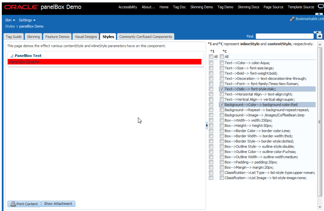
Figure 1-6 Styles Demonstration
