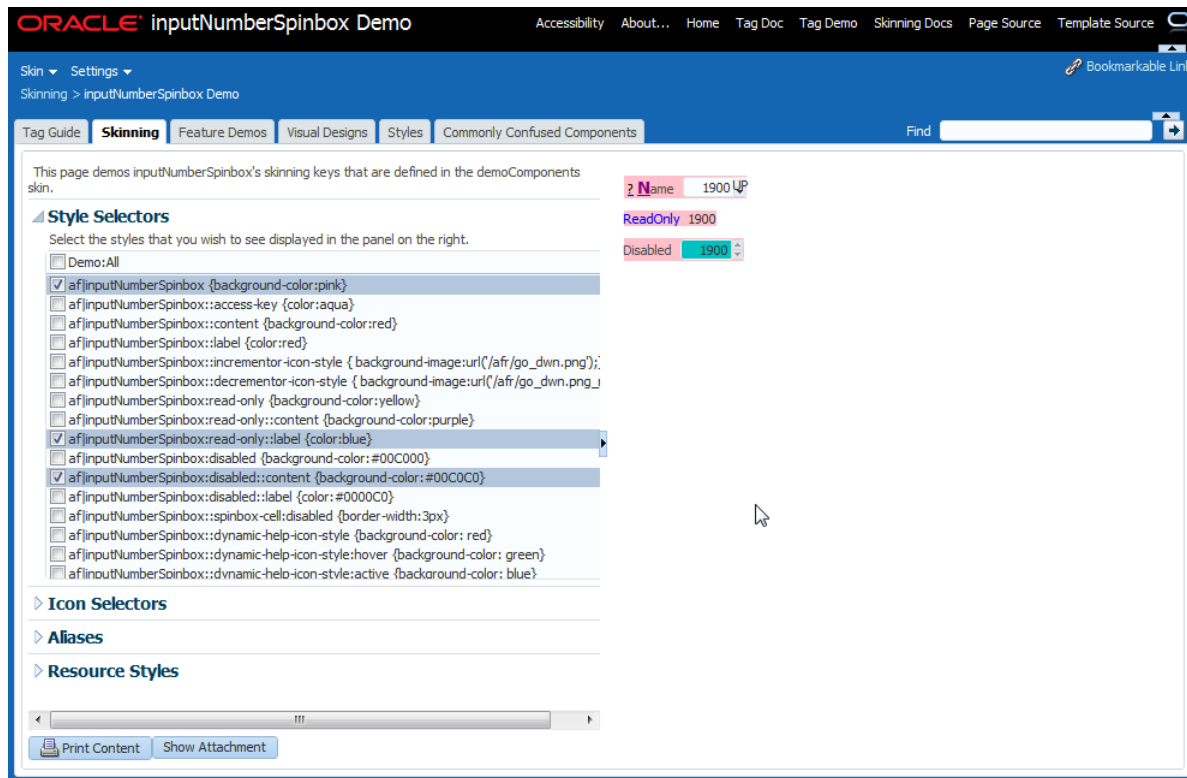
Figure 1–2 Skinning Demonstration
