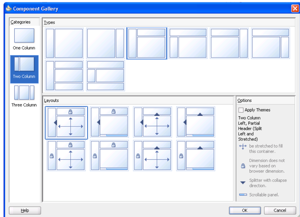
Figure 8-5 Quick Layouts
