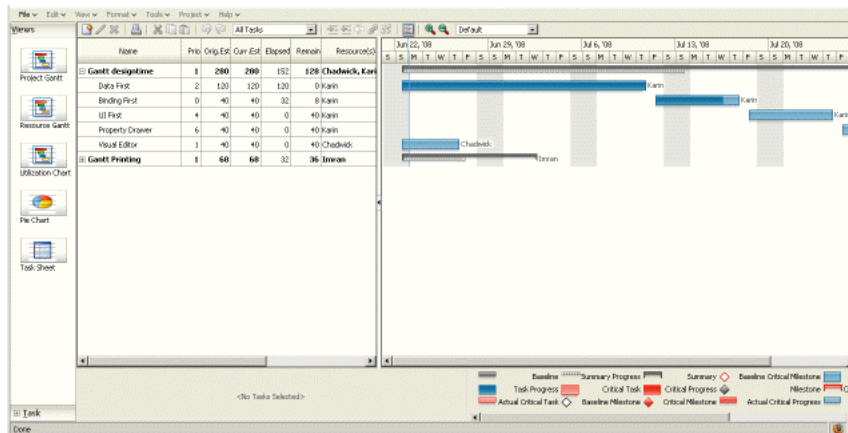
Figure 23–11 Project Gantt
