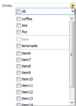
Figure 9–27 selectManyChoice Component
