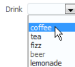
Figure 9–24 selectOneChoice Component
