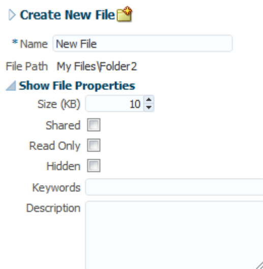
Figure 8–27 Expanded showDetail
