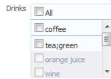
Figure 9–23 selectManyListbox Component
