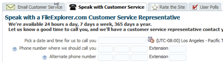
Figure 1–11 Help System
