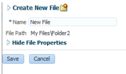
Figure 8–26 Collapsed showDetail
