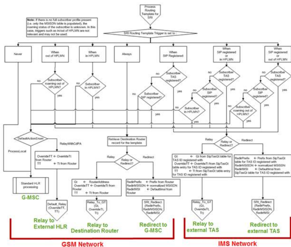
Figure 42: SRI message routing in the Tekelec ngHLR
