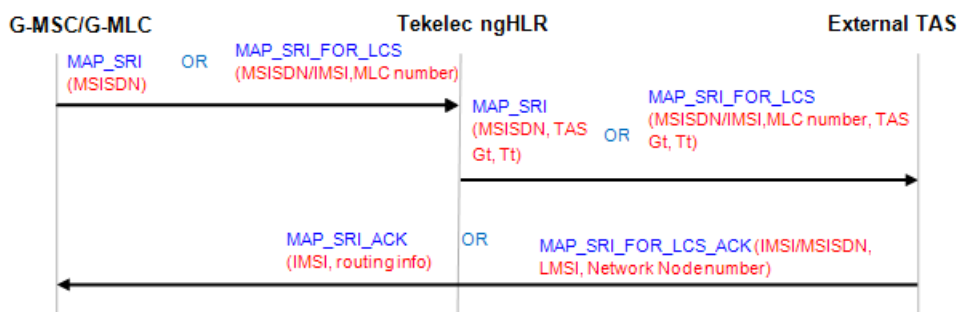
Figure 54: Call flow for SRI-LCS Redirect with external TAS (IMS Network)
