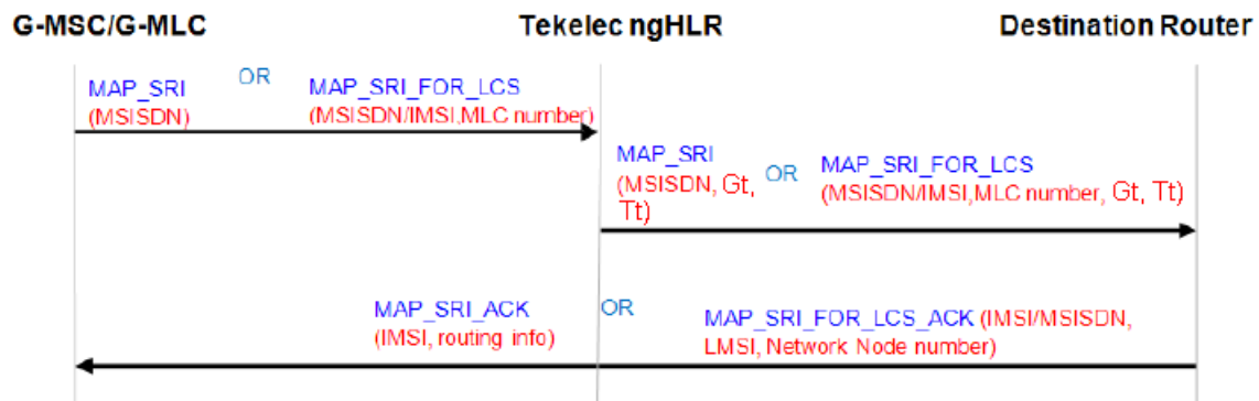
Figure 47: Call flow for SRI/SRI-LCS Relay to a Destination Router within the GSM Network
