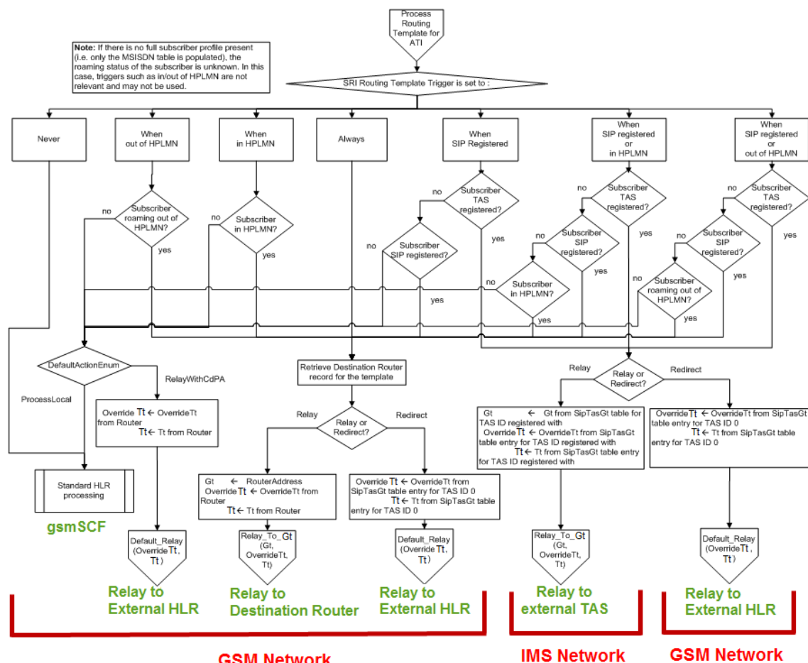
Figure 55: ATI message routing in the Tekelec ngHLR
