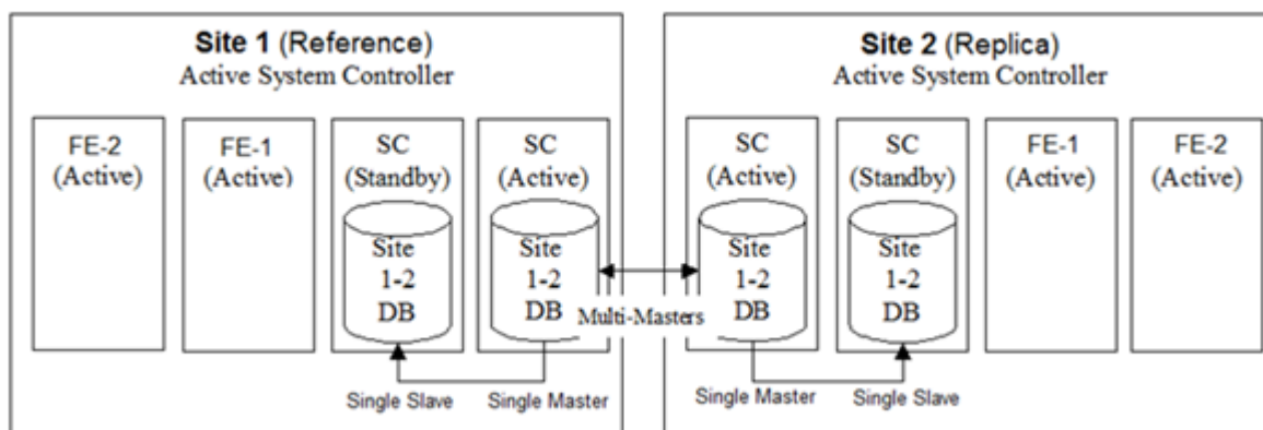
Figure 22: Data replication between two geo-redundant sites.
