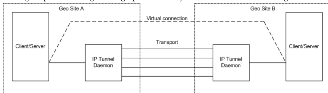
Figure 26: Multi-Homed IP Tunneling
