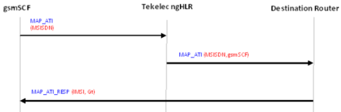
Figure 58: Call flow for ATI Relay to the Destination Router within the IMS Network
