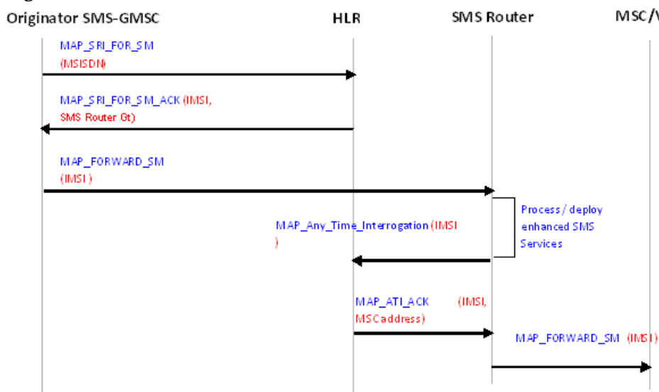
Figure 40: Call flow for MT-SMS Redirect to the MSC/VLR (in the GSM network)
