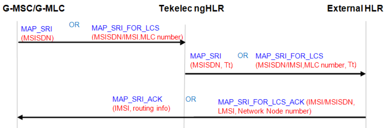
Figure 49: Call flow for SRI/SRI-LCS Default Relay with CdPA to an external HLR within the GSM Network
