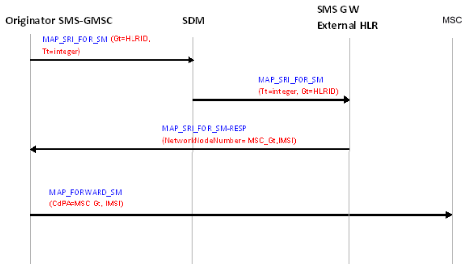
Figure 38: Call flow for MT-SMS Relay to the external HLR within the GSM Network
