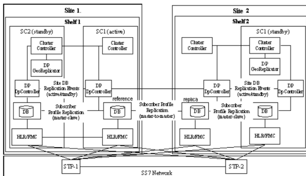
Figure 23: Data replication between two geo-redundant sites at the process level.
