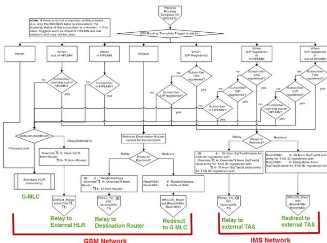
Figure 43: SRI-LCS message routing in the Tekelec ngHLR
