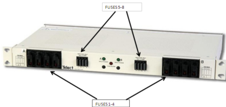
Figure 82: Telect 100A 4/4 fuse panel - front view
