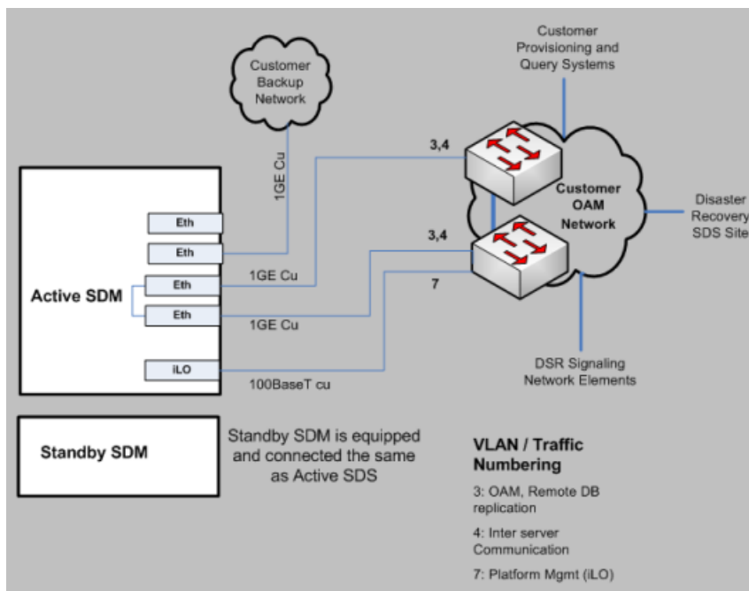
Figure 73: SDM rackmount configuration using dedicated uplink for NetBackup
