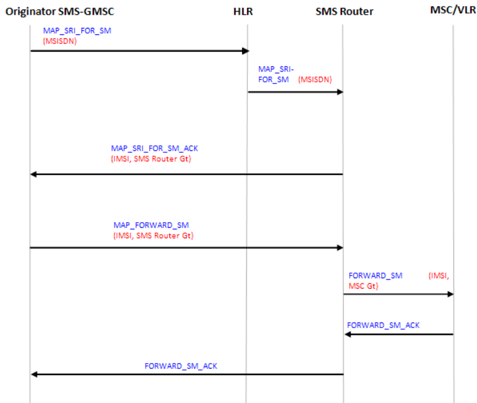
Figure 37: Call flow for MT-SMS Relay to the Destination Router within the GSM Network
