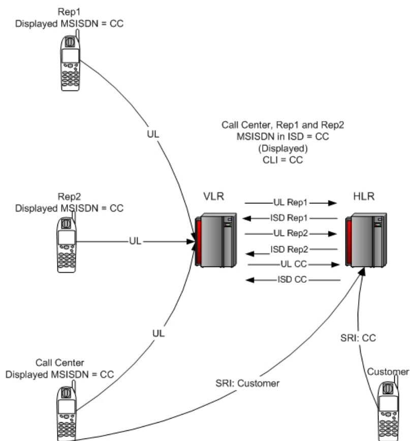
Figure 28: Example using Shared MSISDN across CLI
