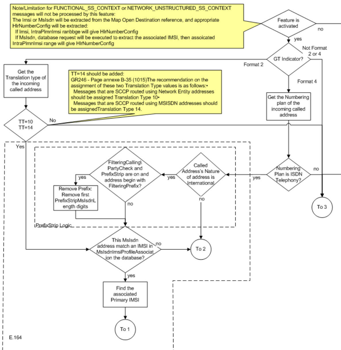
Figure 31: SCCP Routing for ITU and ANSI Calls
