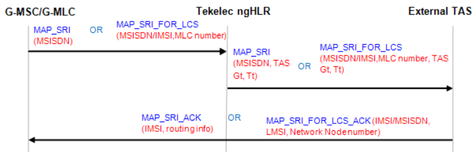
Figure 51: Call flow for SRI/SRI-LCS Relay to the external TAS within the IMS Network
