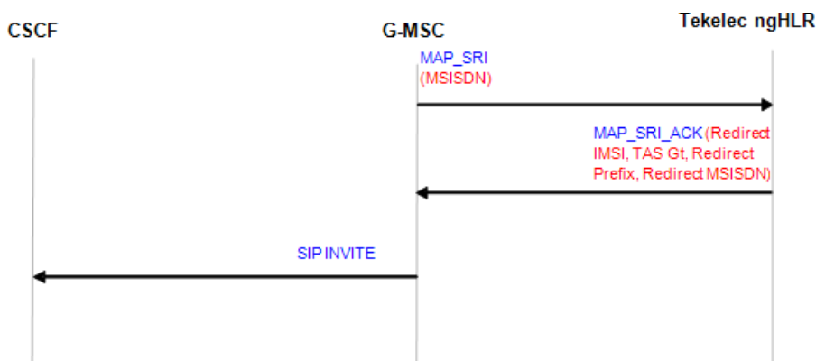
Figure 53: Call flow for SRI Redirect with external TAS (IMS Network)
