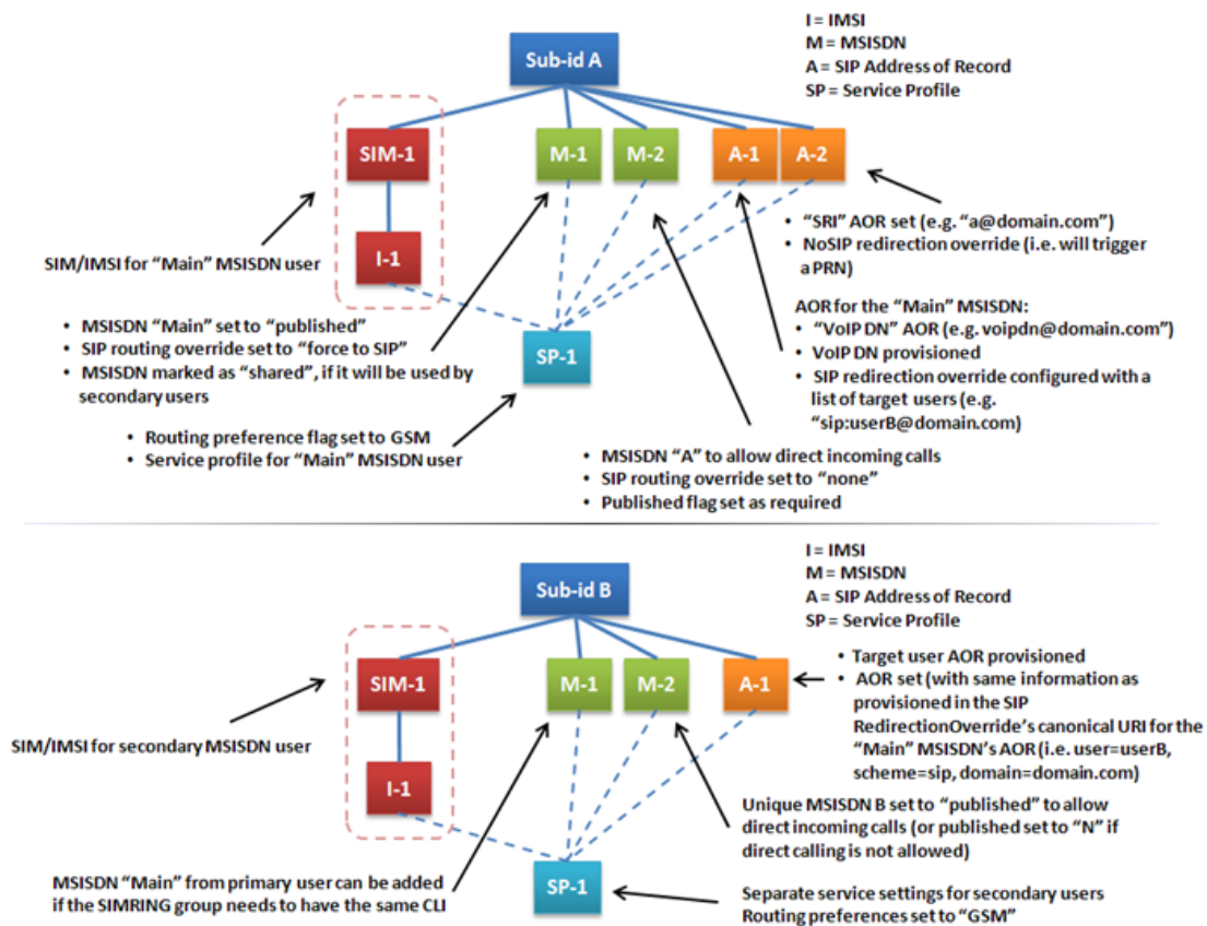
Figure 34: SimRing configuration
