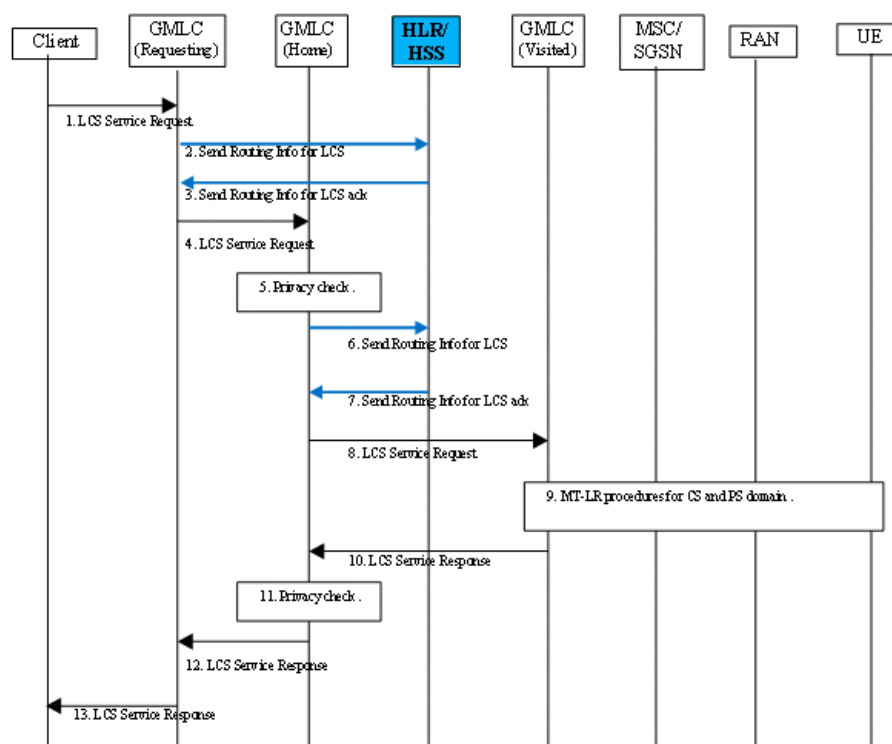
Figure 27: SRI-LCS Call Flow
