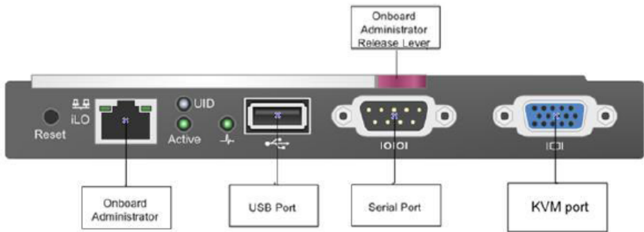
Figure 96: HP c7000 enclosure onboard administrator
