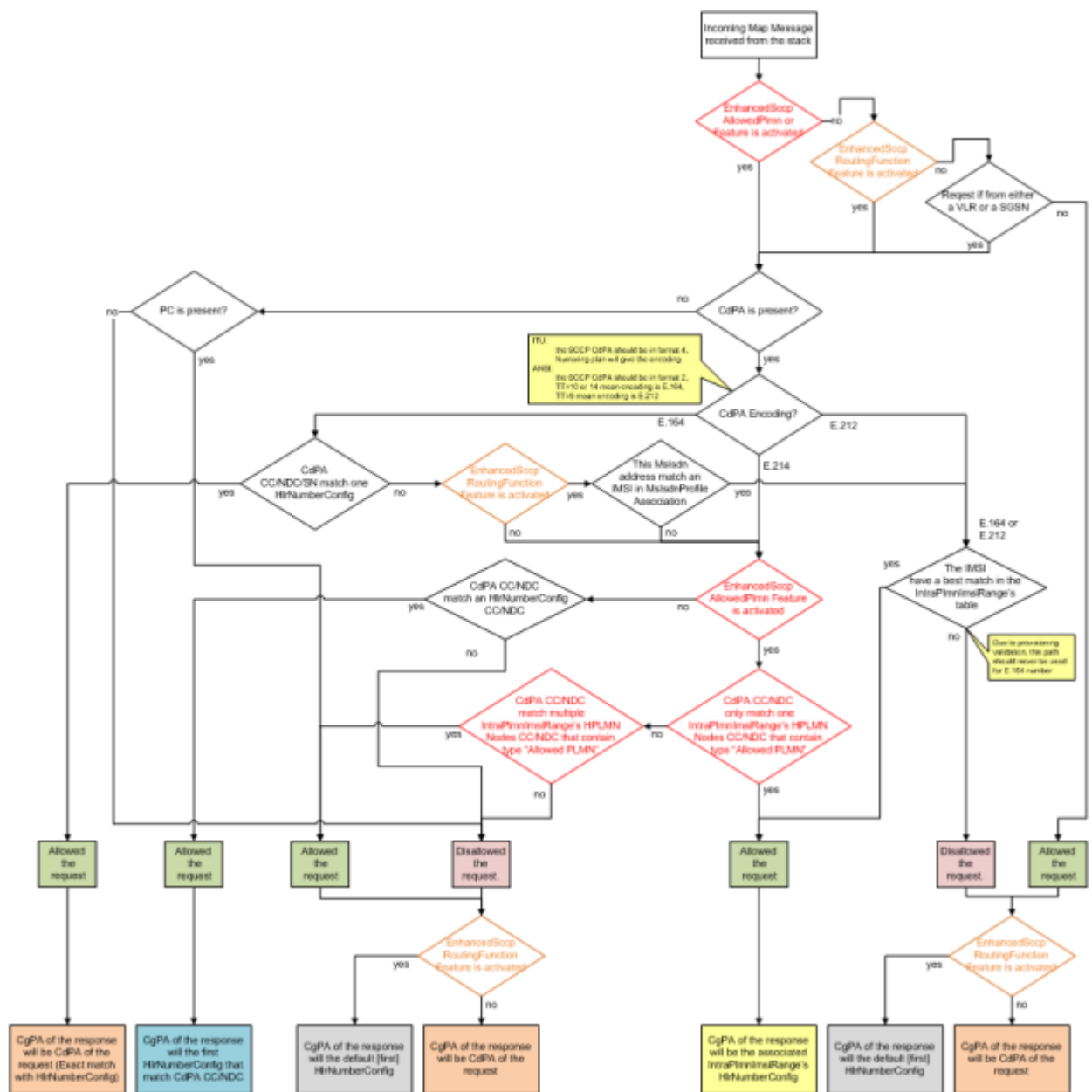
Figure 32: Enhanced SCCP Allowed PLMN flow
