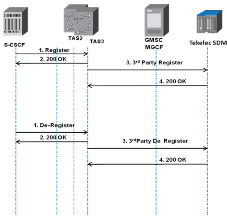
Figure 35: Register/De-Register Call Flow in the IMS Domain for 3rd Party Registration from TAS Node
