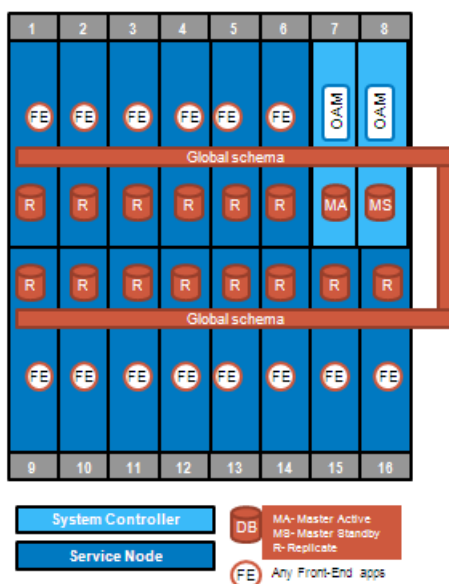
Figure 79: Example of HP c-Class architecture
