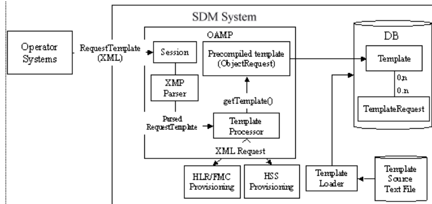
Figure 76: CommandTemplateLoader component diagram
