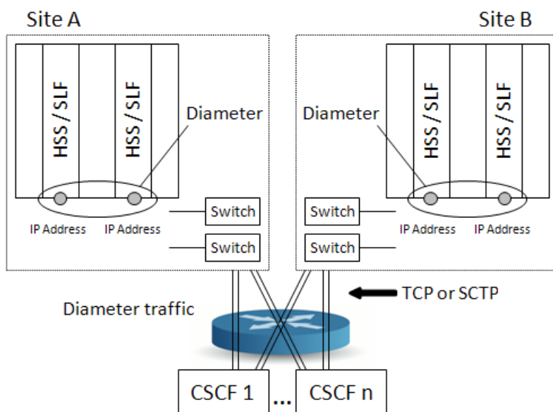
Figure 24: IMS-HSS network connections in a geo-redundant deployment.
