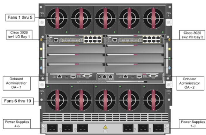
Figure 90: HP c7000 Enclosure Rear View
