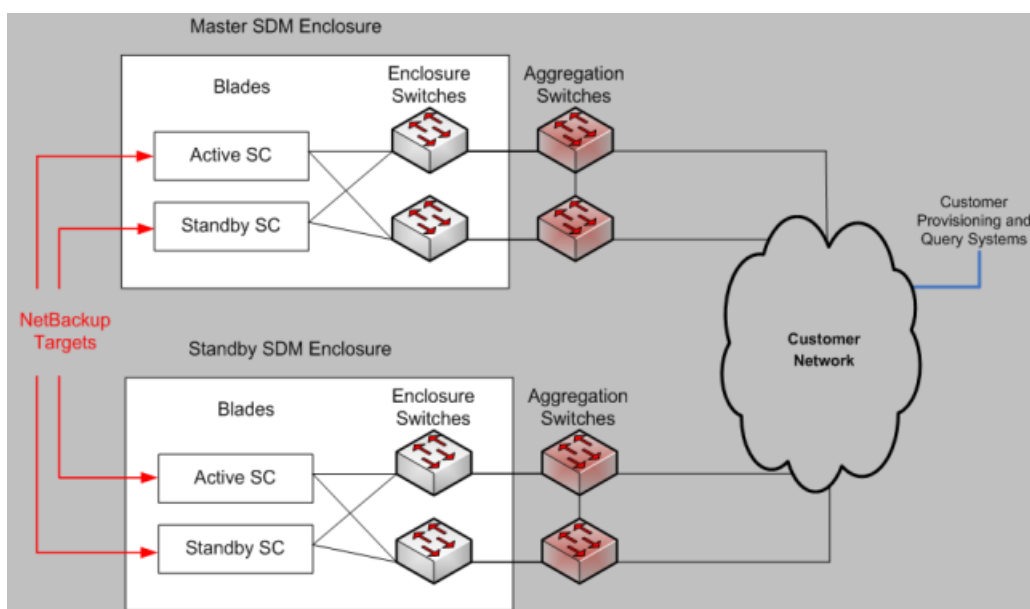
Figure 72: SDM C-Class configuration using XMI for NetBackup
