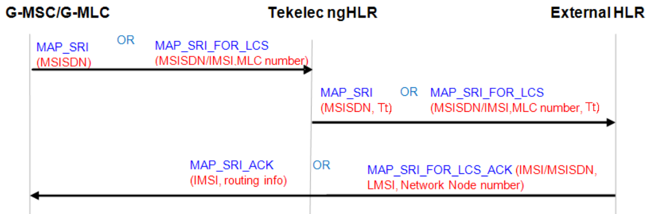
Figure 46: Call flow for SRI/SRI-LCS Default Relay with CdPA to an external HLR within the GSM Network
