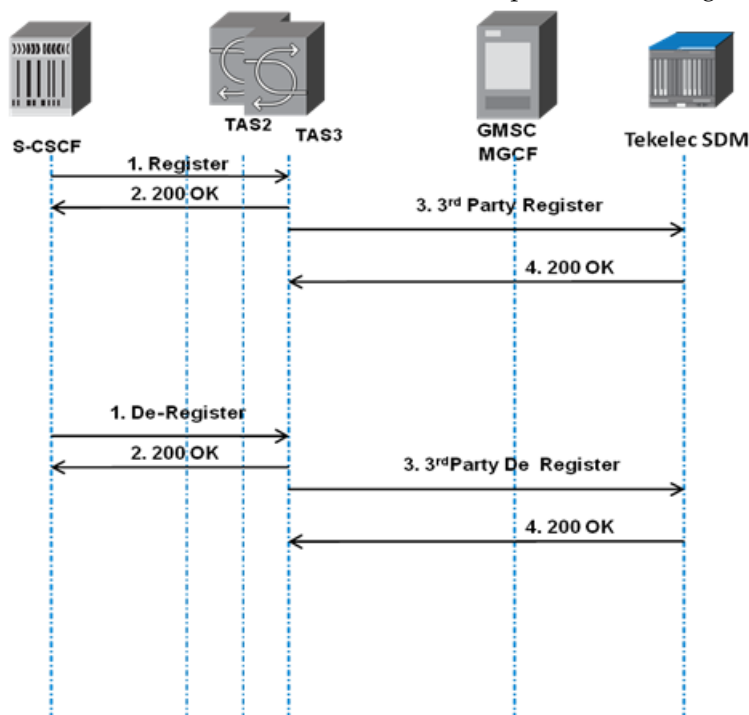
Figure 60: Register/De-register call flow in the IMS Domain for 3rd party registration from TAS node.
