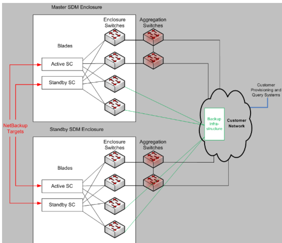
Figure 74: SDM C-Class configuration using dedicated uplink for NetBackup
