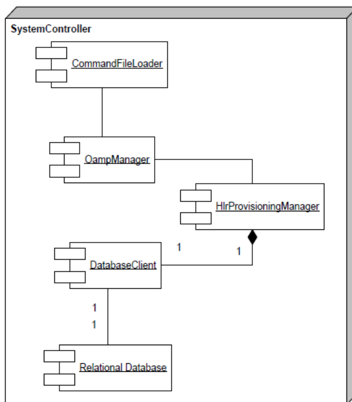
Figure 75: CommandFileLoader component diagram
