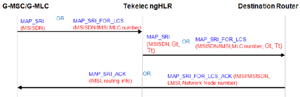
Figure 50: Call flow for SRI/SRI-LCS Relay to a Destination Router within the GSM Network
