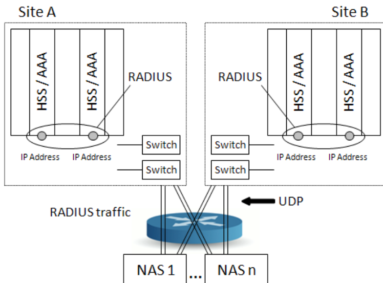
Figure 25: AAA network connections in a geo-redundant deployment.
