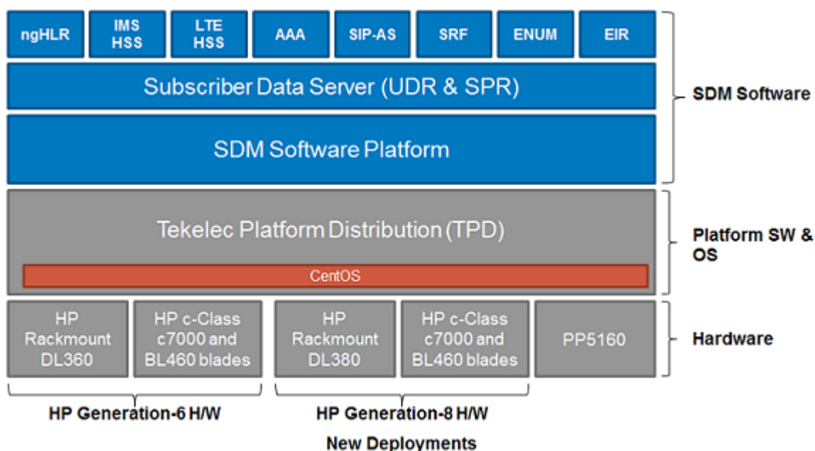
Figure 78: Subscriber Data Management (SDM) architecture
