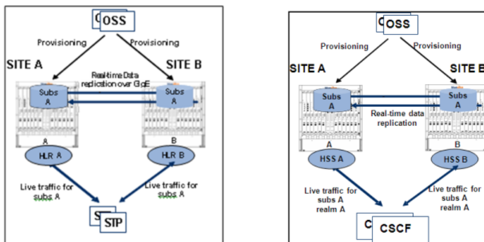
Figure 21: Geo Redundancy logic for the HLR and HSS services.
