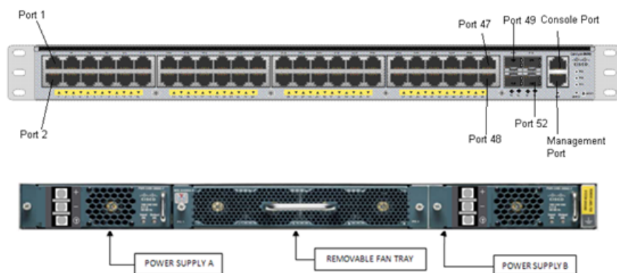
Figure 85: Cisco 4948E-F Aggregation Switch - front and rear views
