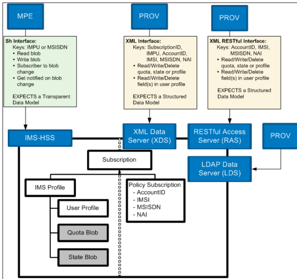
Figure 68: SPR Data Model
