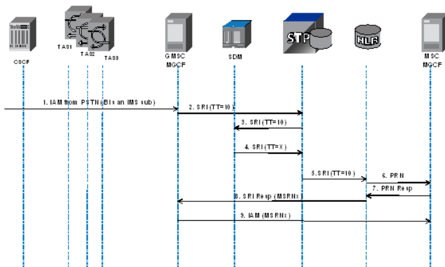
Figure 61: SRI message routing call flow in the IMS Domain for a 3rd party SIP registered subscriber.
