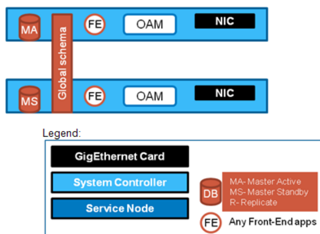
Figure 80: Example of rackmount architecture
