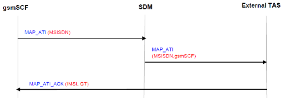
Figure 59: Call flow for ATI Relay to the external TAS within the IMS Network
