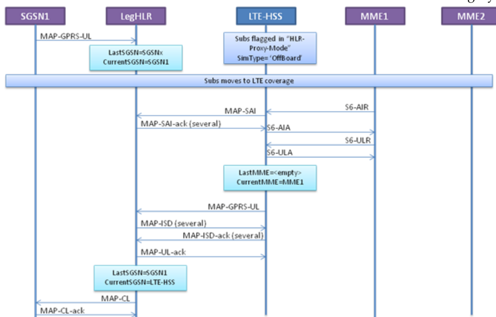
Figure 64: 3G>LTE Mobility
