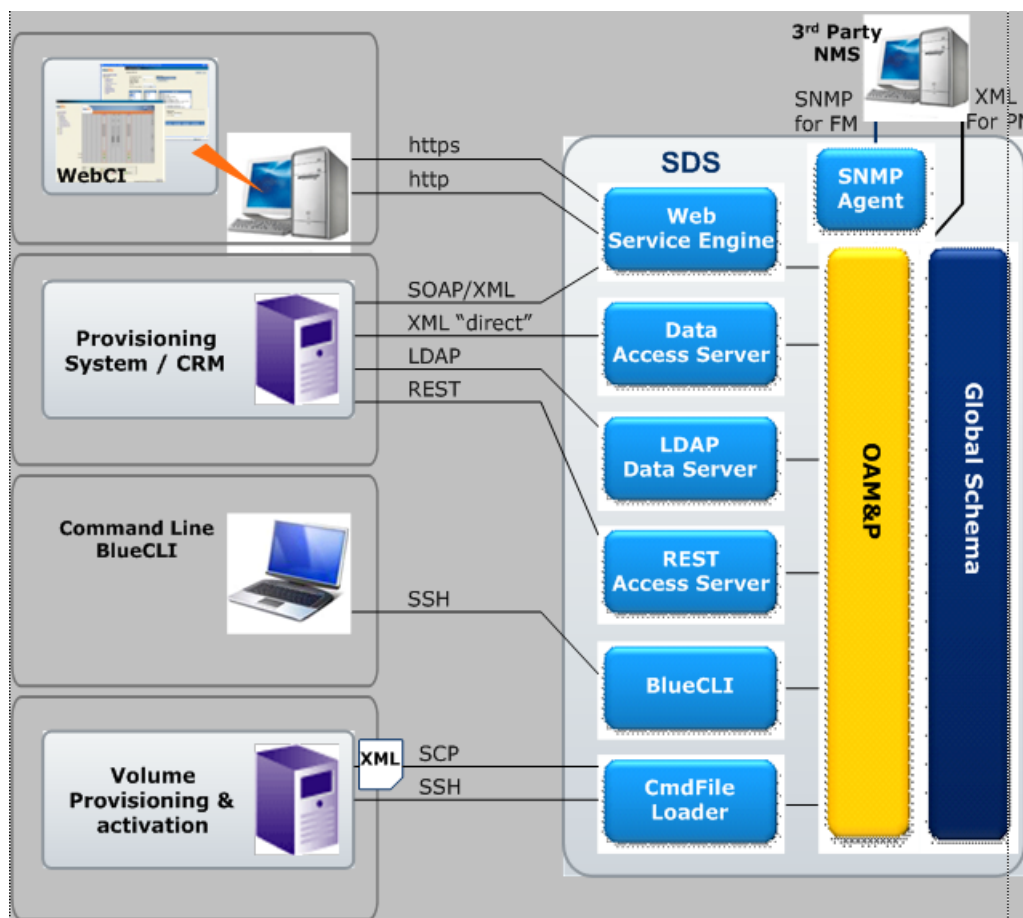
Figure 70: OAM&P interfaces
