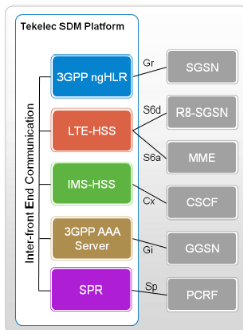
Figure 4: Inter-front-end communication
