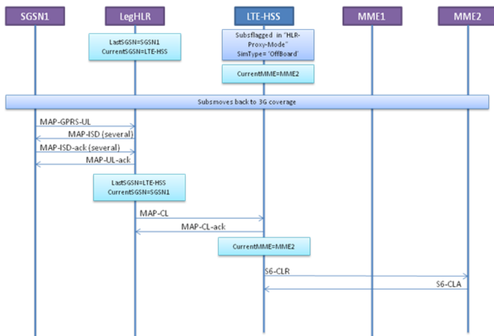
Figure 65: LTE&gt;3G Mobility
