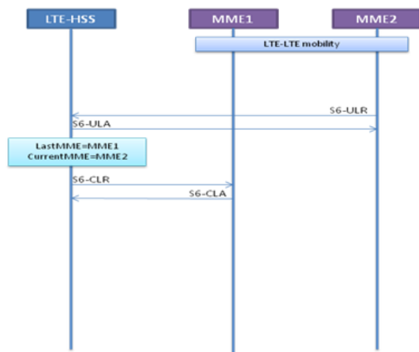
Figure 66: LTE&gt;LTE Mobility
