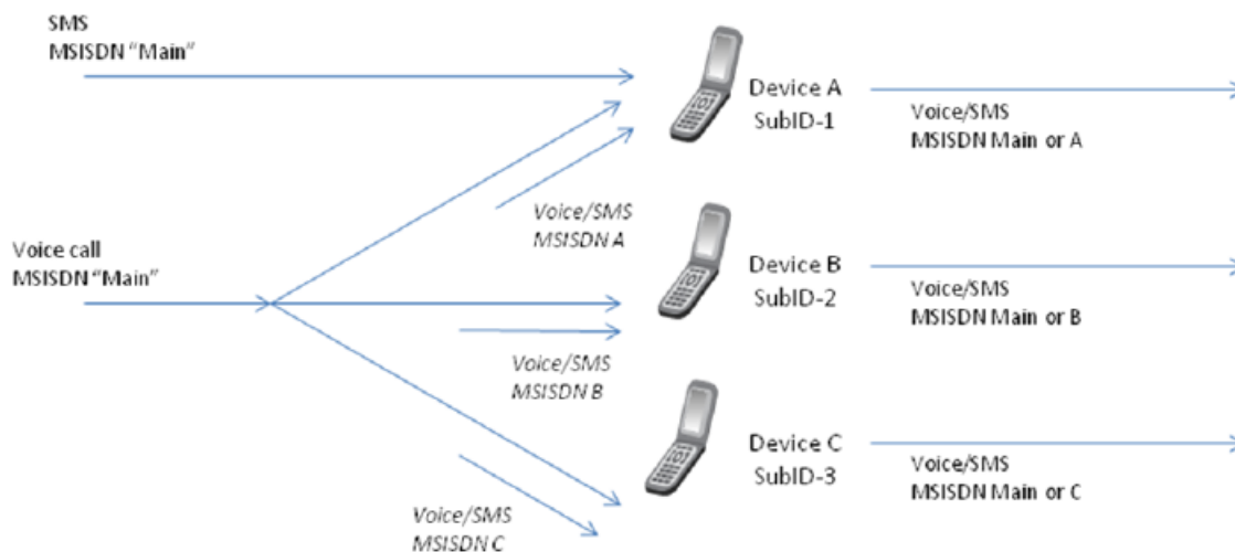
Figure 33: SIP-based SimRing
