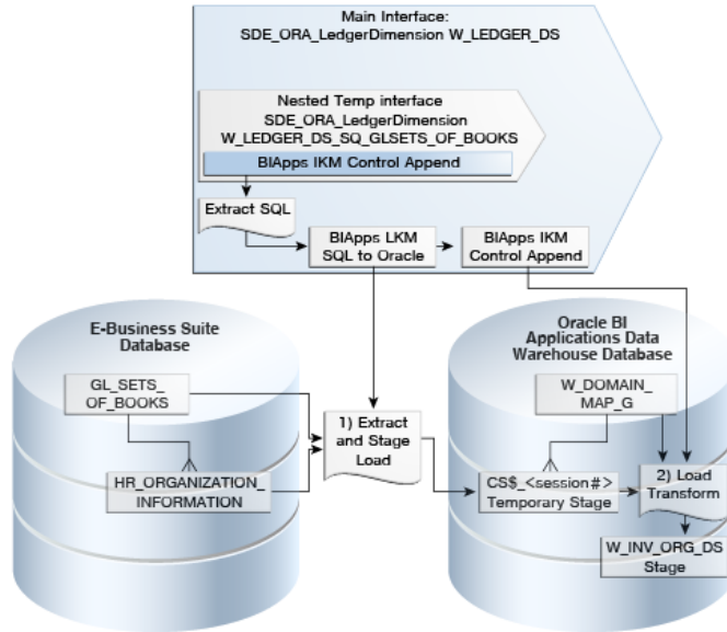
Figure 1-1 ETL Architecture
