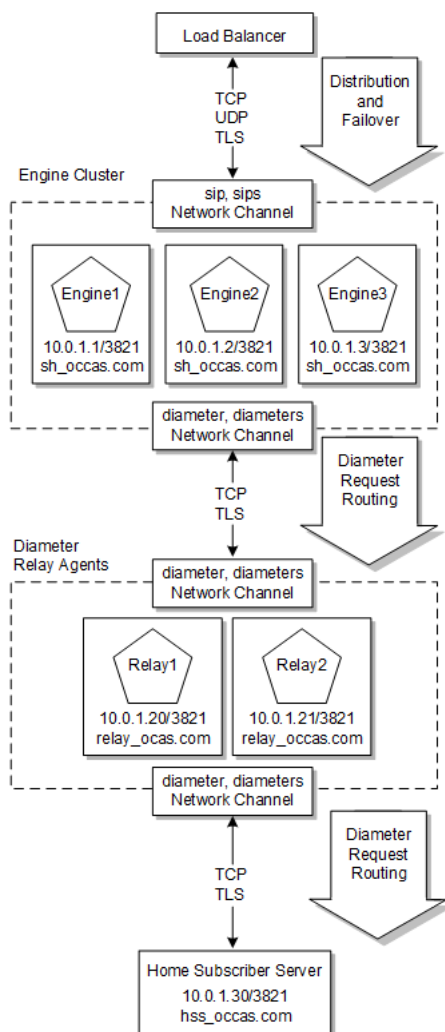
Figure 13–1 Sample Diameter Domain
