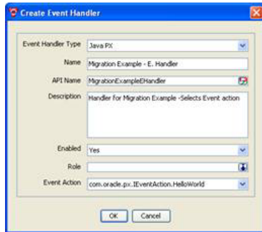
Figure A-7 The Create event Handler dialog
