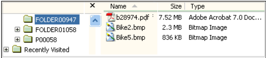
Figure 3–1 Select Folder
