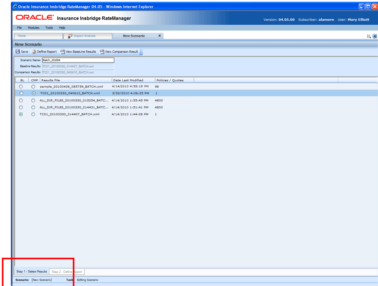
Figure 44 Step 1: Select Results
