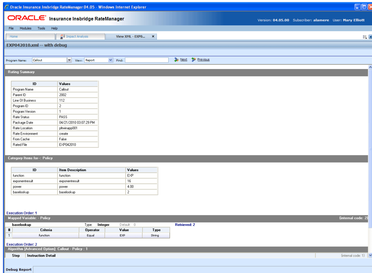
Figure 57 View Output Report
