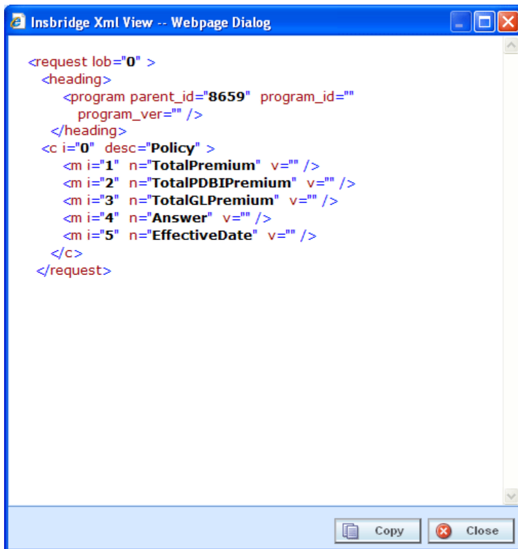
Figure 88 MultiLines Inputs XML
