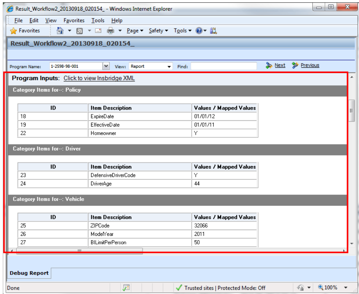
Figure 19 Rating Report with Debug
