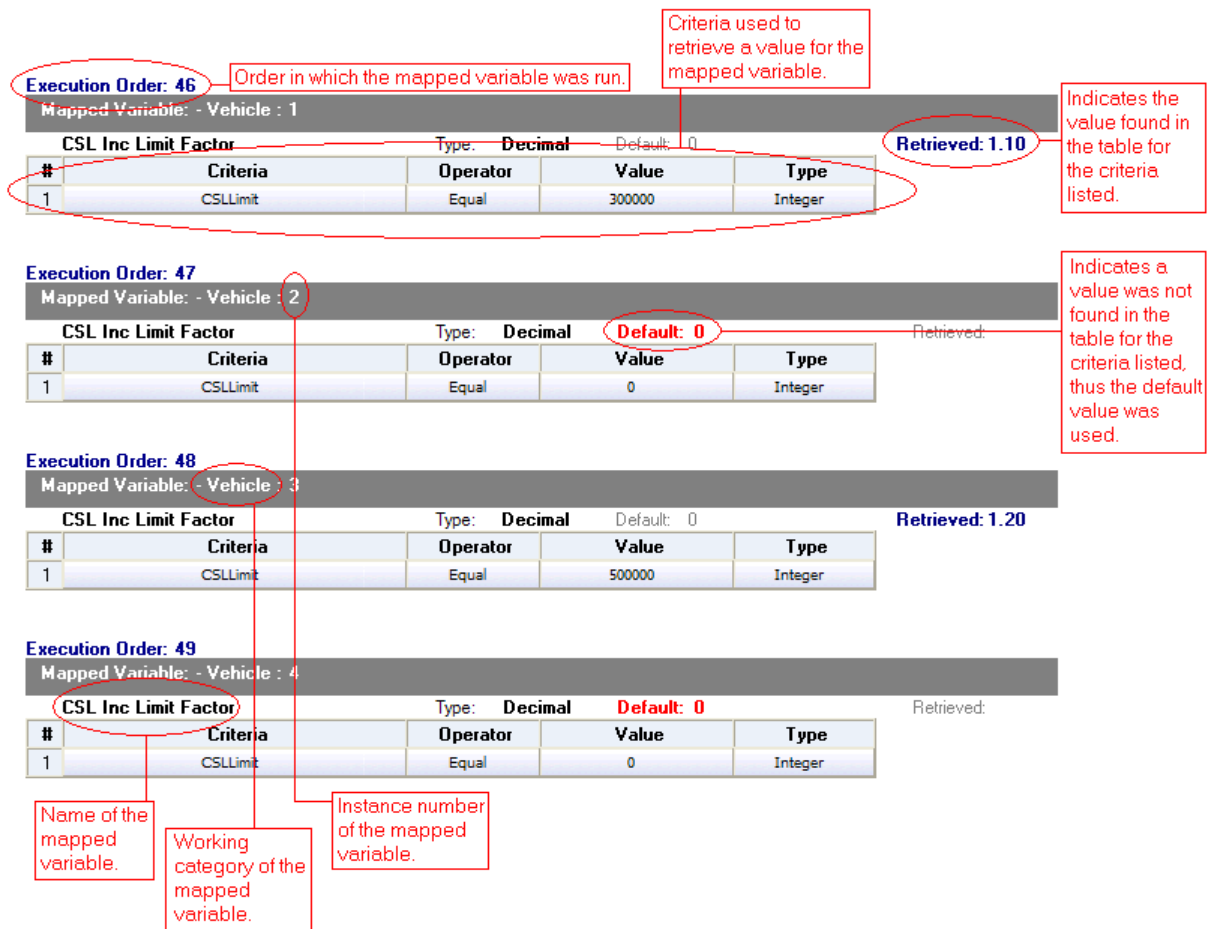
Figure 21 Debug Rating Report with Table Variable Highlighted
