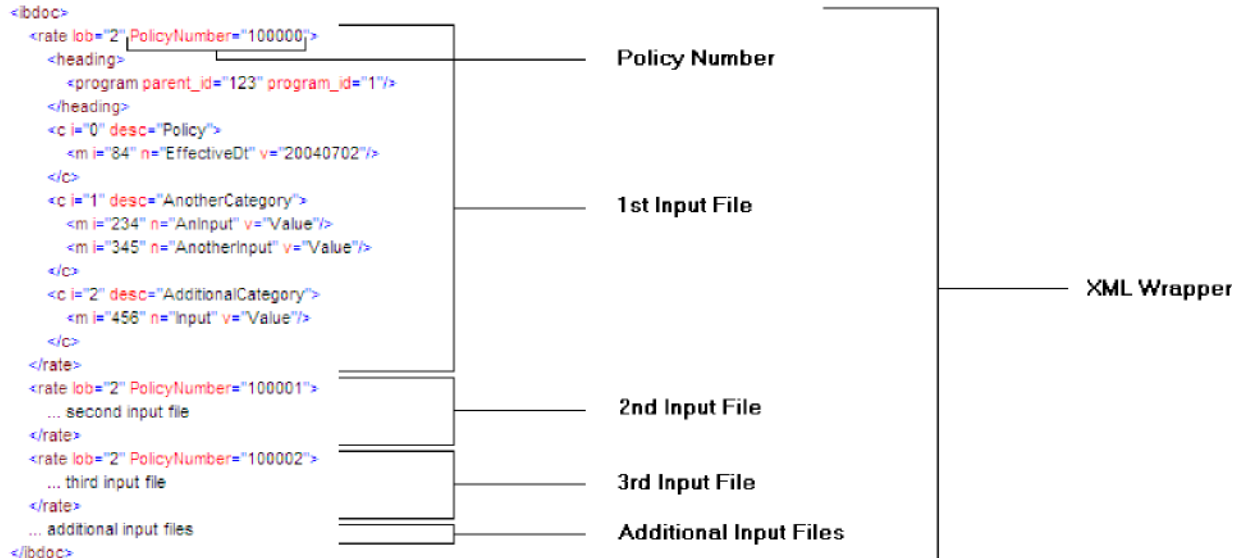
Figure 30 Example of a Batch XML File
