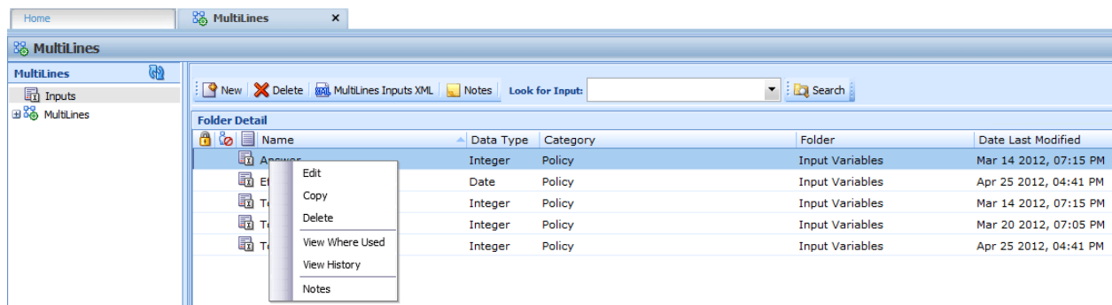
Figure 83 MultiLines Inputs Right Click Menu
