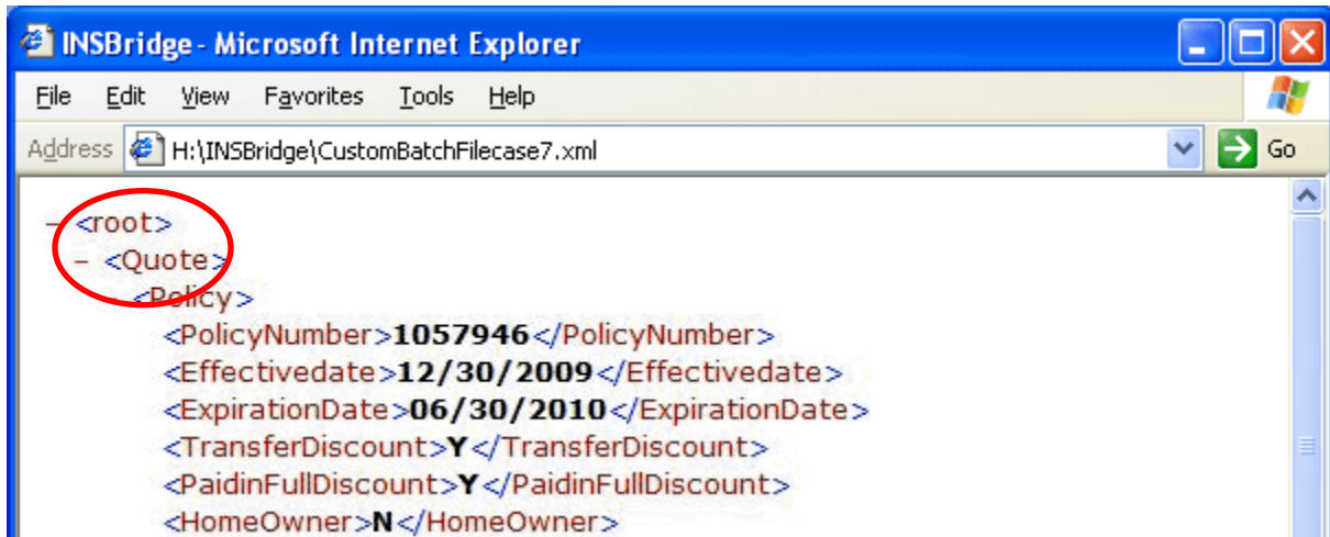
Figure 38 Example Custom Batch File
