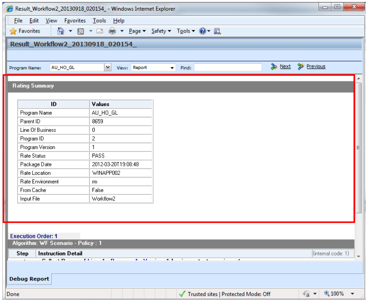
Figure 18 Rating Summary on a Debug Report
