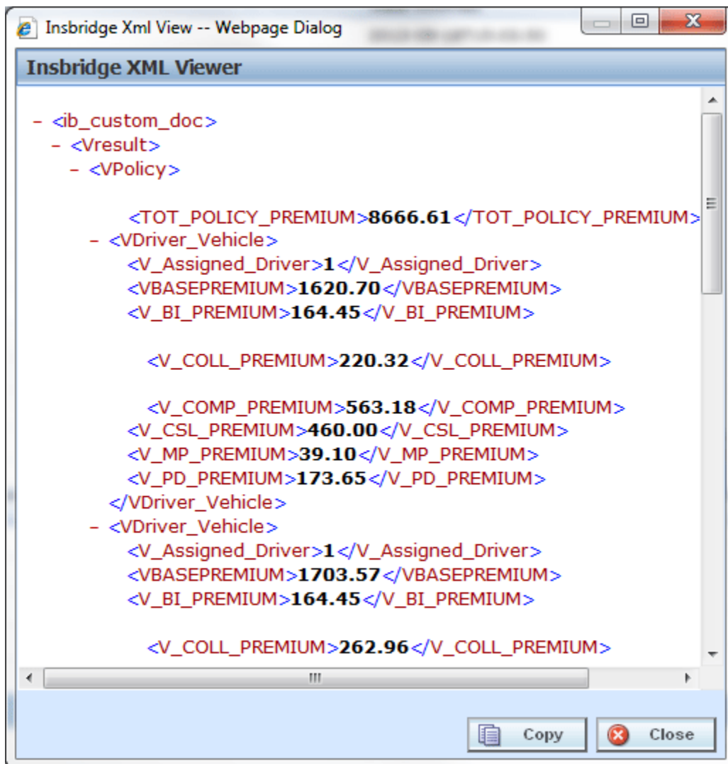
Figure 25 Using Custom Output Mapping
