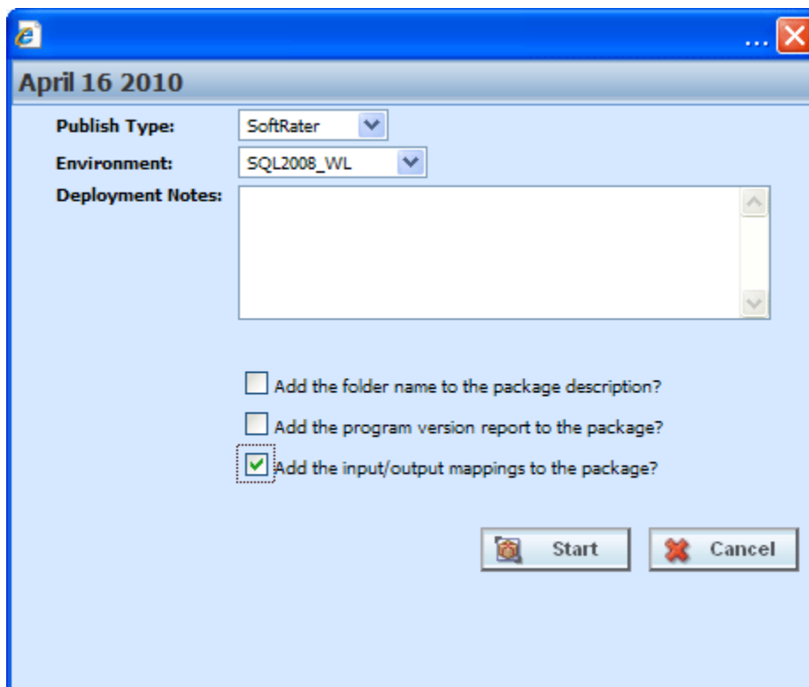
Figure 76 Editing Program Packaging Options Allowing for Override
