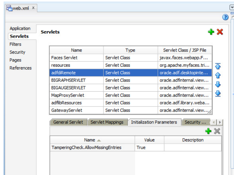
Figure 4–4 Enabling Missing Metadata Entries In JDeveloper
