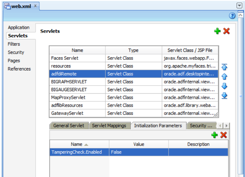
Figure 4-3 Disabling the Metadata Tamper Check In JDeveloper
