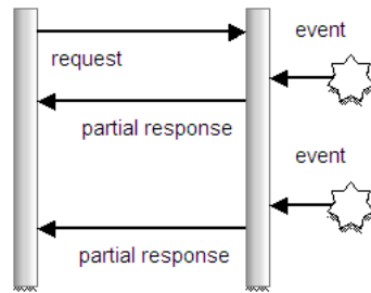
Figure 44–3 Streaming Mode
