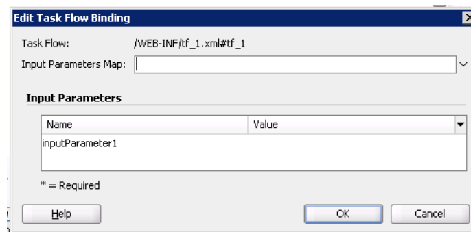
Figure 19–3 Edit Task Flow Binding Dialog for an ADF Region
