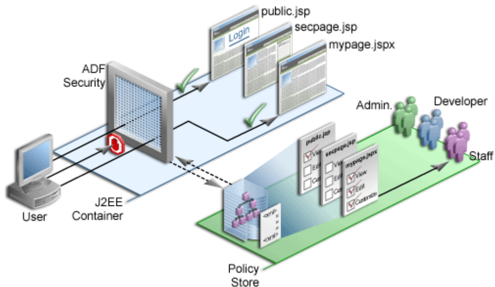
Figure 32–28 ADF Security Authorization
