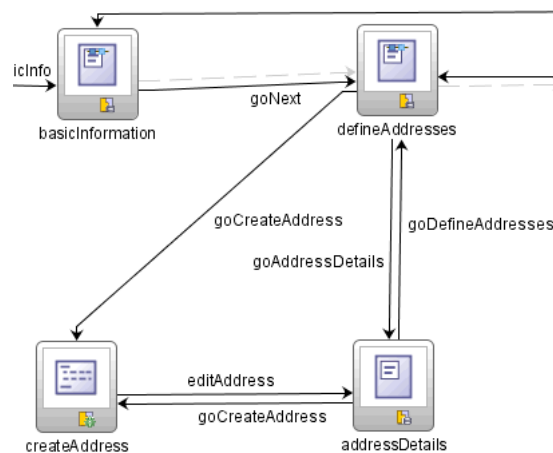
Figure 24–9 Task Flow for an Input Form
