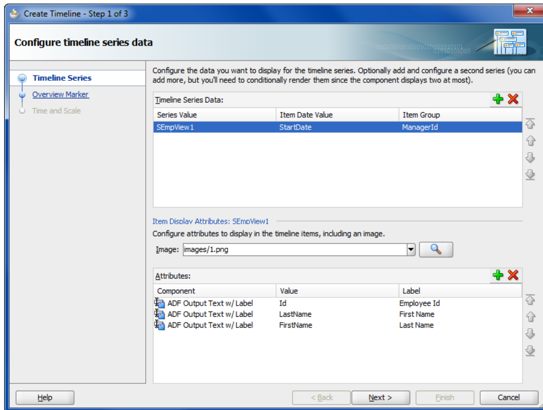
Figure 28–93 Configure Timeline Series Data Page of Create Timeline Wizard
