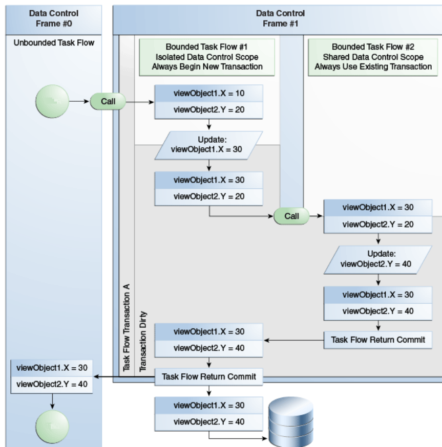
Figure 20–5 Guaranteed Joined Transactions
