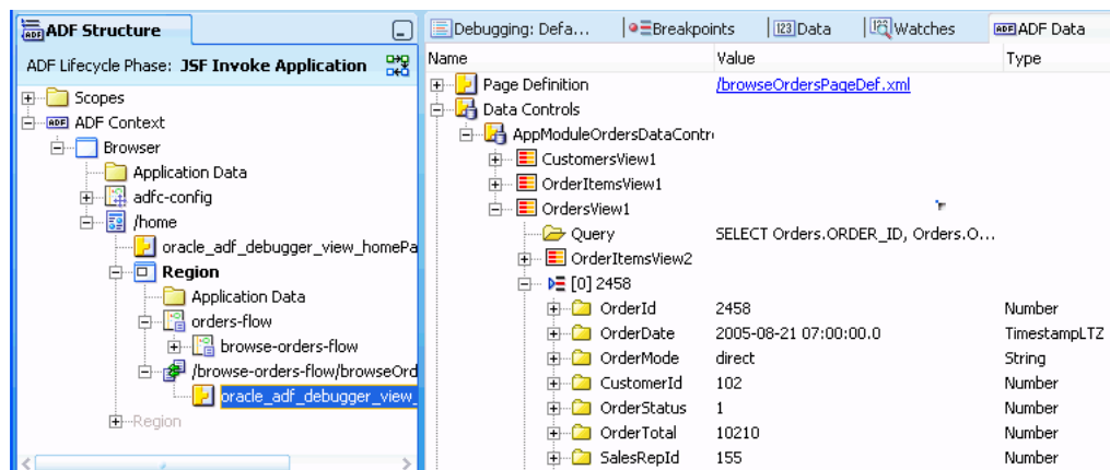
Figure 33–41 Binding Container (Business Components) Selected for the ADF Data Window
