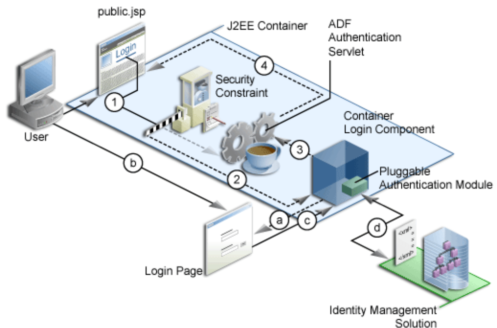
Figure 32–27 ADF Security Explicit Authentication
