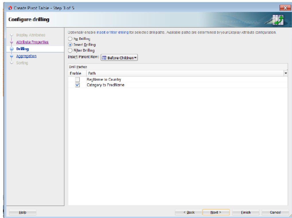
Figure 28–42 Configure Drilling Page of Create Pivot Table Wizard
