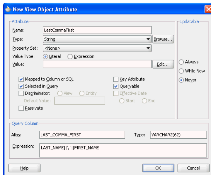
Figure 5-53 New SQL-Calculated Attribute
