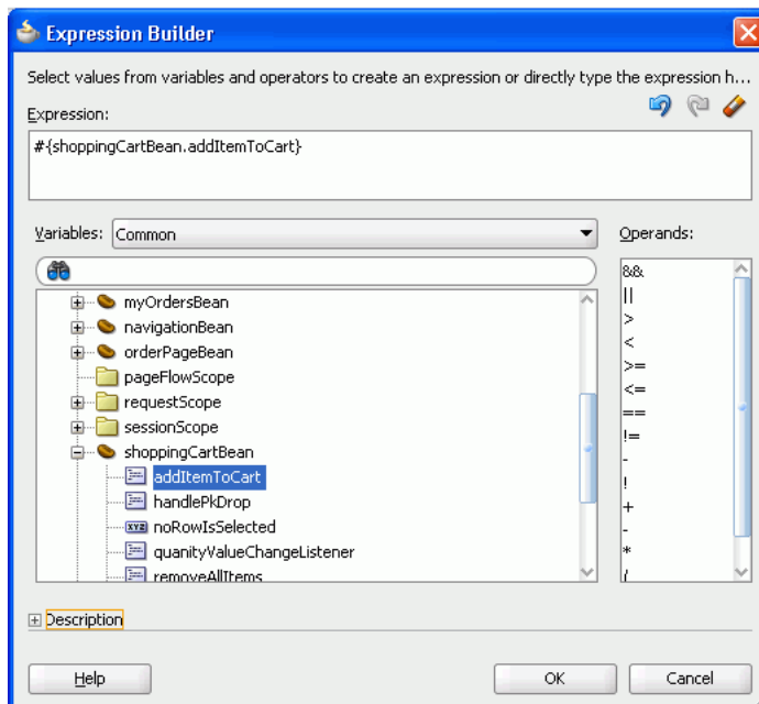
Figure 17-7 EL Expression for Method in Expression Builder Dialog
