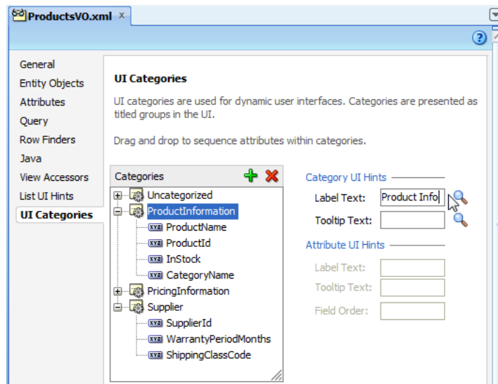
Figure 29–6 View Object Overview Editor UI Categories Page
