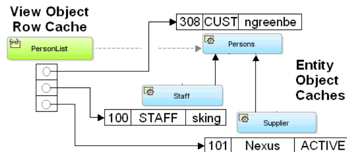
Figure 41–8 View Object with a Polymorphic Entity Usage Handles Entity Subtypes
