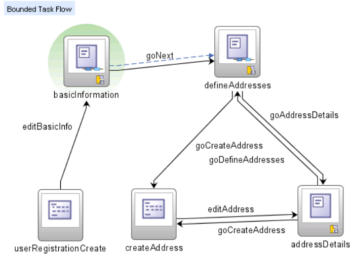
Figure 20–12 Detail of Customer Registration Task Flow
