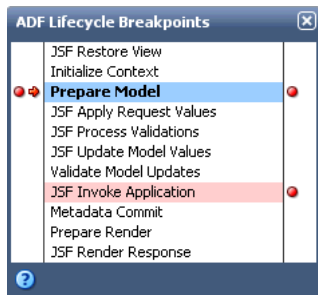
Figure 33–31 Execution Point Displayed in the ADF Lifecycle Breakpoints Window
