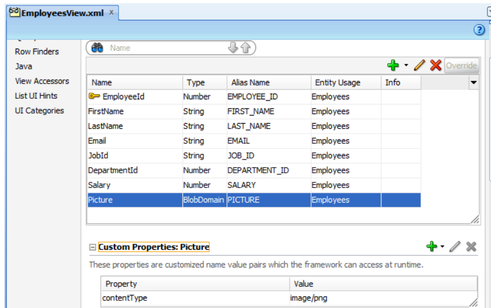
Figure 12-6 Custom Content Type Configured for LOB Attributes
