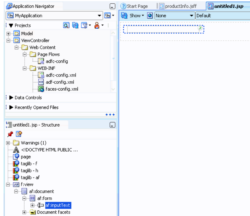
Figure 13-16 The Structure Window in JDeveloper
