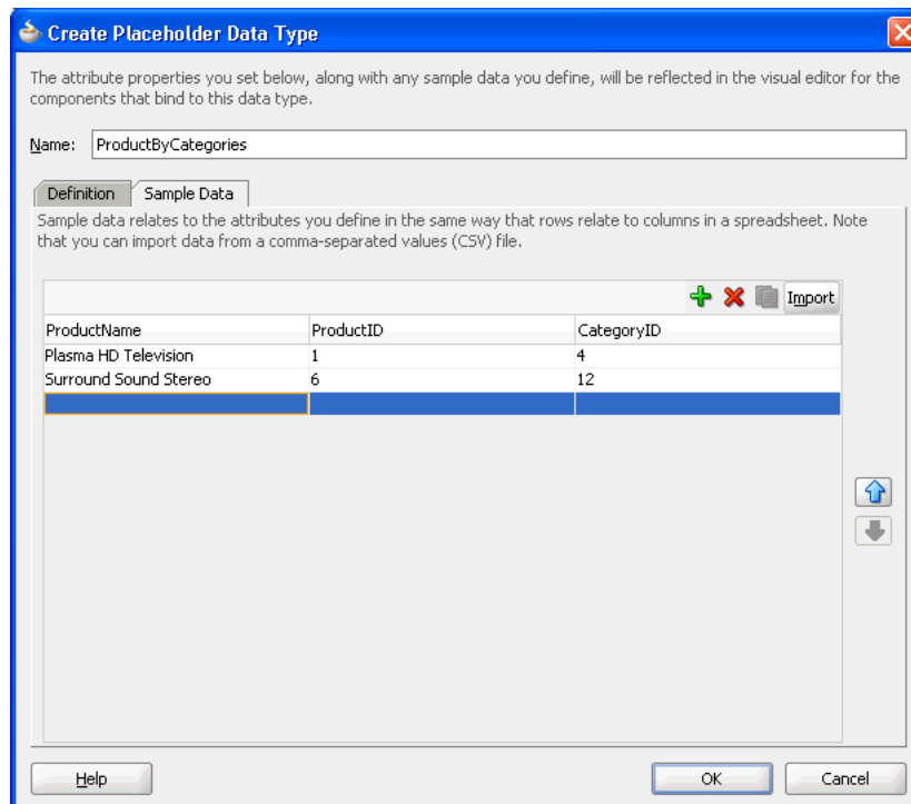
Figure 31–10 Adding Sample Data
