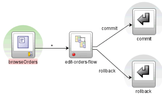
Figure 33–16 ADF Declarative Breakpoint on a Task Flow Activity
