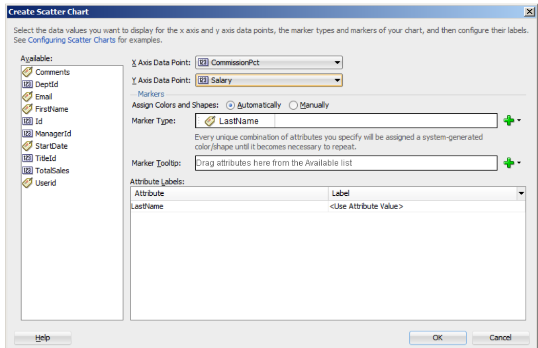
Figure 28–16 Create Scatter Chart Dialog
