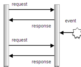
Figure 44–4 Poll Mode
