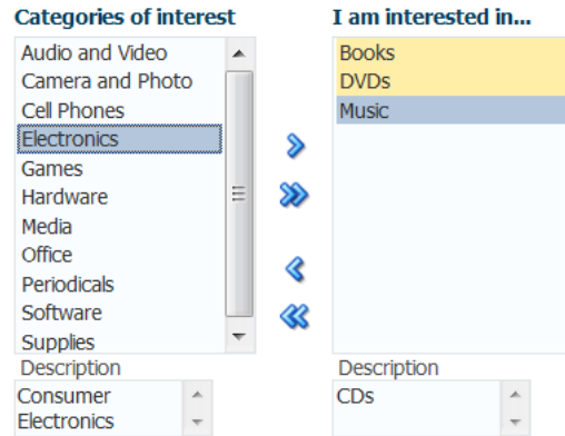
Figure 27-7 SelectManyShuttle Component
