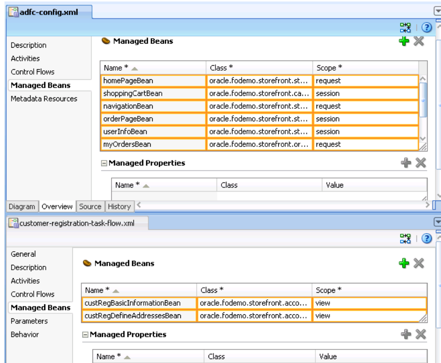
Figure 16–10 Managed Beans Registered with Task Flows
