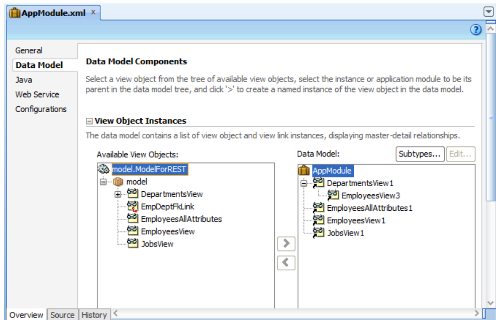
Figure 15–2 REST Sample Project - Application Module Data Model
