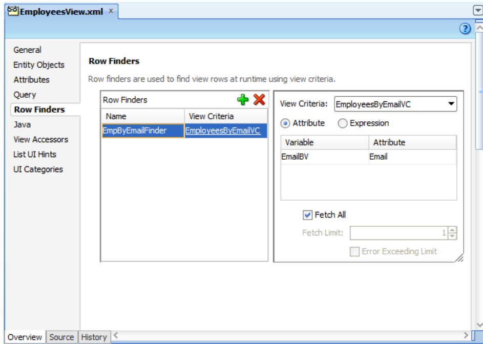
Figure 15–7 REST Sample Project - Employees Row Finder
