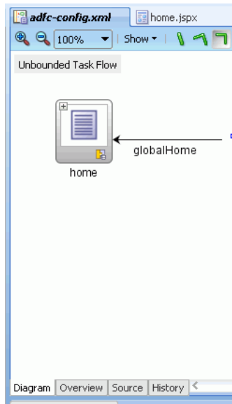
Figure 17–2 View Activity
