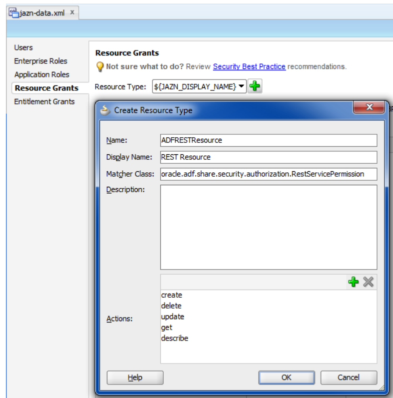
Figure 12–13 Creating an ADF REST Resource Type
