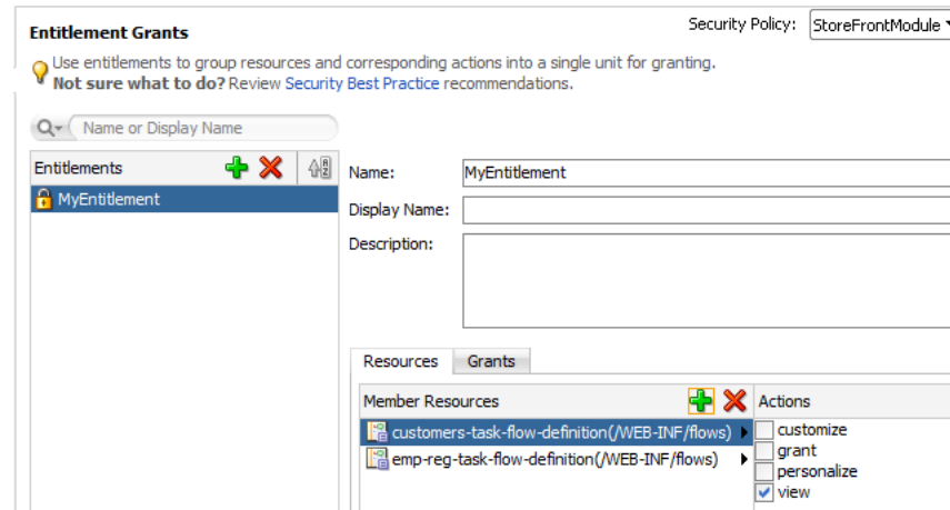
Figure 32–14 Adding a Bounded Task Flow as a Resource in an Entitlement Grant
