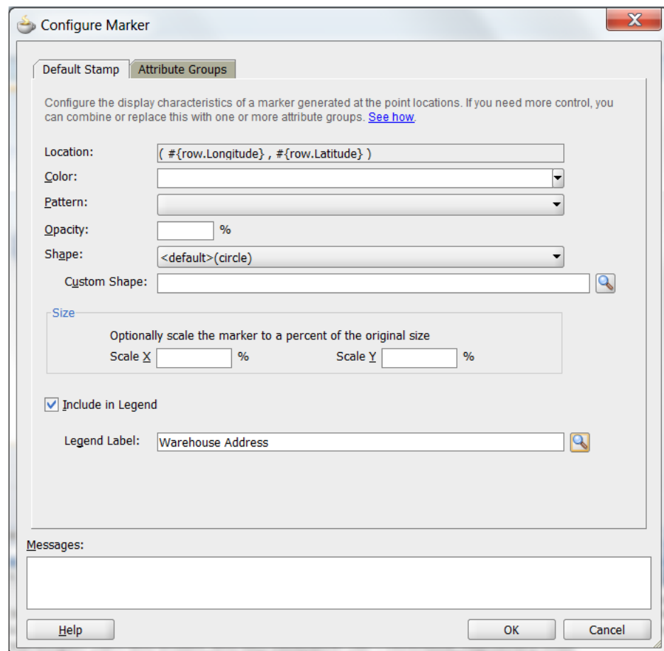
Figure 28–70 Configure Marker Dialog Default Stamp Page
