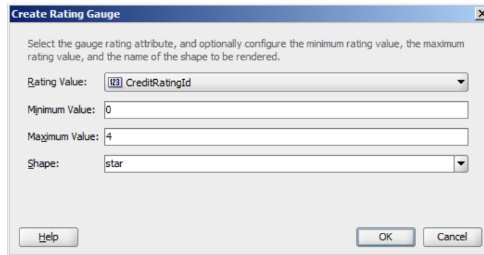
Figure 28–29 Create Rating Gauge Dialog for Credit Rating Gauge
