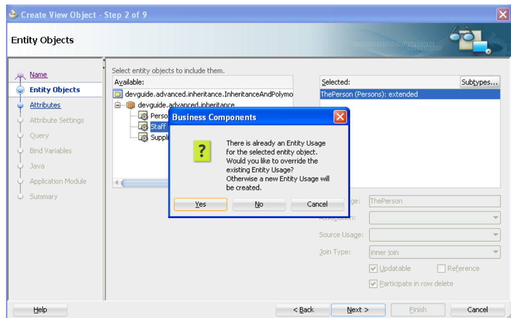
Figure 41-11 View Object with a Polymorphic Entity Subtype Selection
