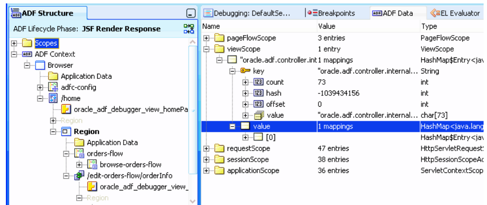
Figure 33–35 Scopes Node Selected in the ADF Structure Window
