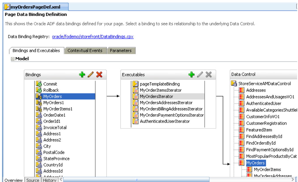
Figure 34–1 Page Data Binding Definition Overview Tab
