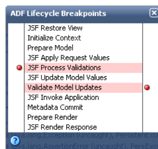
Figure 33–24 ADF Lifecycle Phase Breakpoints Enabled in the ADF Lifecycle Breakpoints Window
