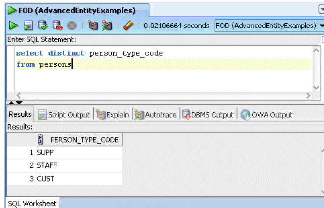
Figure 40–2 Using the SQL Worksheet to Find Distinct Discriminator Column Values
