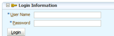
Figure 32–18 Login Page
