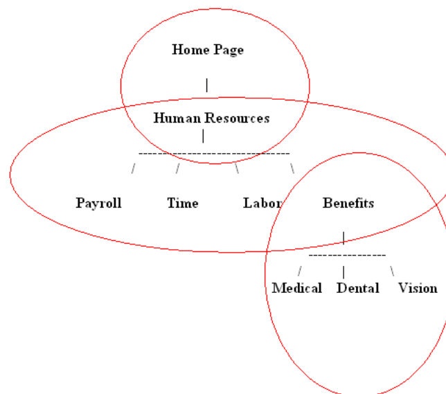
Figure 20–22 Menu Hierarchy
