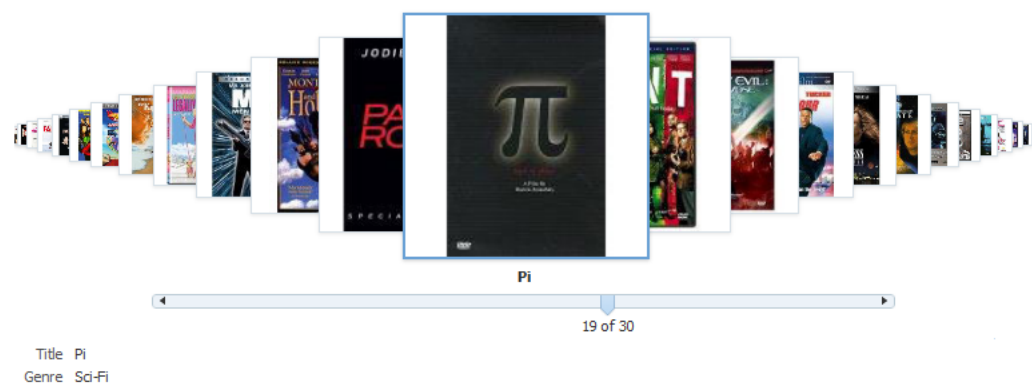
Figure 30–6 Carousel Component
