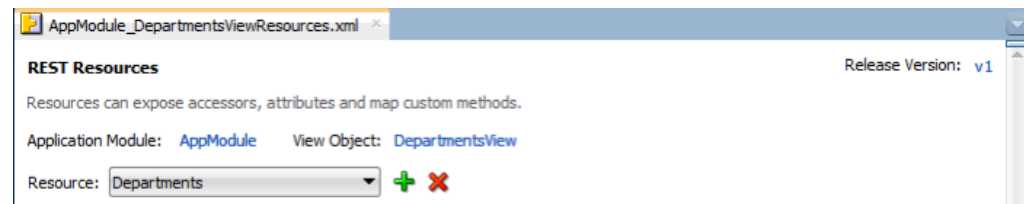
Figure 12–11 REST Resource Editor Displays Version
