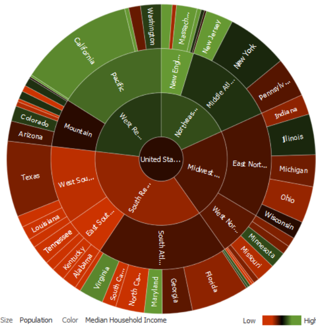
Figure 31–2 Sunburst Displaying United States Population and Median Income by Regions
