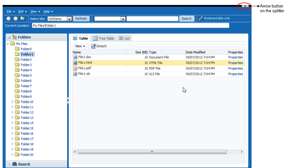
Figure 8–9 File Explorer Uses panelSplitter with a Vertical Split
