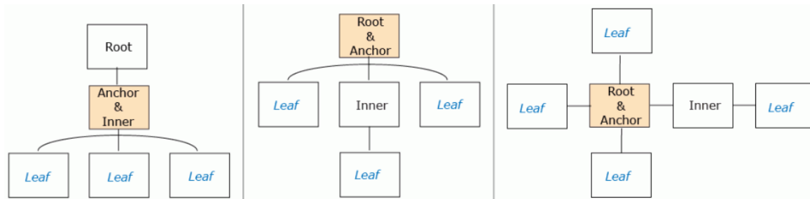
Figure 30–8 Node Types and Positions
