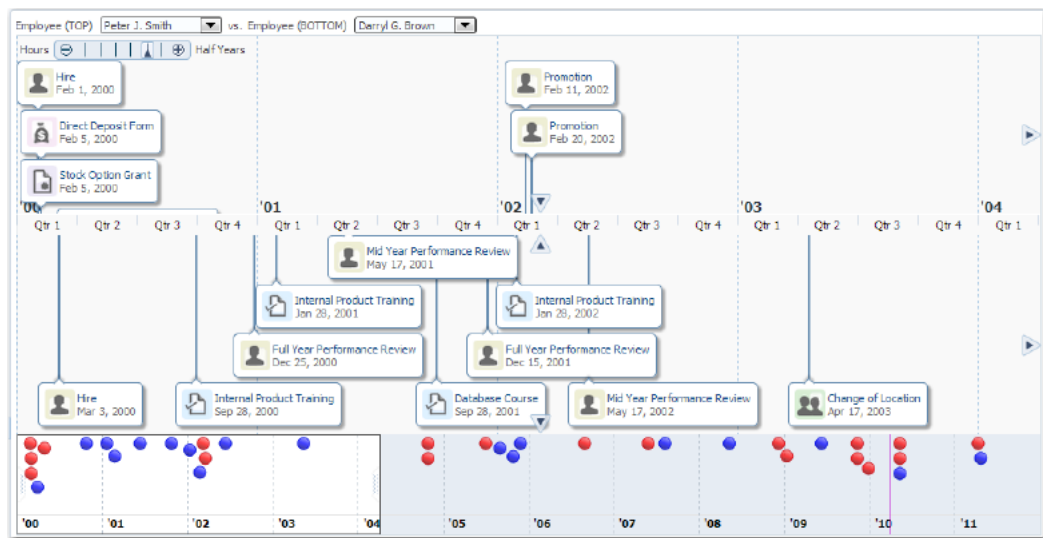
Figure 28–2 Dual Timeline Comparing Employee Change Events
