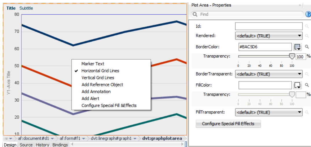
Figure G–23 Line Graph Plot Area Context Menu
