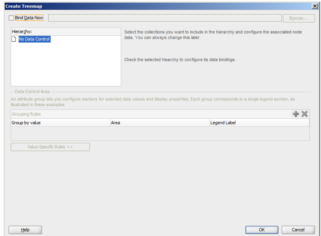
Figure 31–27 Create Treemap Dialog Using UI-First Development
