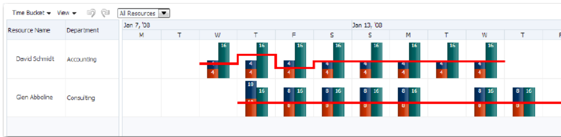
Figure 27–9 Resource Utilization Gantt Chart Resource Capacity Line
