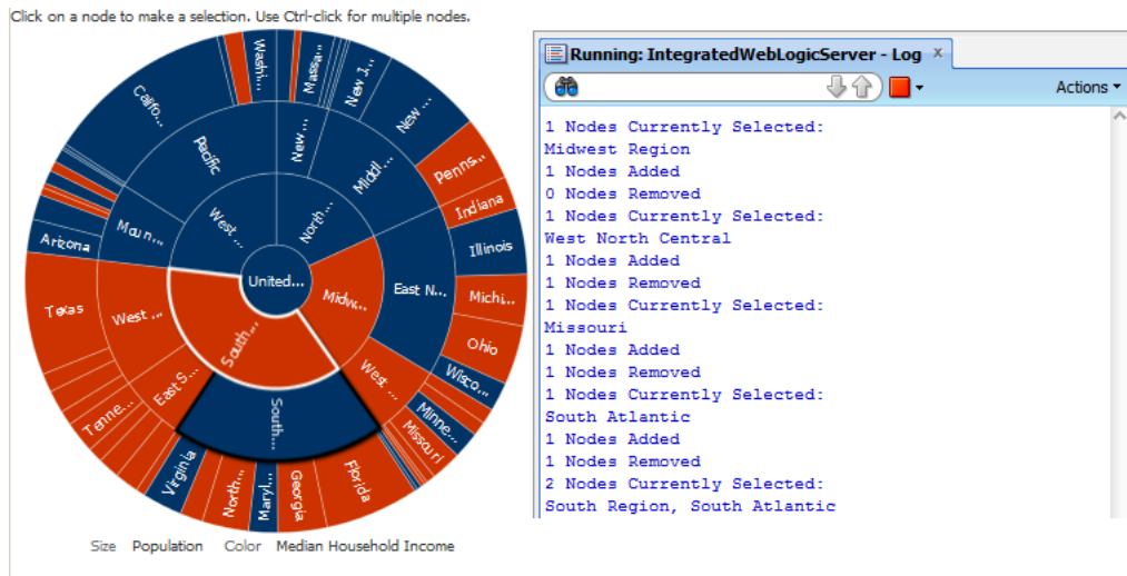
Figure 31–36 Sunburst Illustrating Custom Selection Listener
