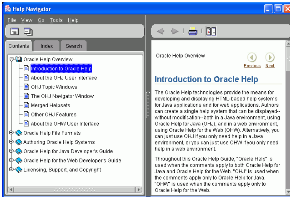
Figure 2-2 Docked Windows
