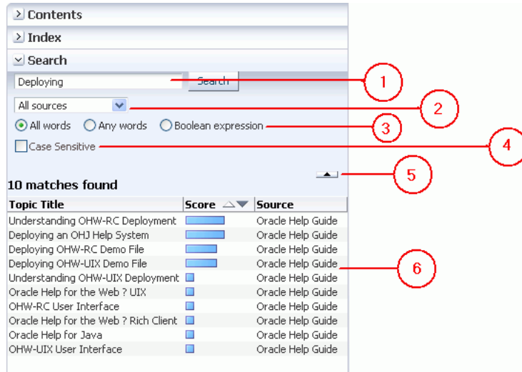
Figure 3–5 OHW-RC Search Navigator
