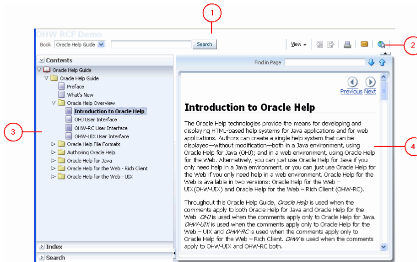
Figure 3–1 numbered callouts identify the following user interface components:
