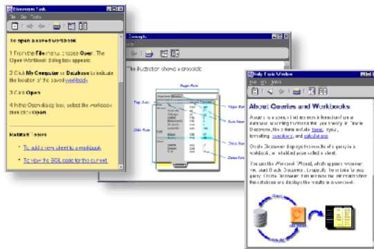
Figure 2-3 Topic Windows
