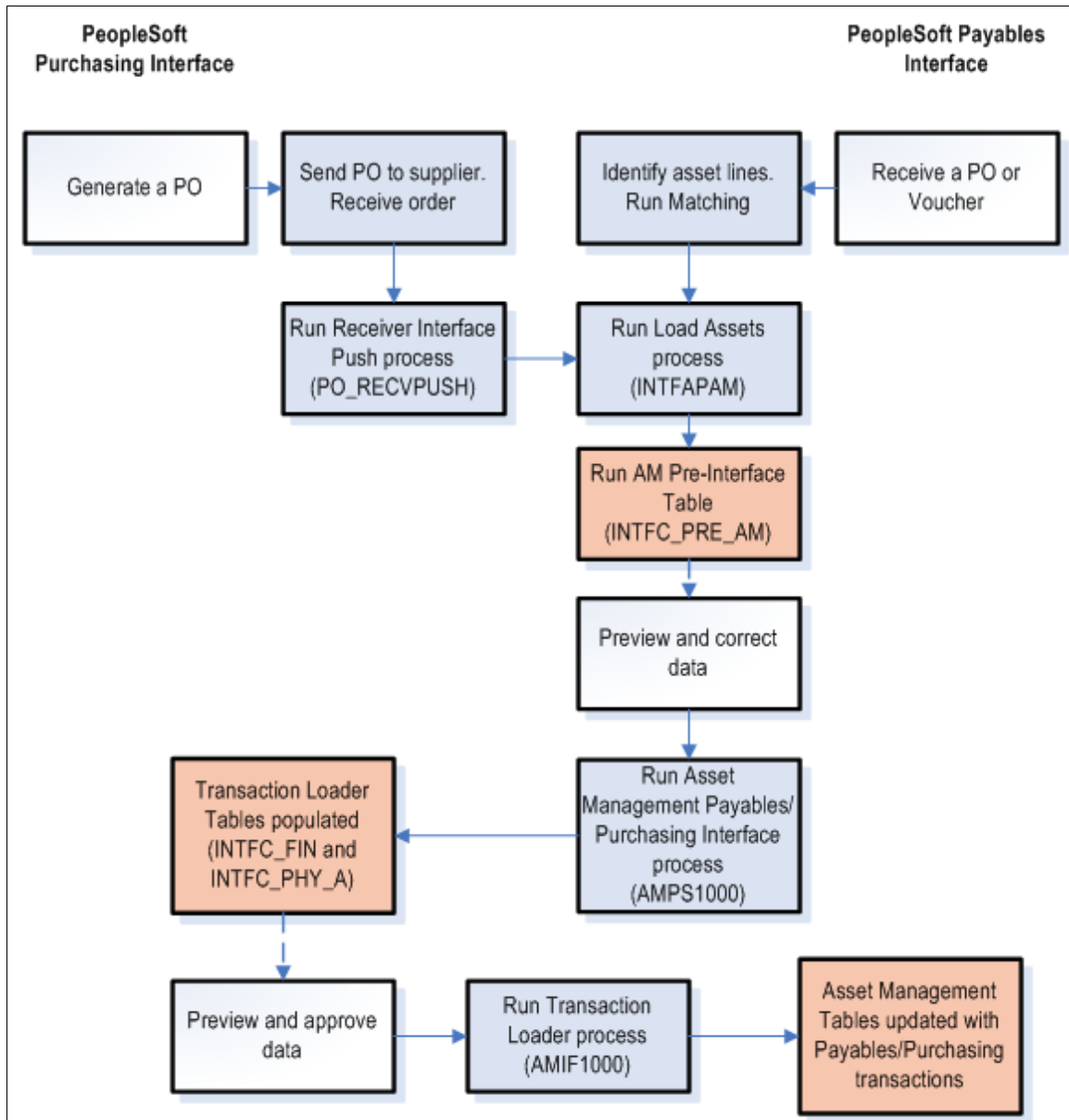
Data Flow Between Asset Management, Purchasing, and Payables
