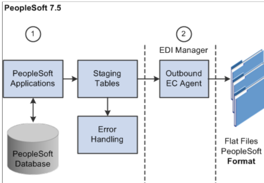
Image: PeopleSoft 7.5 Outbound flat file EDI transaction process (2 of 2)
