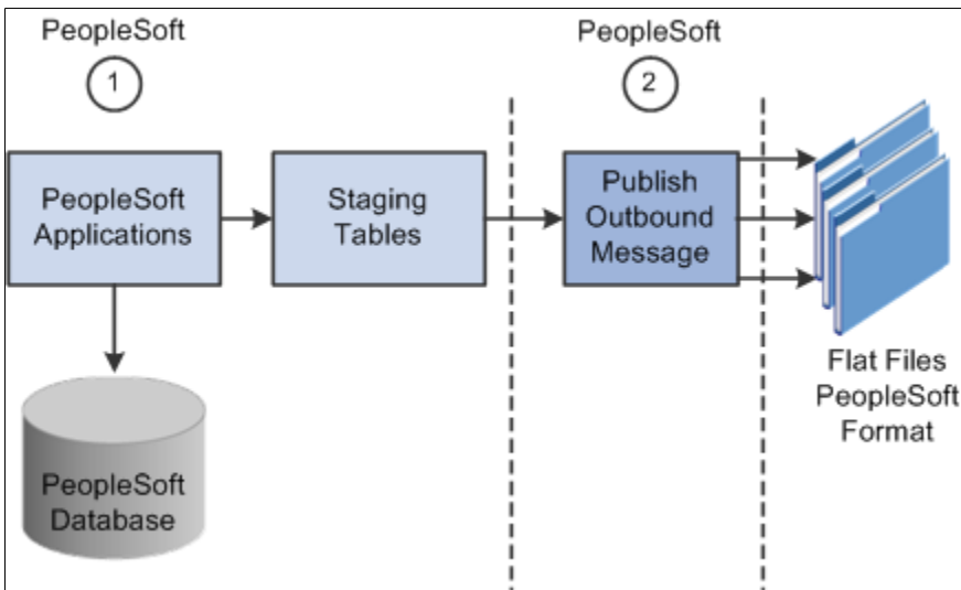
Image: Outbound flat file EDI transaction processing using the PeopleSoft format (2 of 2)
