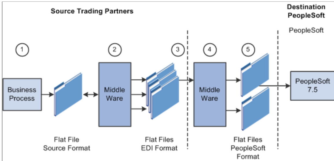
Image: PeopleSoft 7.5 Inbound Flat File EDI Transaction Process (2 of 2)
