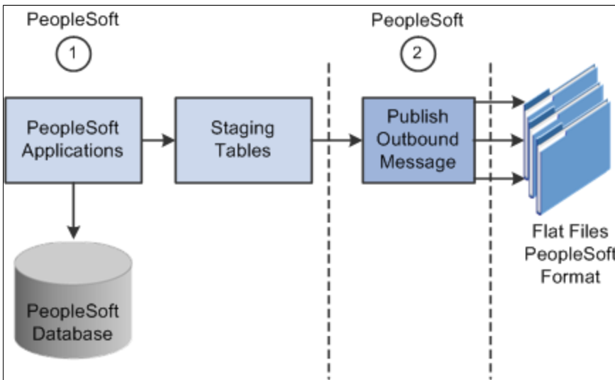
Image: Outbound flat file EDI transaction process for PeopleSoft 9.0 using the PeopleSoft format (2 of 2)
