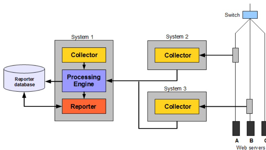
Figure 1–6 Multiple-Collector Deployment
