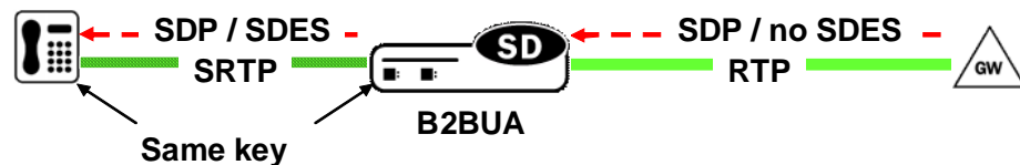
Figure 15 - 1: Single-Ended SRTP Termination
