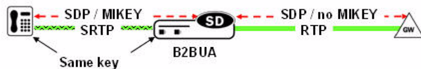
Figure 15 - 4: Single-Ended SRTP Termination
