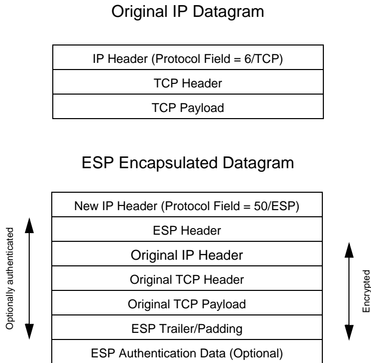
Figure 14: ESP Tunnel Mode
