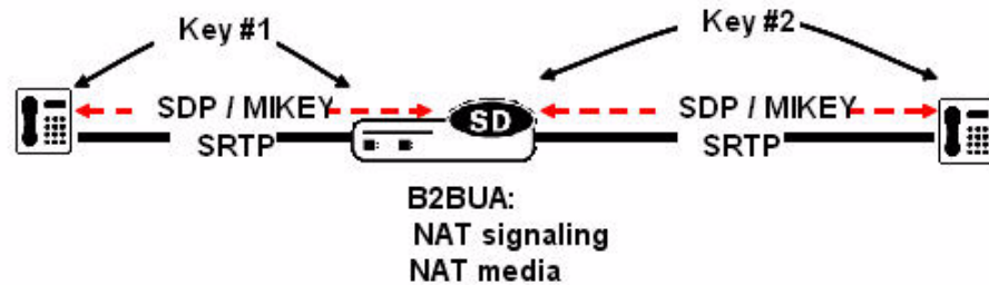
Figure 15 - 5: Back-to-Back SRTP Termination
