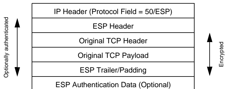
Figure 13: ESP Transport Mode
