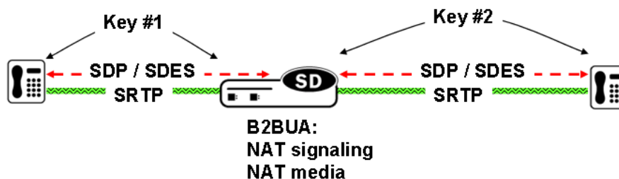
Figure 15 - 2: Back-to-Back SRTP Termination
