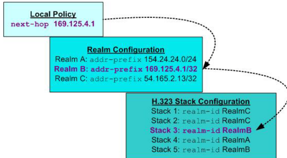
Figure 10-1: Policy-Based Stack Selection
