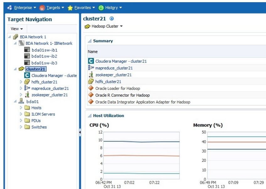
Figure 2–1 Cluster Home in Oracle Enterprise Manager
