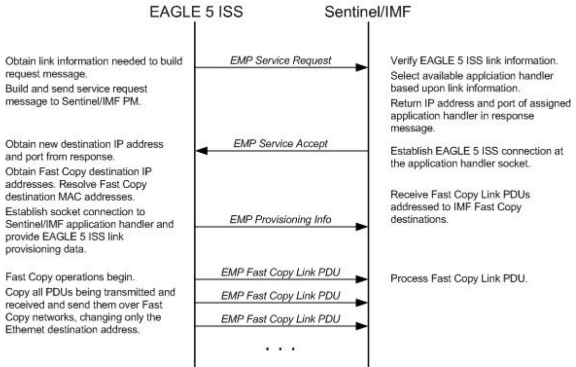
Figure 20: Ethernet Link Establishment - EMP Fast Copy Link PDU
