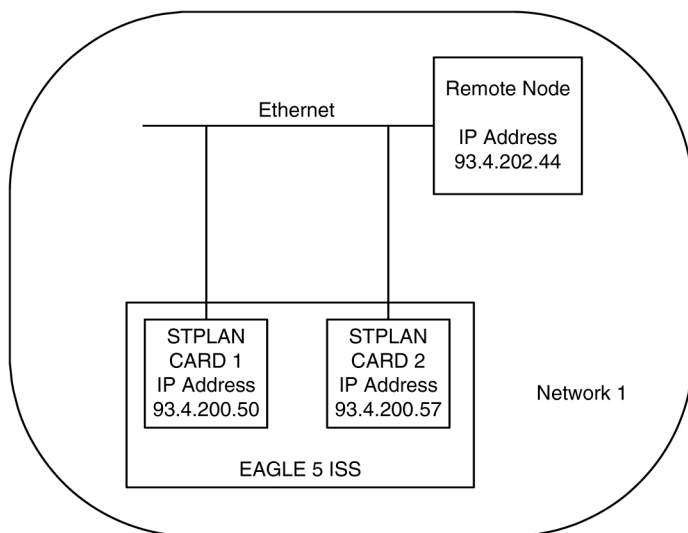
Figure 5: STPLAN in a Large Network
