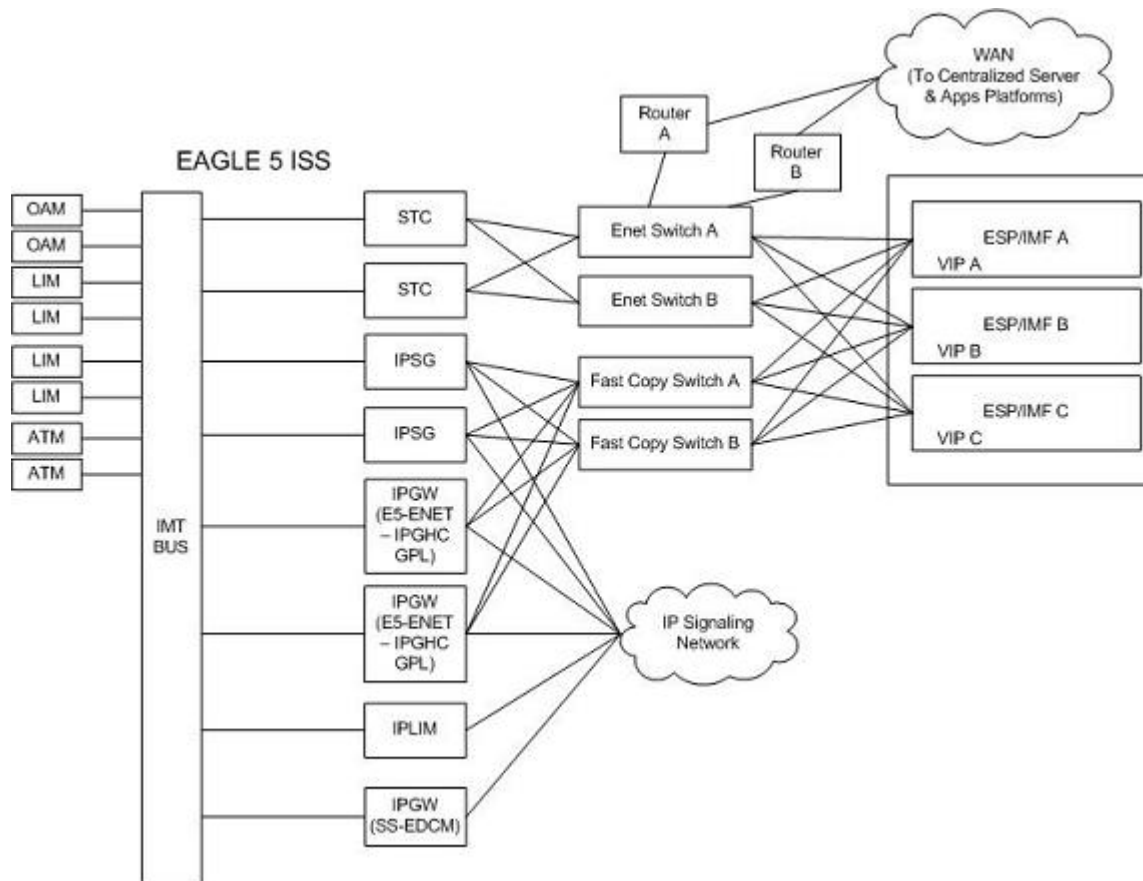
Figure 18: ESP/IMF/EAGLE 5 ISS Network
