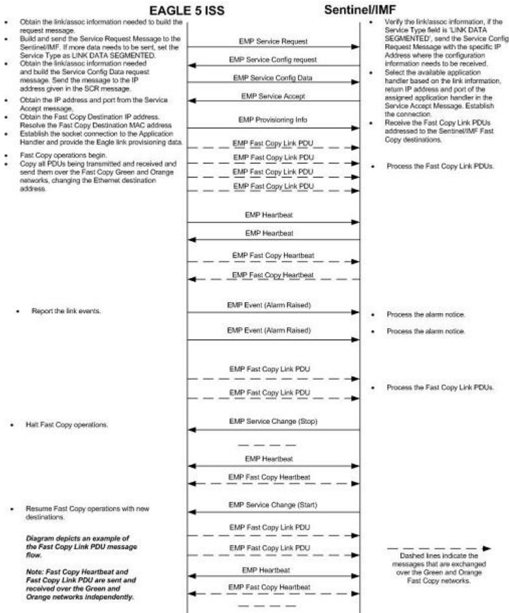
Figure 21: Ethernet Link Establishment - EMP Fast Copy Link PDU Modified for the IPGHC GPL
