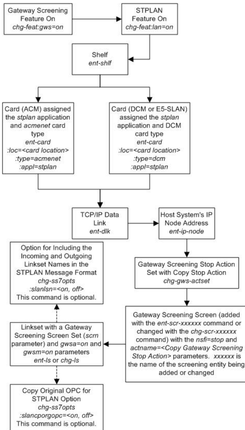
Figure 8: STPLAN Database Relationships
