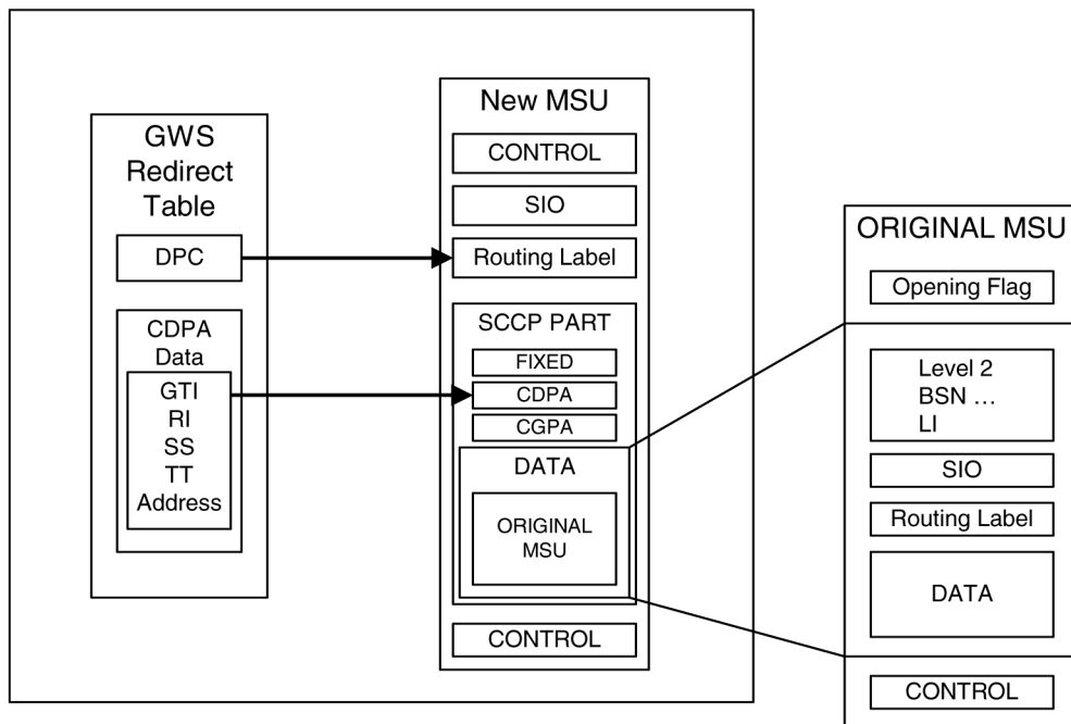
Figure 11: DTA Encapsulation
