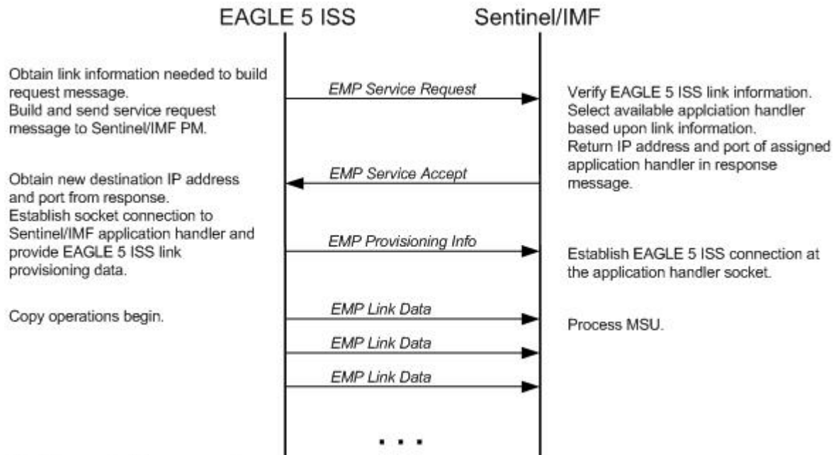
Figure 19: Ethernet Link Establishment - EMP Link Data
