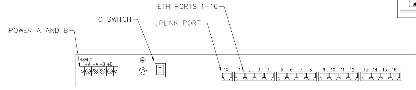
DETAIL G REAR VIEW-HUB
