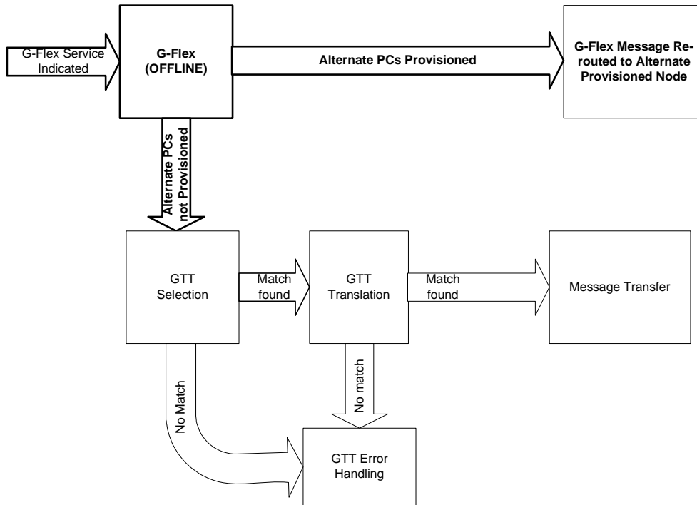
Figure 2-13. Functional Diagram – G-Flex SCCP Service Re-Route (OFFLINE)
