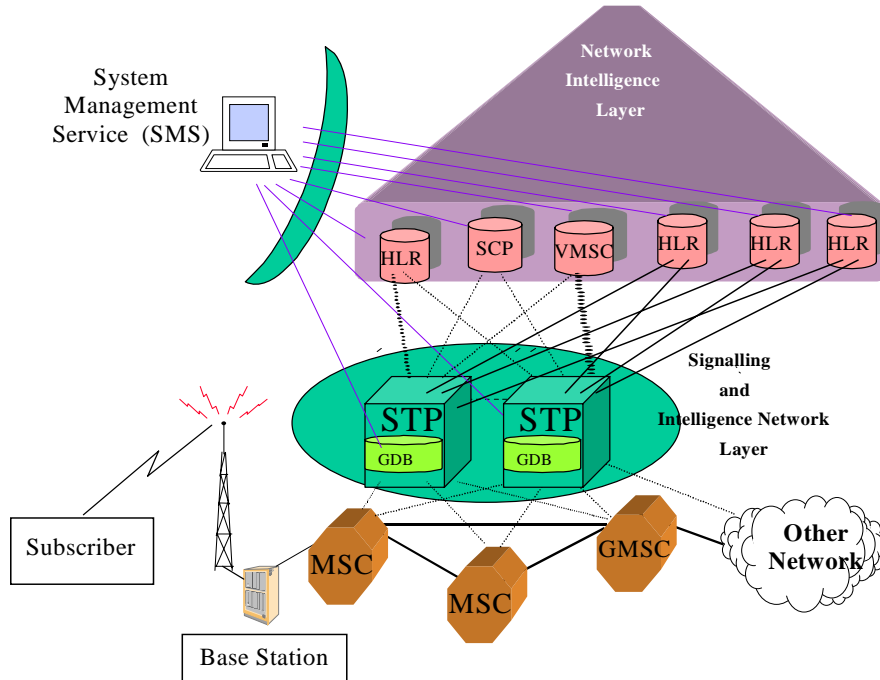
Figure 2-10. Location of an Integrated EAGLE 5 ISS/G-Flex Node in Wireless Network
