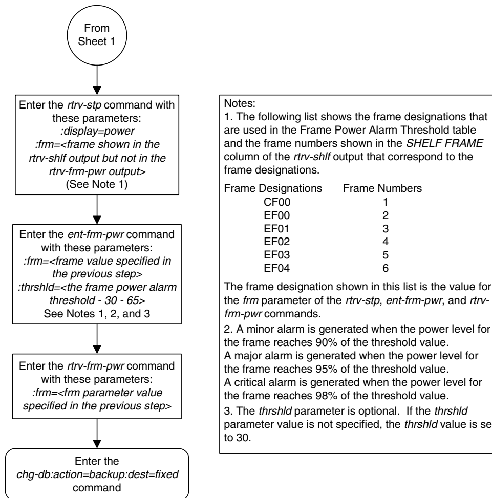
Flowchart 4-30. Adding an Entry to the Frame Power Alarm Threshold Table (Sheet 2 of 2)
