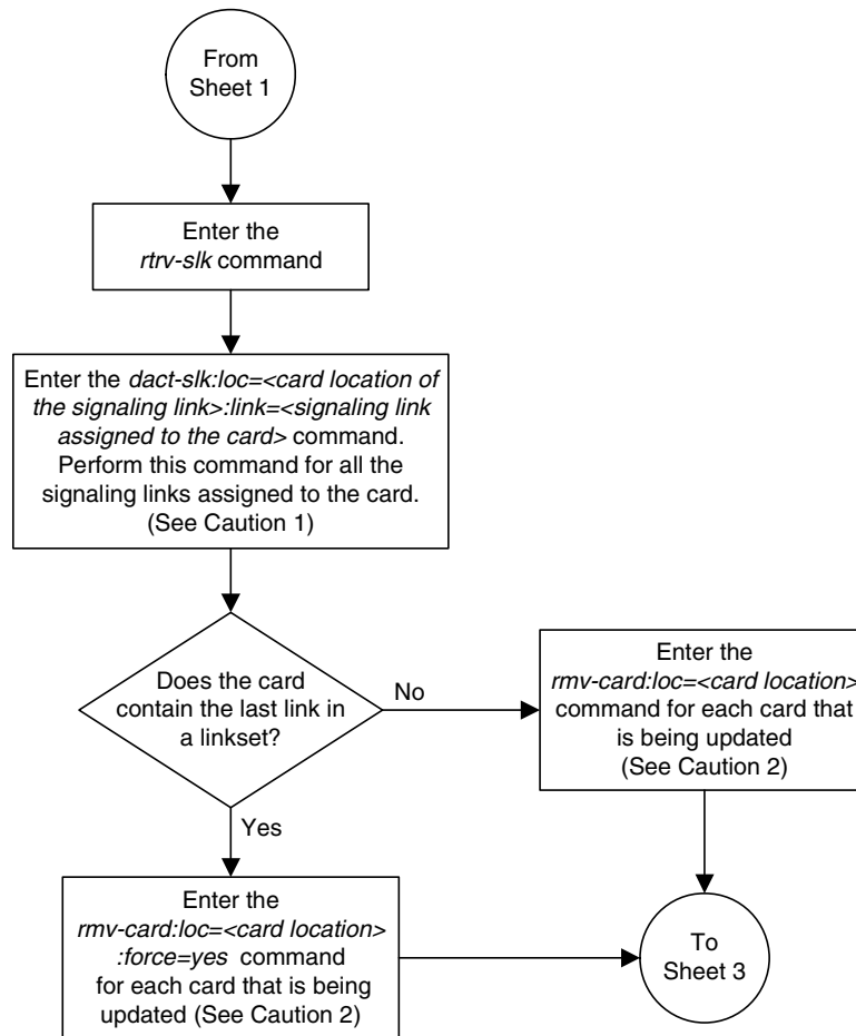
Flowchart 3-6. Updating One of the Flash GPLs on the HC MIMs, E5-ENET Cards, or E5-E1T1 Cards (Sheet 2 of 5)
