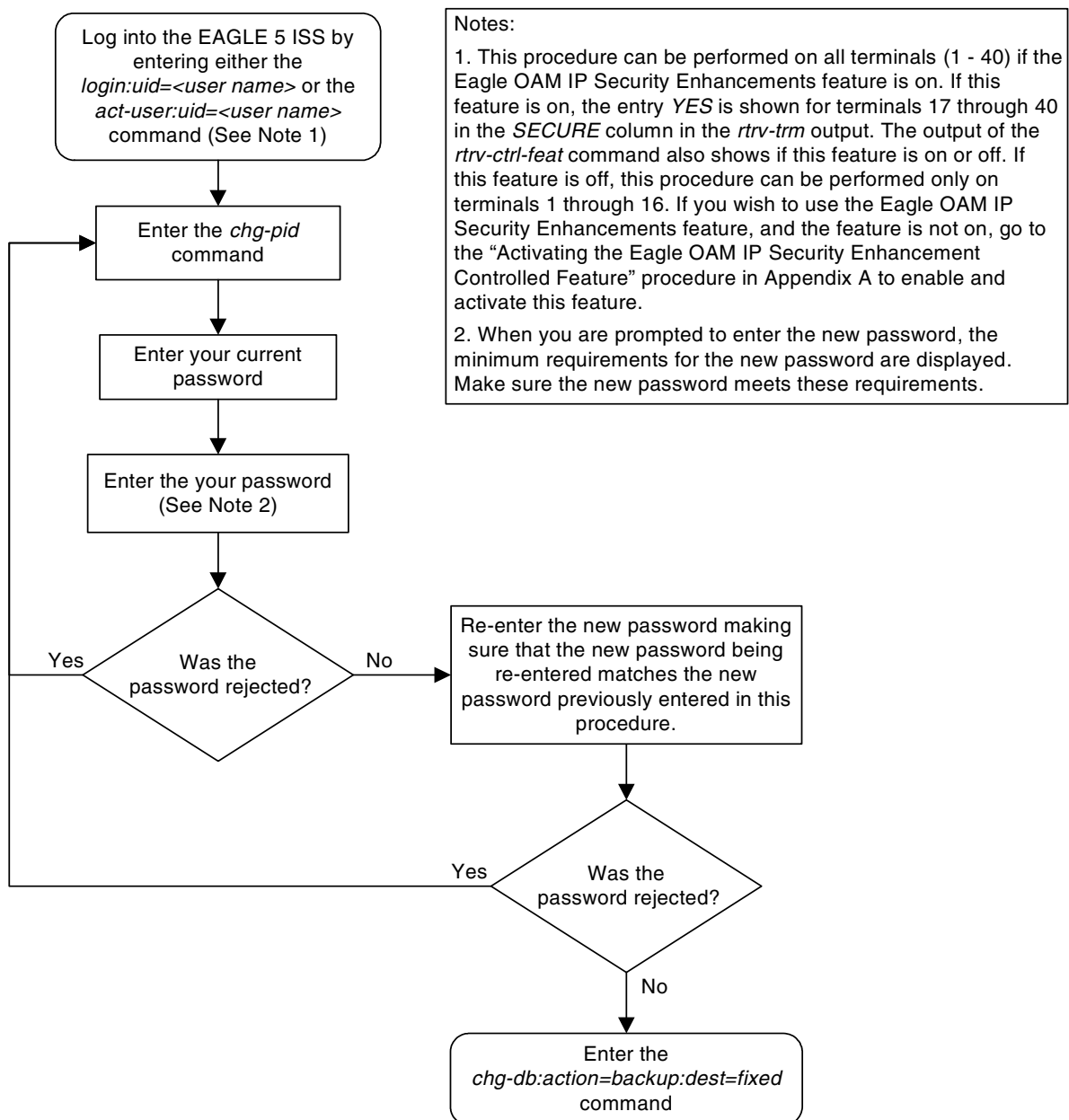
Flowchart 4-9. Changing a Password
