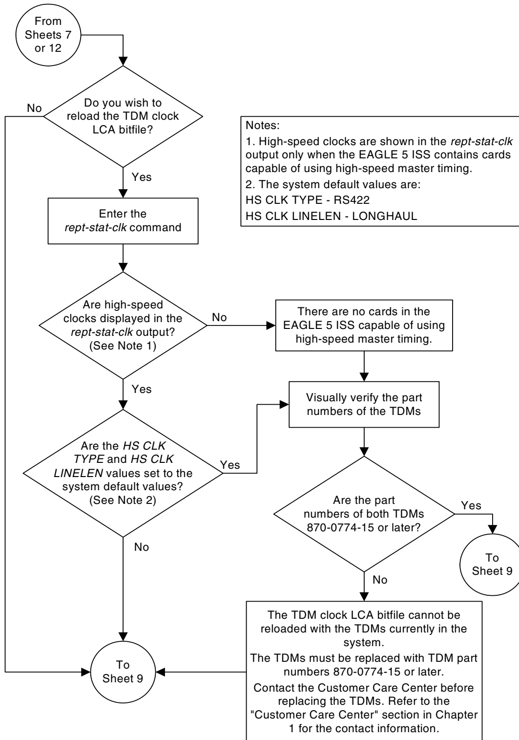
Flowchart 3-5. Updating the Flash GPLs (Sheet 8 of 13)
