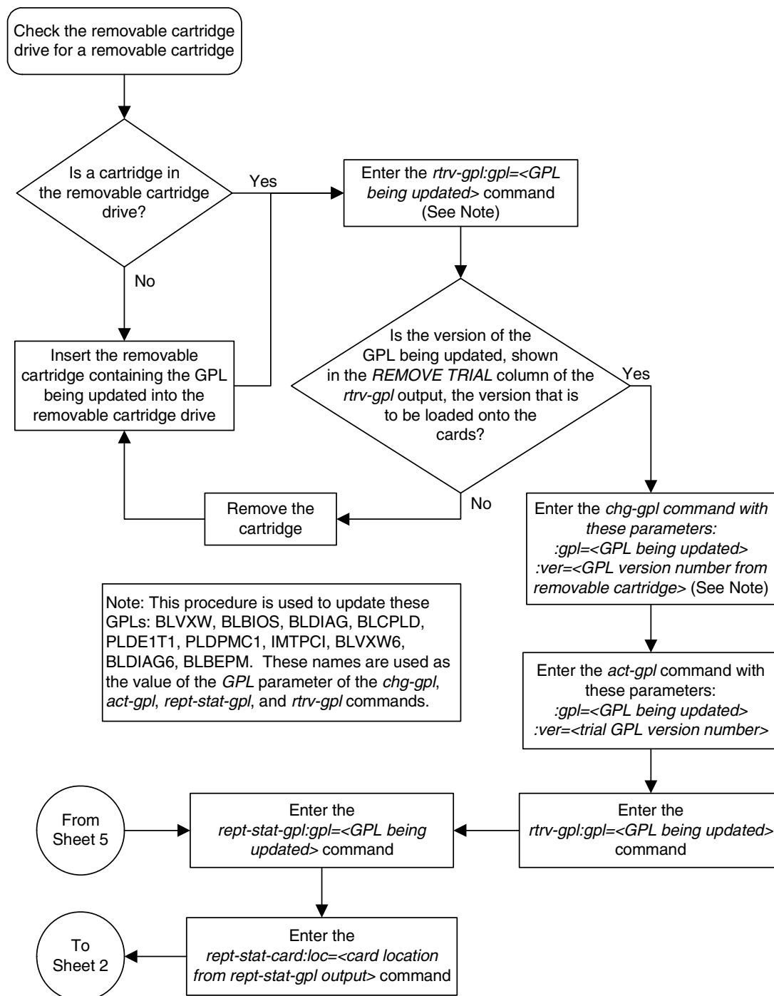
Flowchart 3-6. Updating One of the Flash GPLs on the HC MIMs, E5-ENET Cards, or E5-E1T1 Cards (Sheet 1 of 5)
