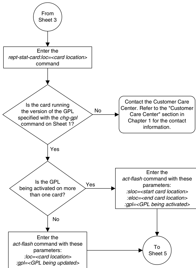
Flowchart 3-6. Updating One of the Flash GPLs on the HC MIMs, E5-ENET Cards, or E5-E1T1 Cards (Sheet 4 of 5)
