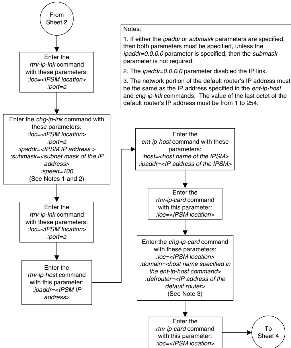
Flowchart 4-26. Adding an IPSM (Sheet 3 of 4)
