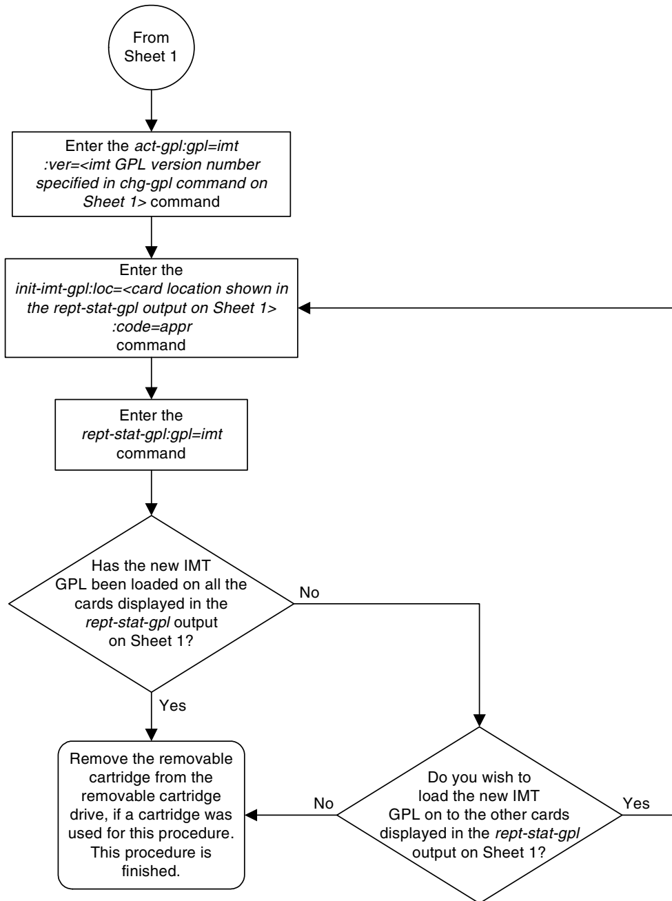
Flowchart 3-1. Updating the IMT GPL (Sheet 2 of 2)
