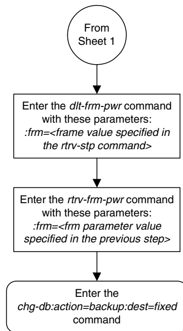
Flowchart 4-31. Removing an Entry from the Frame Power Alarm Threshold Table (Sheet 2 of 2)
