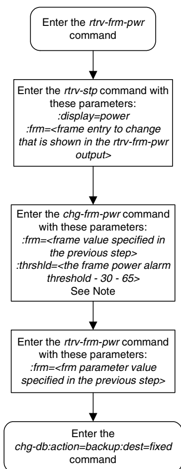
Flowchart 4-32. Changing an Entry in the Frame Power Alarm Threshold Table
