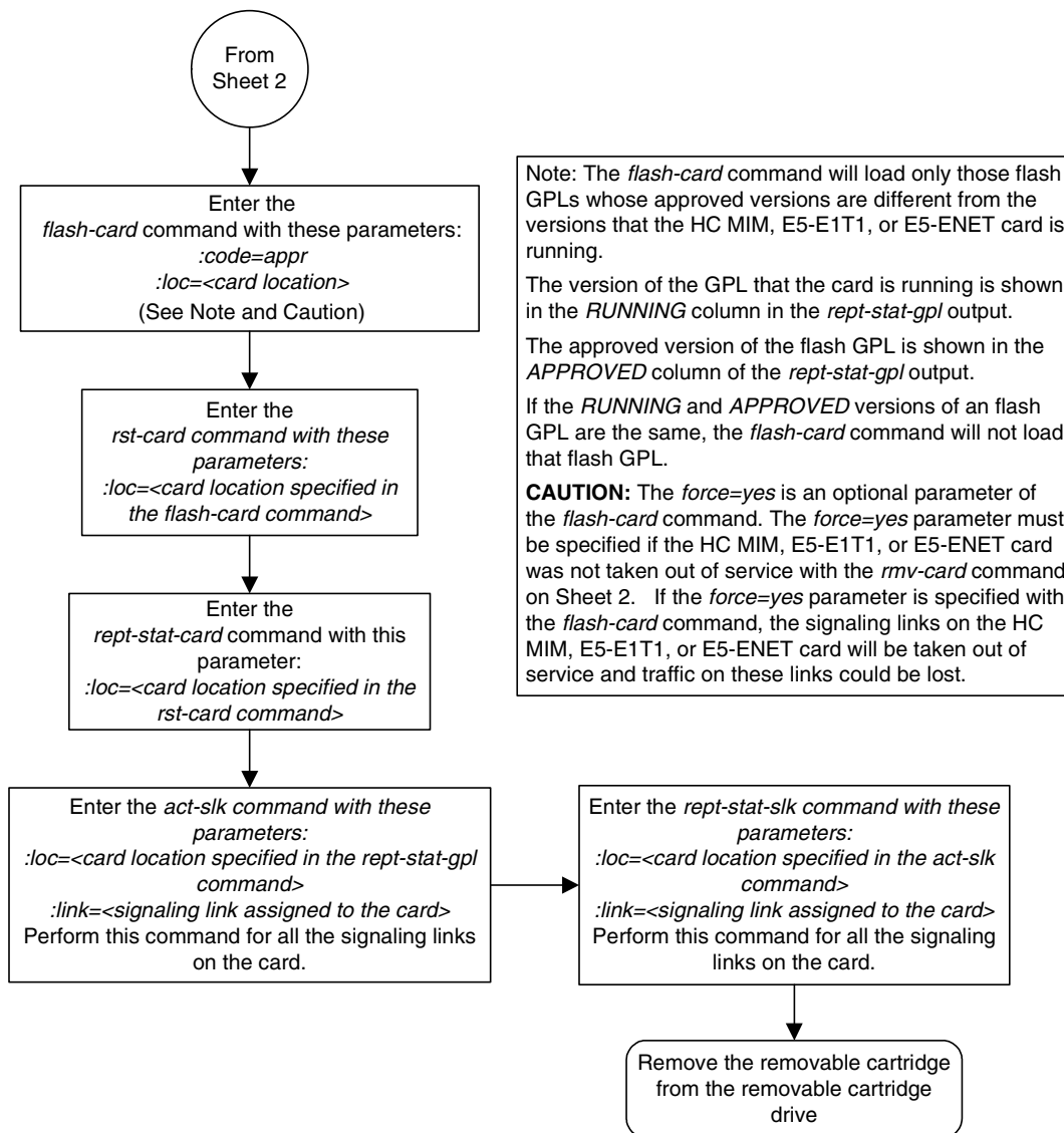
Flowchart 3-7. Updating All the Flash GPLs on the HC MIMs, E5-ENET Cards, or E5-E1T1 Cards (Sheet 3 of 3)
