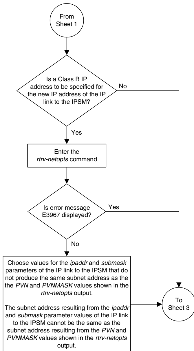
Flowchart 4-26. Adding an IPSM (Sheet 2 of 4)
