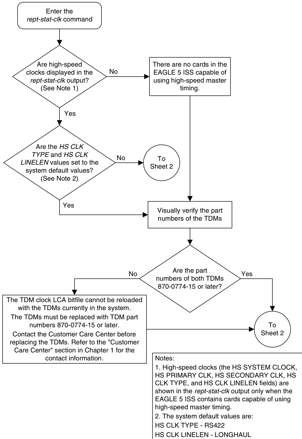
Flowchart 3-12. Reloading the TDM LCA Clock Bitfile (Sheet 1 of 4)
