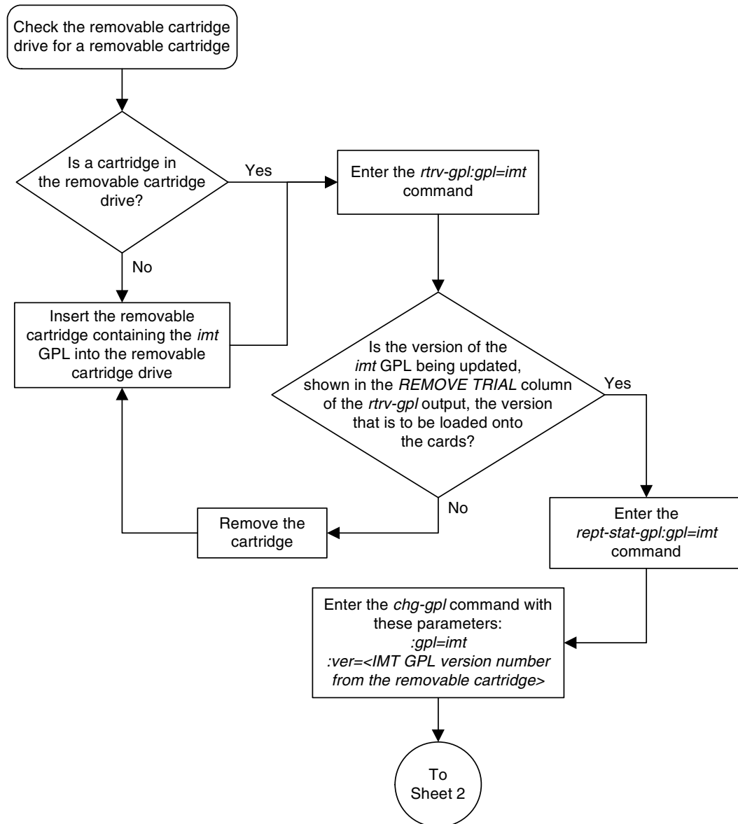
Flowchart 3-1. Updating the IMT GPL (Sheet 1 of 2)
