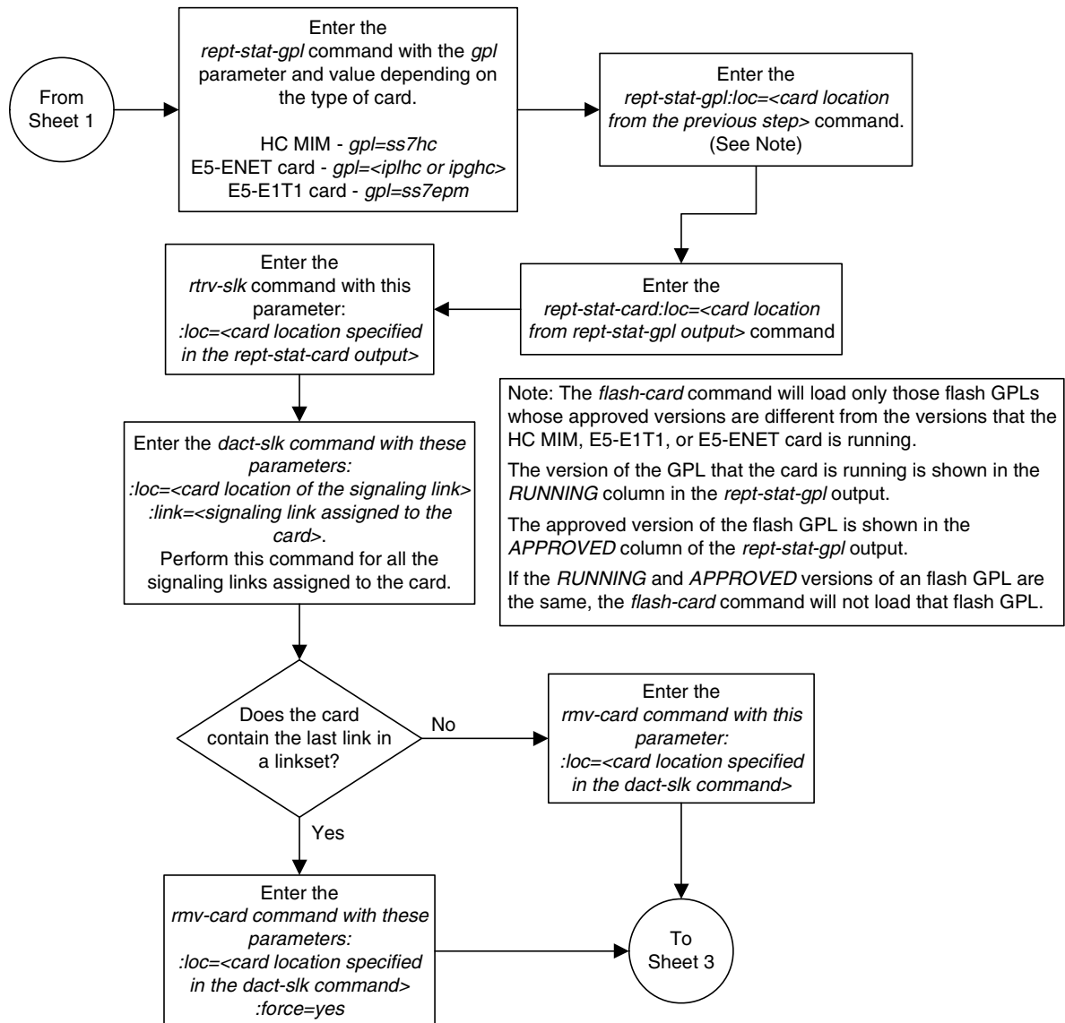
Flowchart 3-7. Updating All the Flash GPLs on the HC MIMs, E5-ENET Cards, or E5-E1T1 Cards (Sheet 2 of 3)
