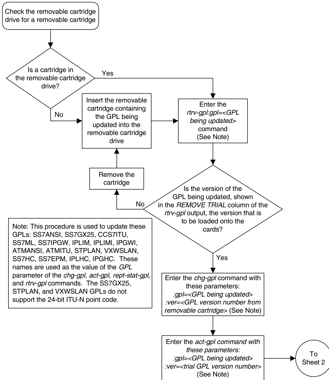
Flowchart 3-3. Updating the Signaling Link and Data Link GPLs (Sheet 1 of 3)
