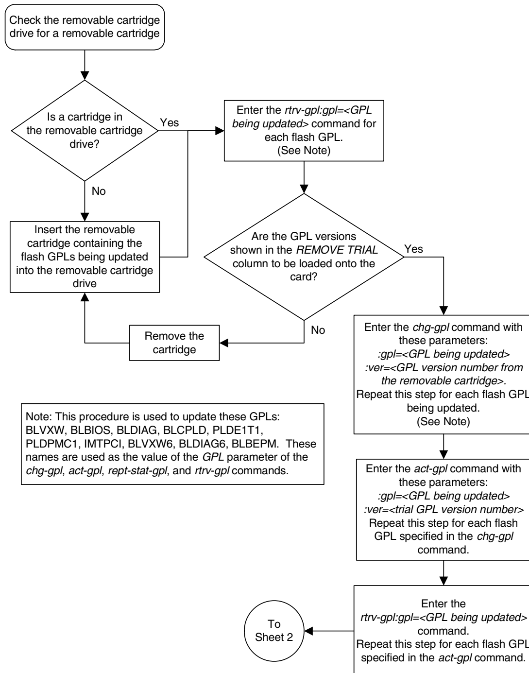
Flowchart 3-7. Updating All the Flash GPLs on the HC MIMs, E5-ENET Cards, or E5-E1T1 Cards (Sheet 1 of 3)
