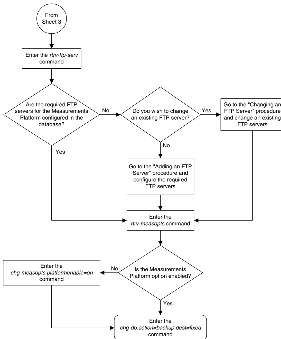
Flowchart 4-22. Configuring the Measurements Platform Feature (Sheet 4 of 4)
