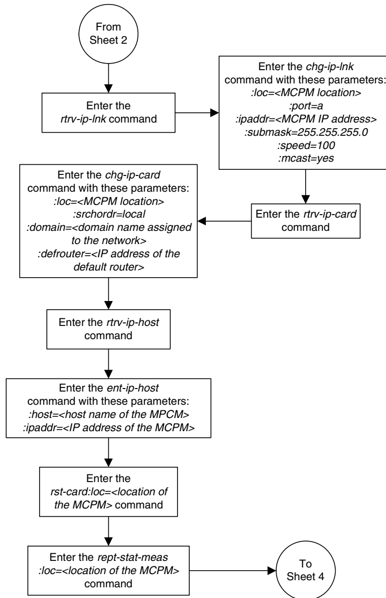
Flowchart 4-22. Configuring the Measurements Platform Feature (Sheet 3 of 4)
