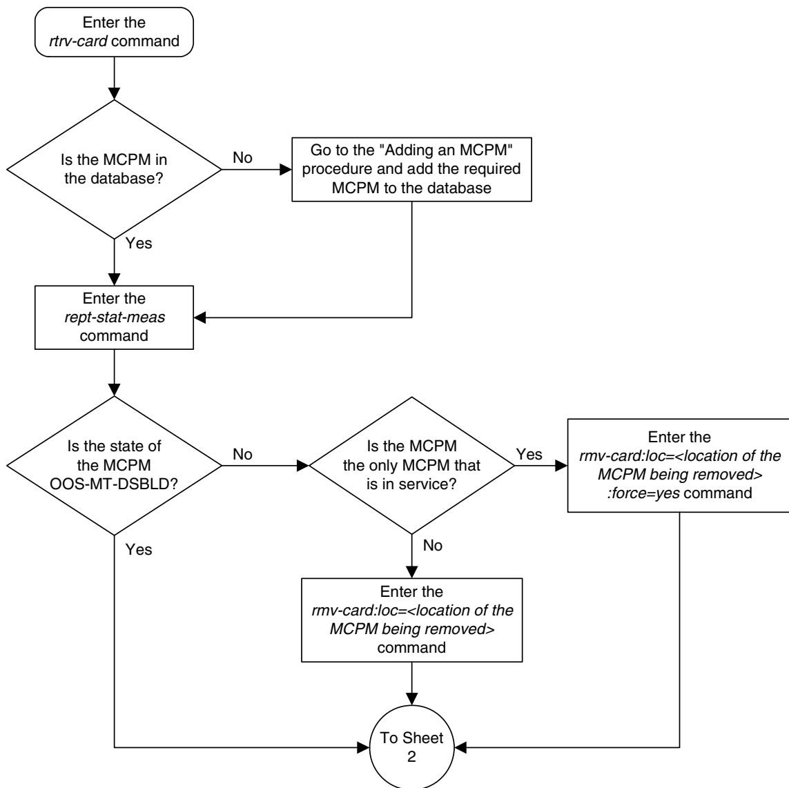
Flowchart 4-22. Configuring the Measurements Platform Feature (Sheet 1 of 4)
