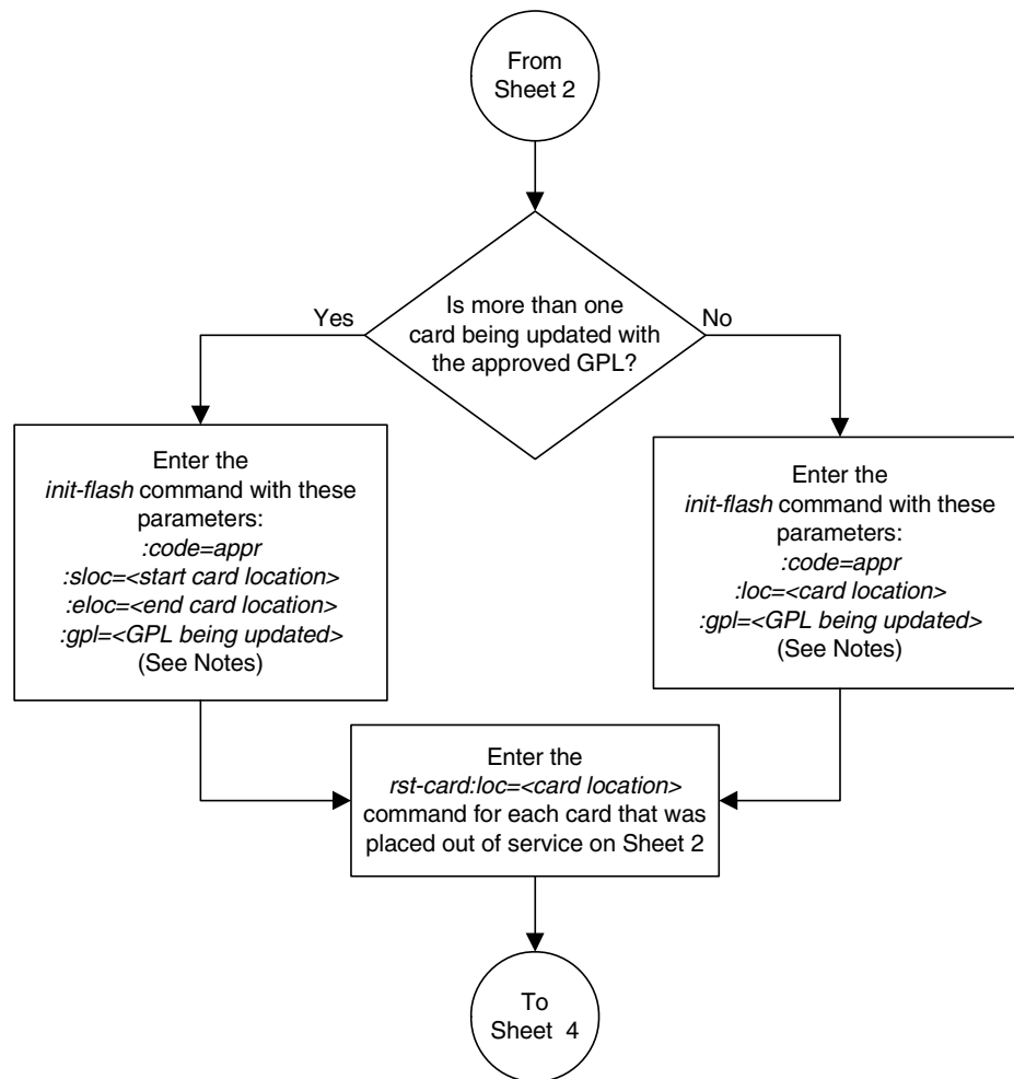
Flowchart 3-6. Updating One of the Flash GPLs on the HC MIMs, E5-ENET Cards, or E5-E1T1 Cards (Sheet 3 of 5)
