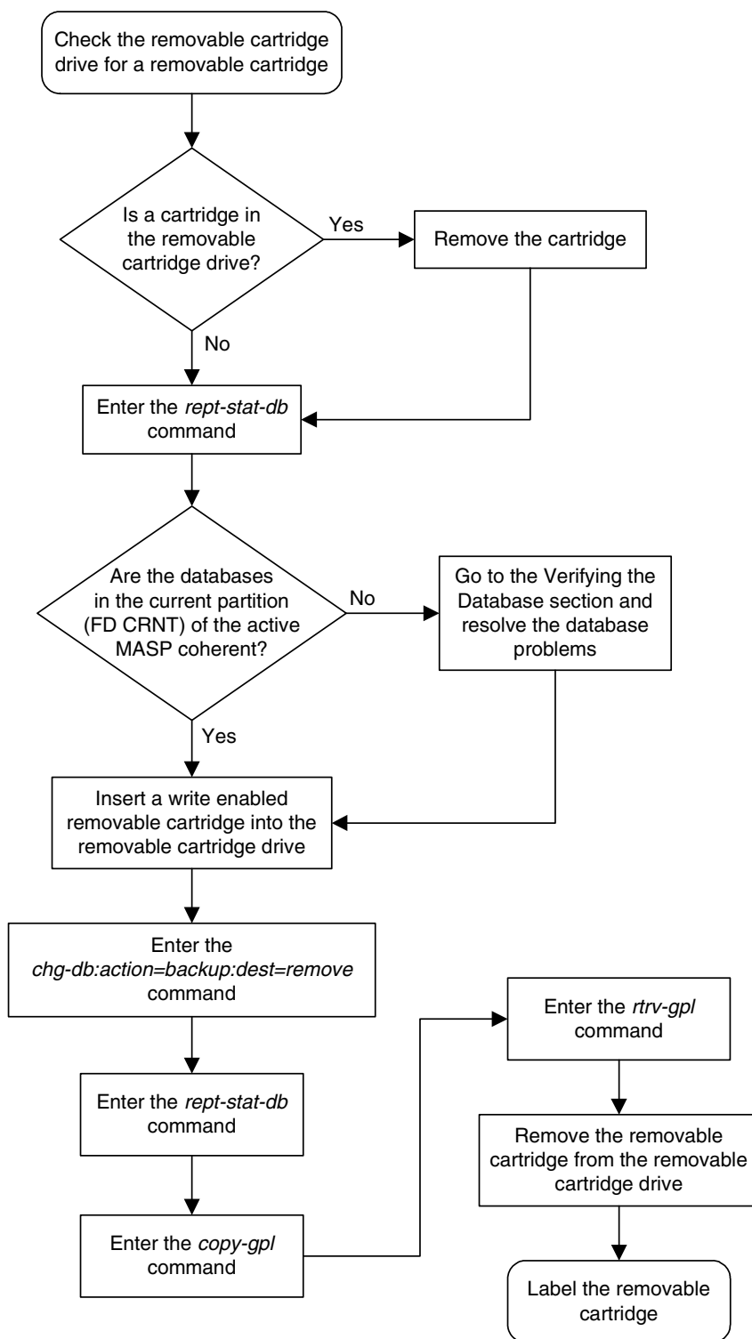
Flowchart 2-7. Backing Up System Data to the Removable Cartridge
