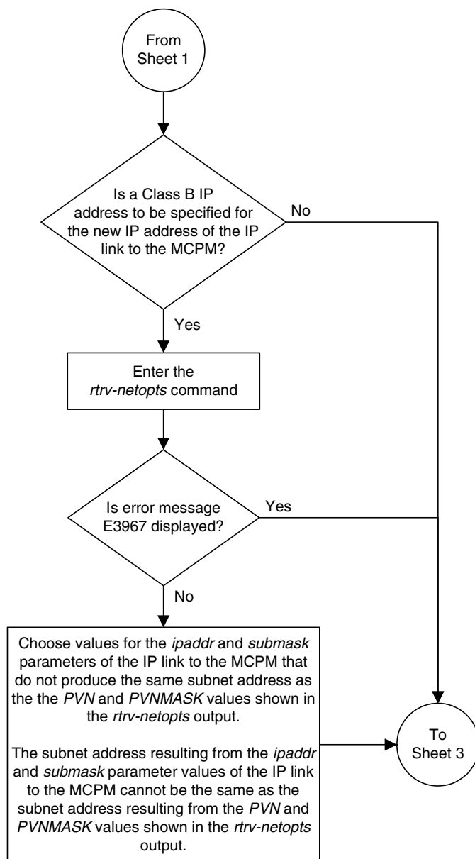
Flowchart 4-22. Configuring the Measurements Platform Feature (Sheet 2 of 4)
