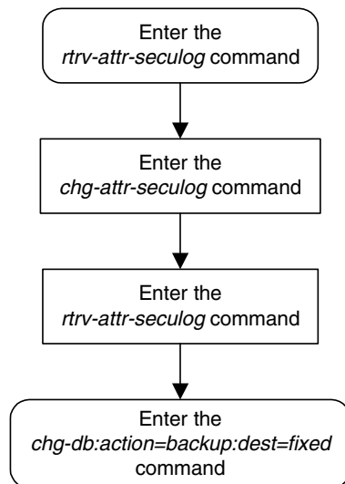
Flowchart 4-4. Changing the Security Log Characteristics
