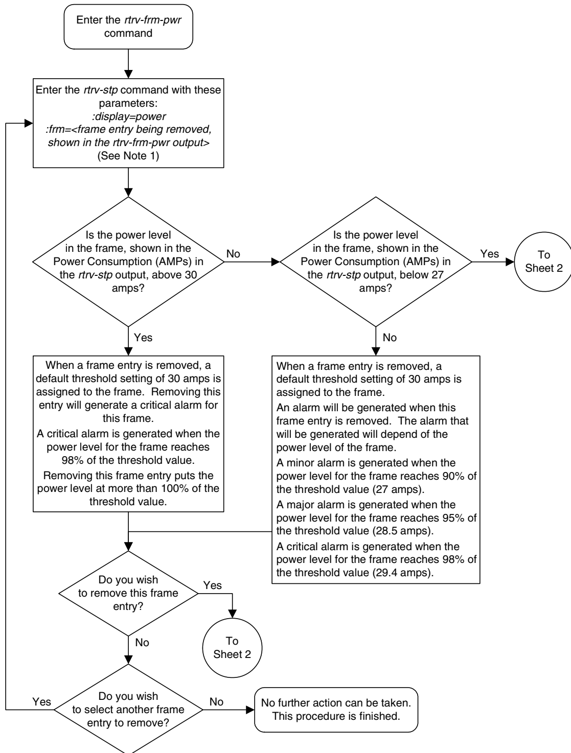
Flowchart 4-31. Removing an Entry from the Frame Power Alarm Threshold Table (Sheet 1 of 2)
