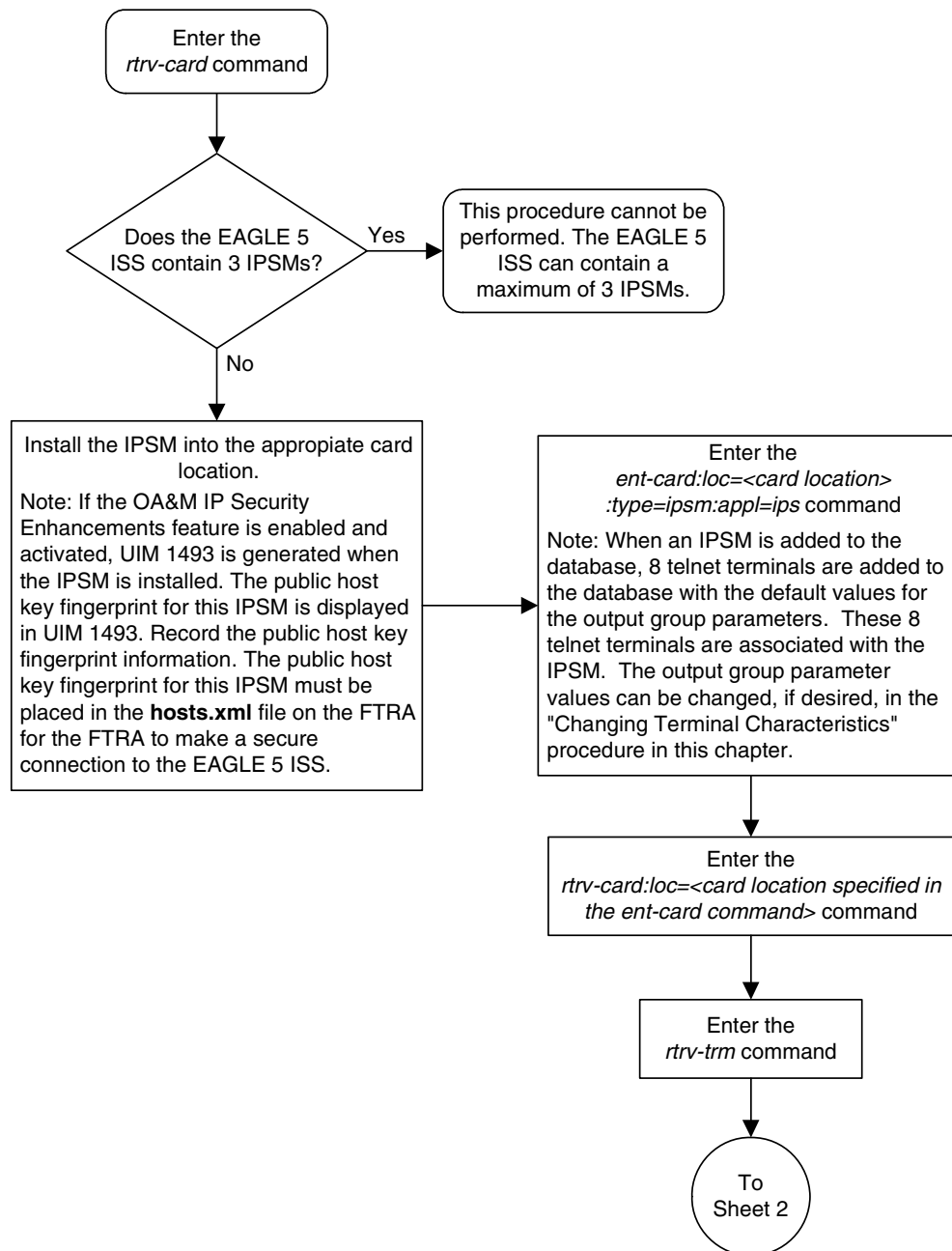
Flowchart 4-26. Adding an IPSM (Sheet 1 of 4)
