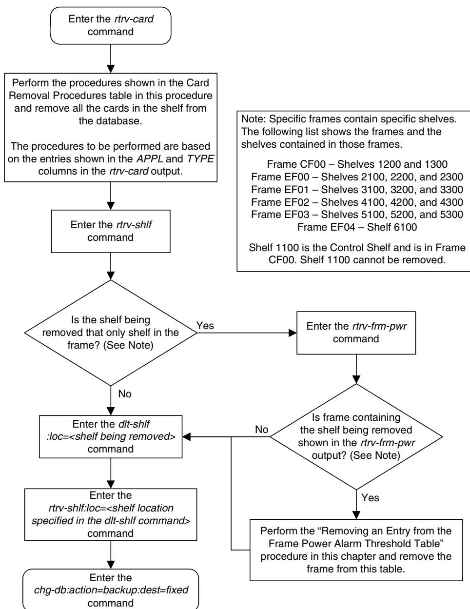
Flowchart 4-14. Removing a Shelf
