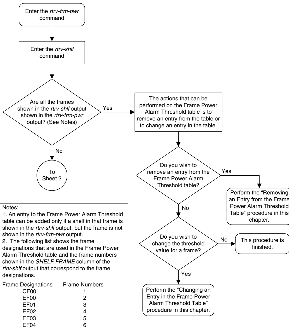
Flowchart 4-30. Adding an Entry to the Frame Power Alarm Threshold Table (Sheet 1 of 2)
