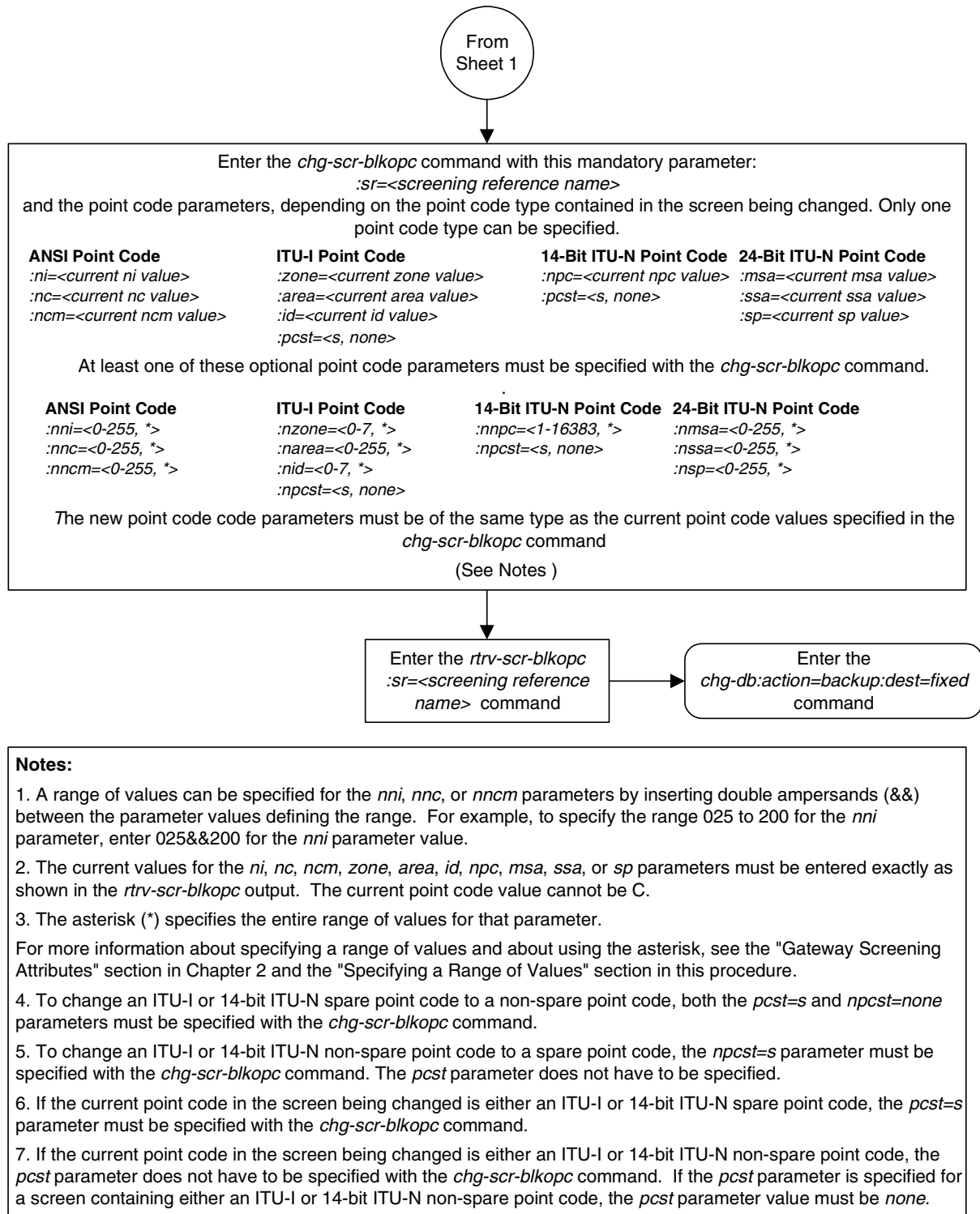
Flowchart 11-4. Changing a Blocked OPC Screen (Sheet 2 of 5)
