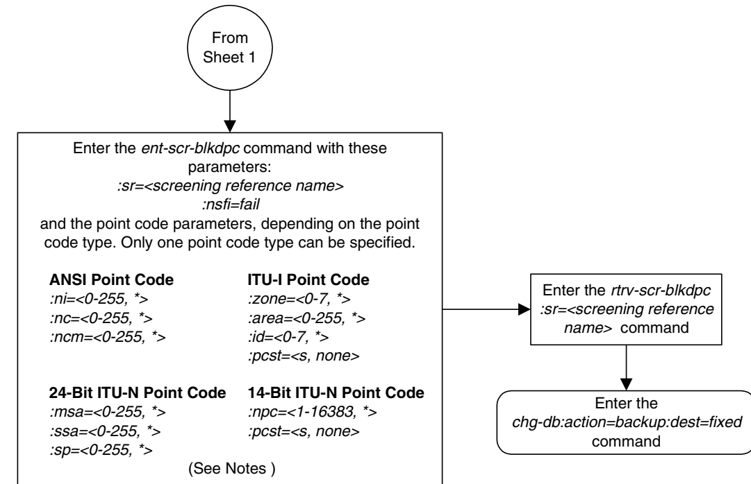
Flowchart 8-2. Adding a Blocked DPC Screen (Sheet 2 of 5)
