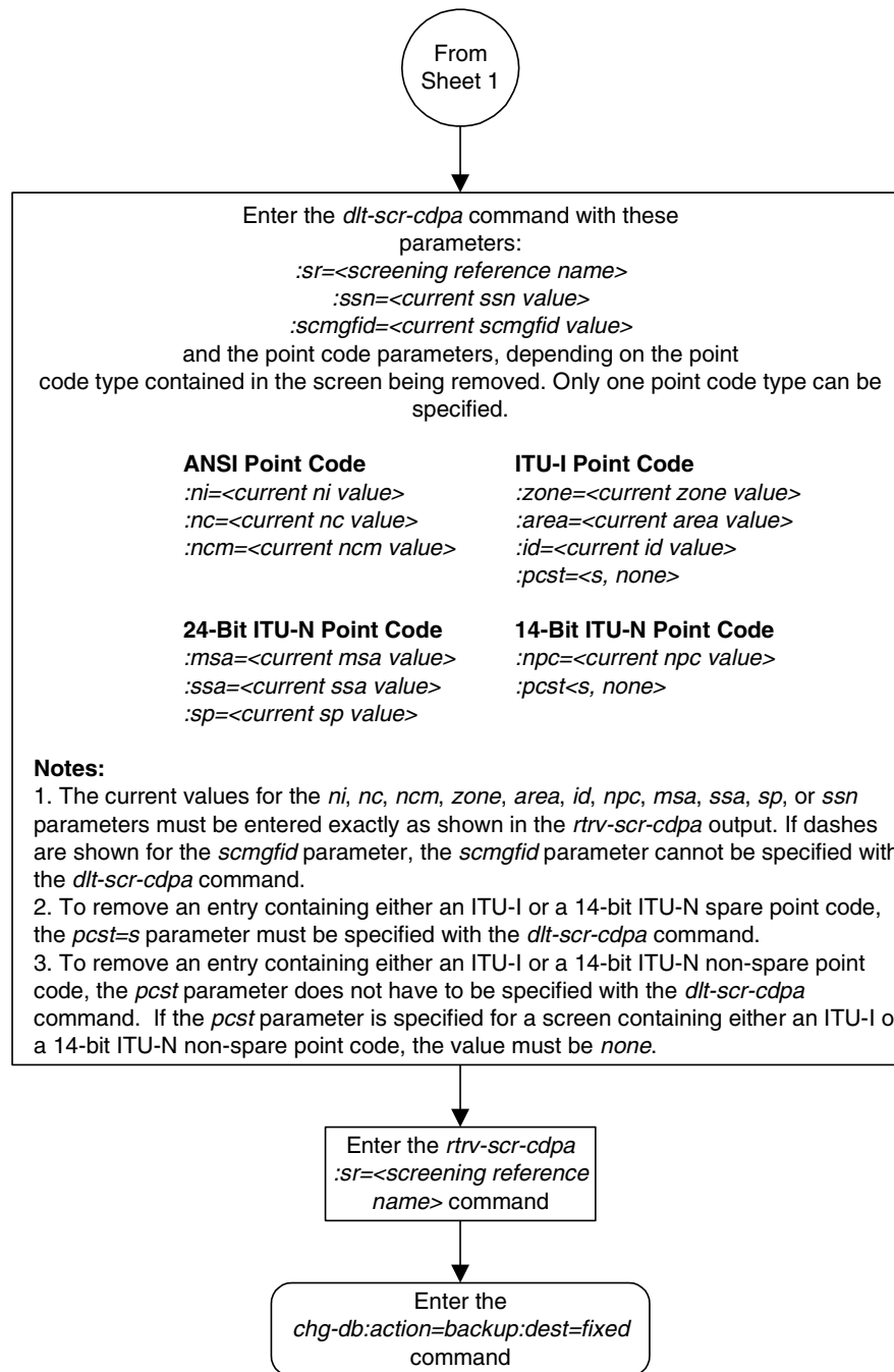
Flowchart 4-3. Removing an Allowed Called Party Address Screen (Sheet 2 of 2)
