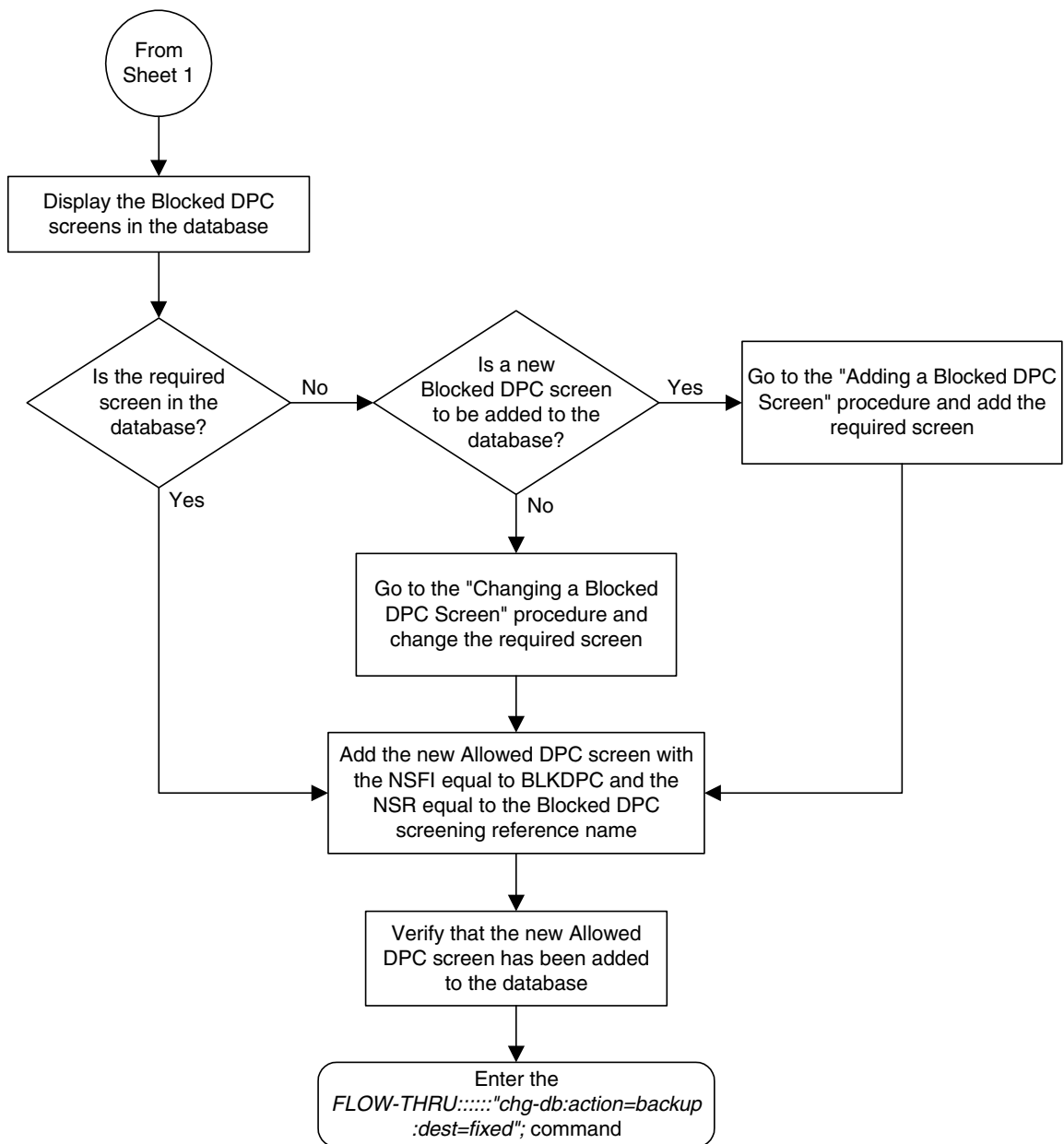
Flowchart 5-19. Adding an Allowed DPC Screen from the SEAS Terminal (Sheet 2 of 5)
