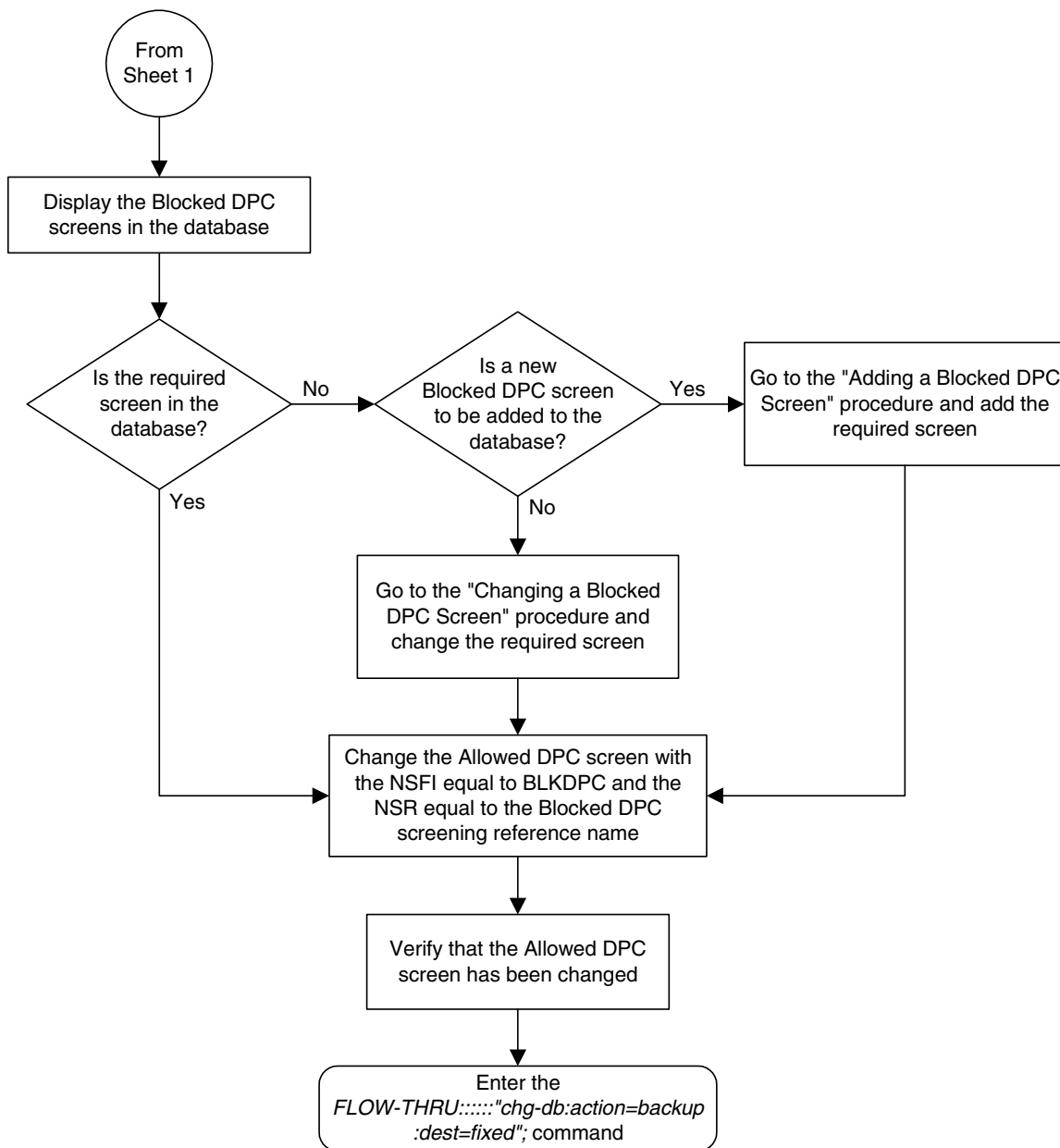
Flowchart 5-21. Changing an Allowed DPC Screen from the SEAS Terminal (Sheet 2 of 5)
