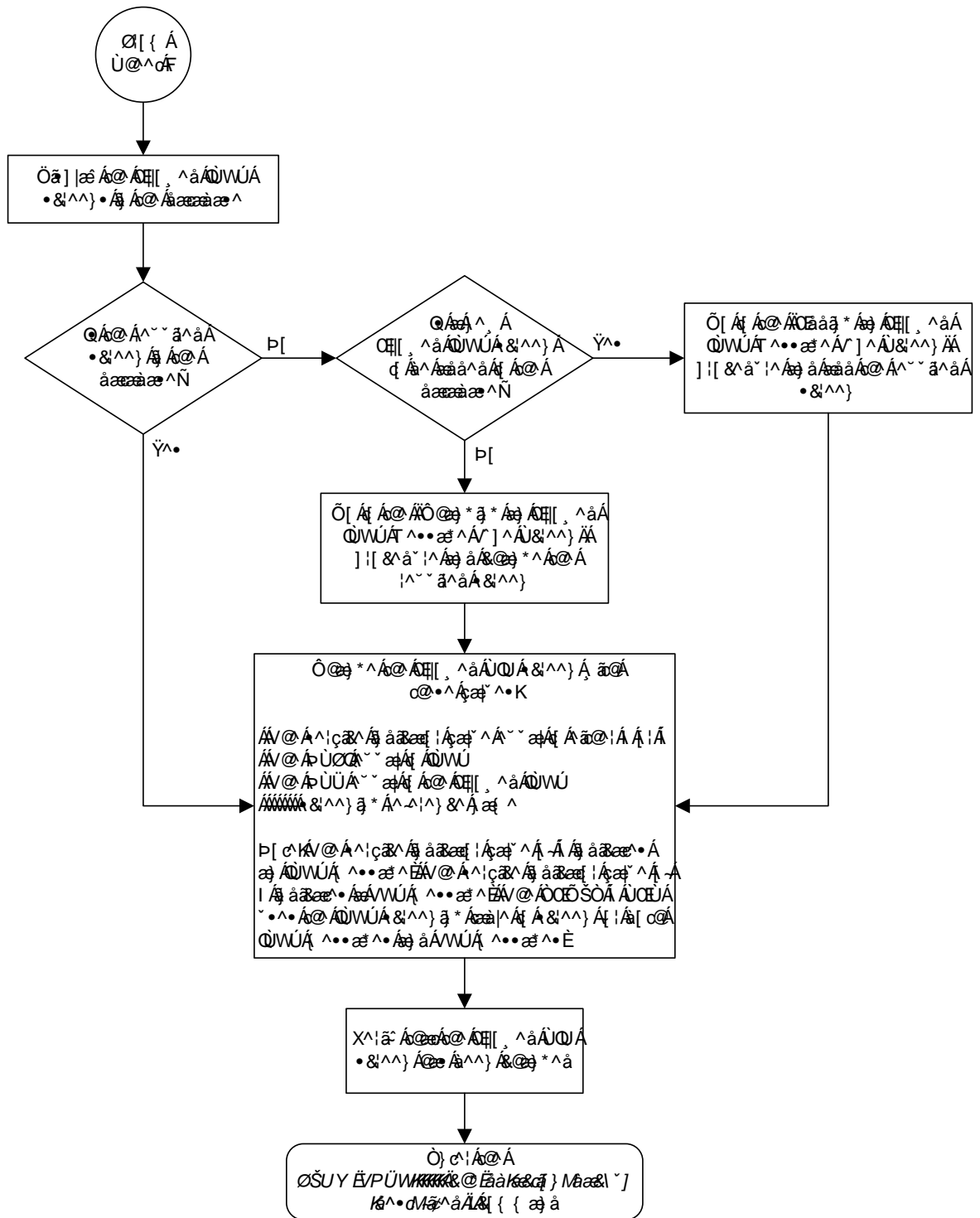
Flowchart 5-24. Changing an Allowed SIO Screen from the SEAS Terminal (Sheet 7 of 7)
