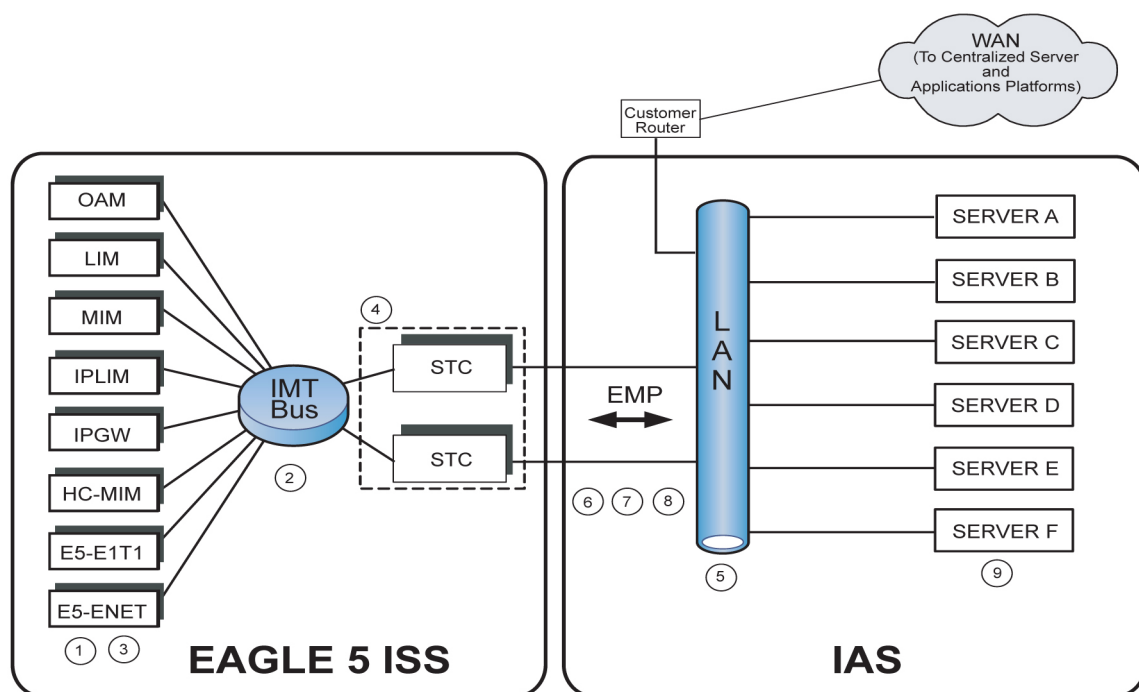
Figure 5: EAGLE-IAS Interfacing
