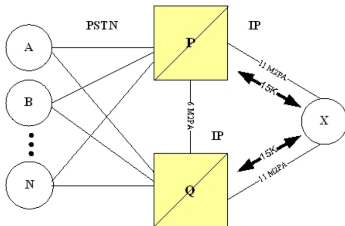
Figure 20: SG connected to IP SEP via eleven M2PA links
