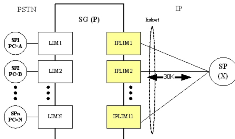
Figure 19: SG connected to IP SEP via eleven M2PA links
