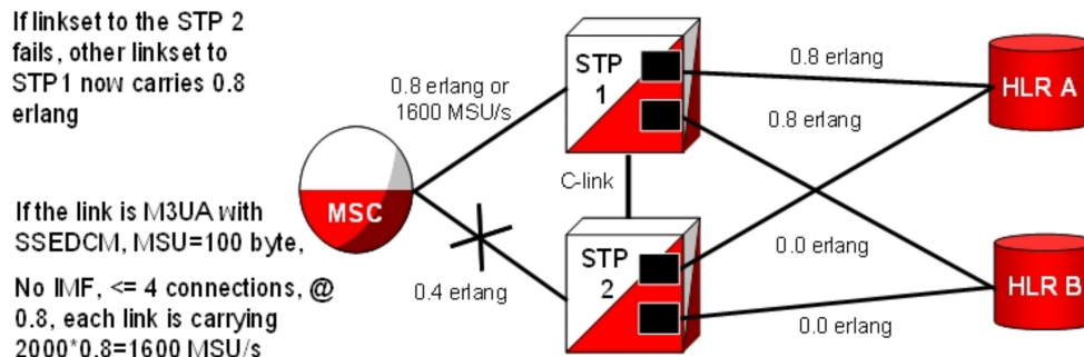
Figure 11: EAGLE 5 ISS: Failover at 0.8 Erlang and 1600 MSU/s
