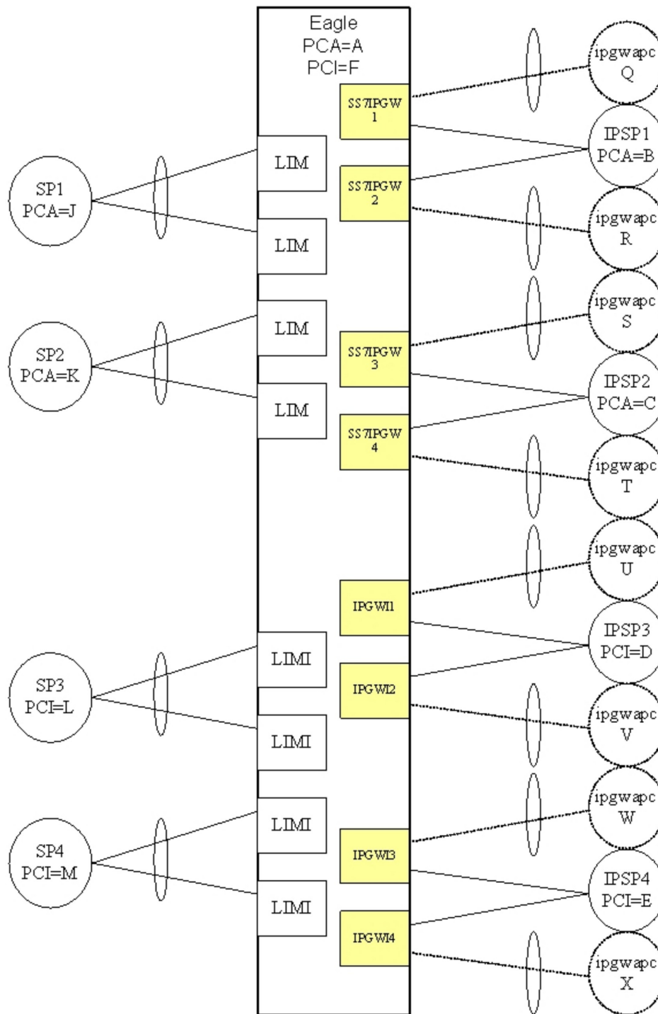
Figure 23: Four IPGWx pairs (two SS7IPW pairs and two IPGWI pairs)
