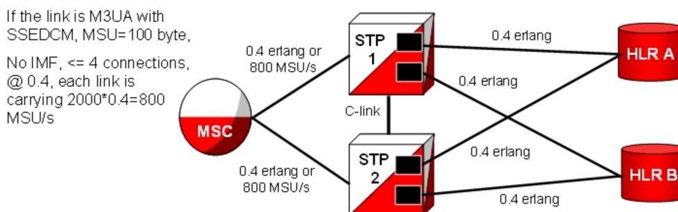
Figure 10: SIGTRAN: Every Link at 0.4 Erlang and 800 MSU/s
