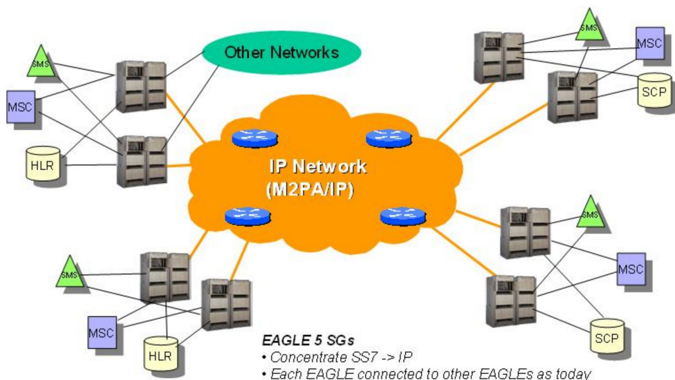
Figure 3: M2PA Network
