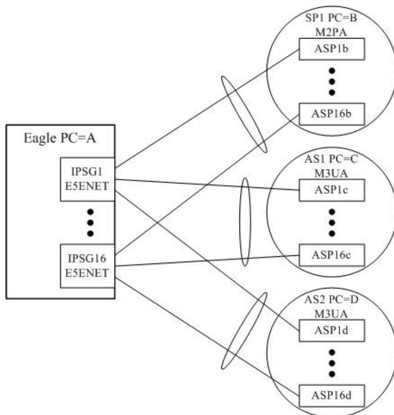
Figure 17: Example Deployment of IPSG Application
