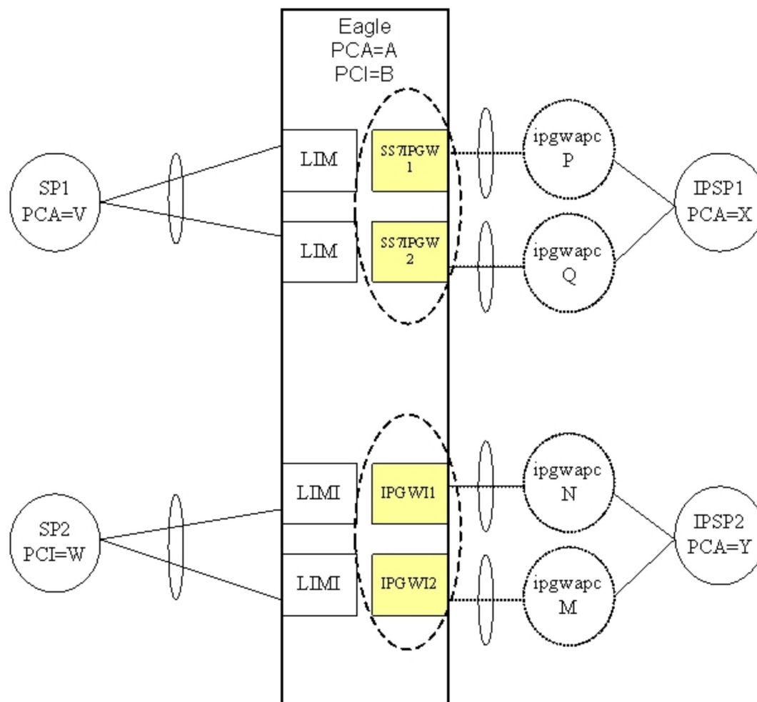
Figure 22: Two-Pair IPGWx for maximum TPS
