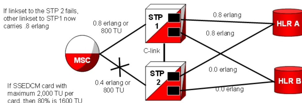
Figure 9: SIGTRAN: Failover at 0.8 Erlang
