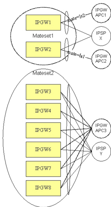
Figure 24: Eight IPGWx cards, two mates, three linksets
