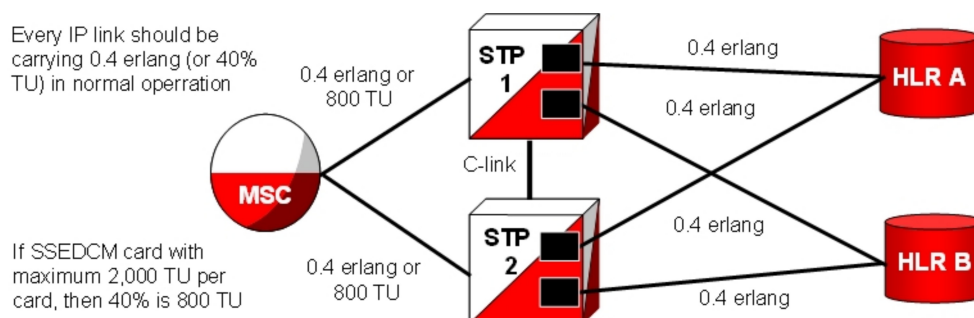
Figure 8: SIGTRAN: Every IP Link at 0.4 Erlang
