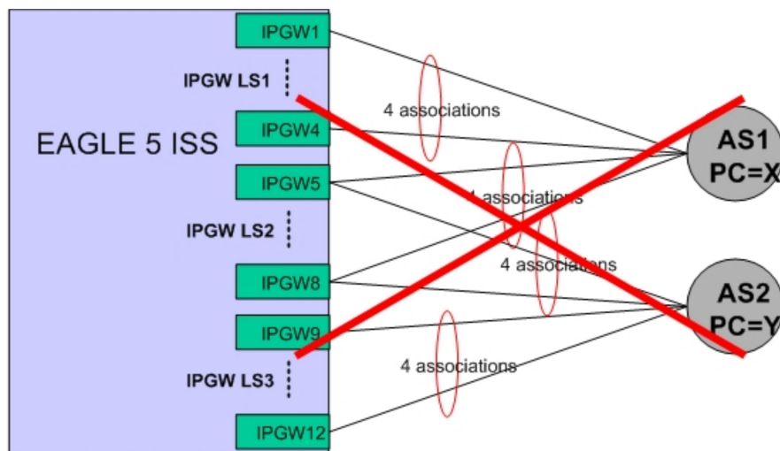
Figure 27: Unsupported deployment scenario: combined linksets (2)
