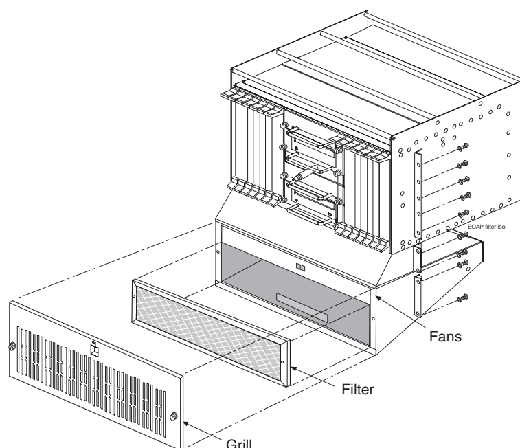
Figure 2-14. Fan Filter Replacement
