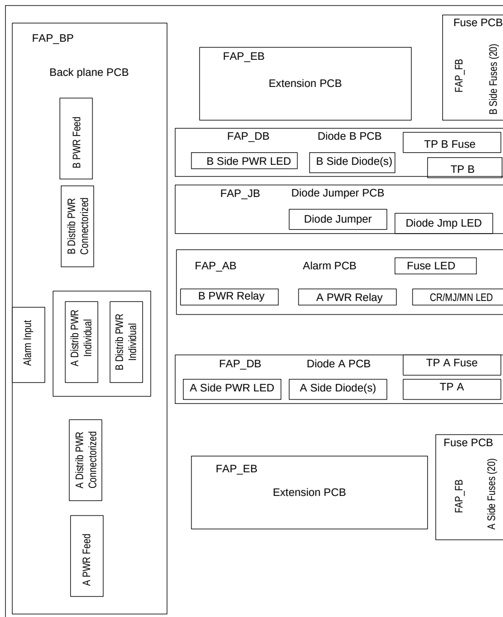
Figure 2-7.FAP Component Functions
