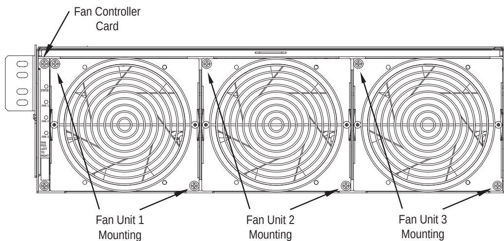
Figure A-24. Fan Unit Mounting Screws
