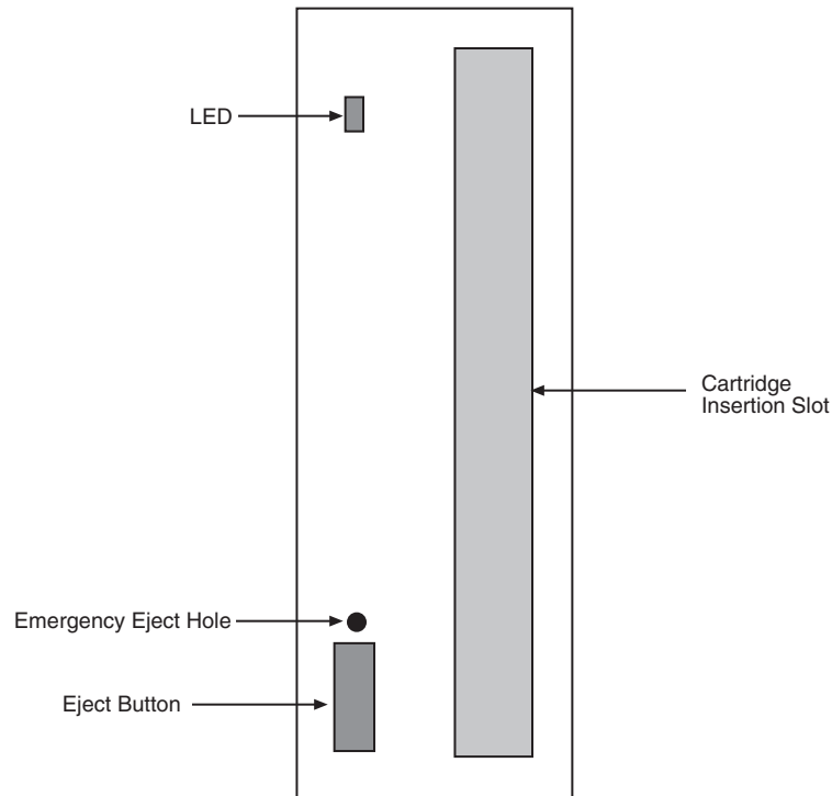
Figure 2-10.2.3 Gbyte Removable Cartridge Drive Layout
