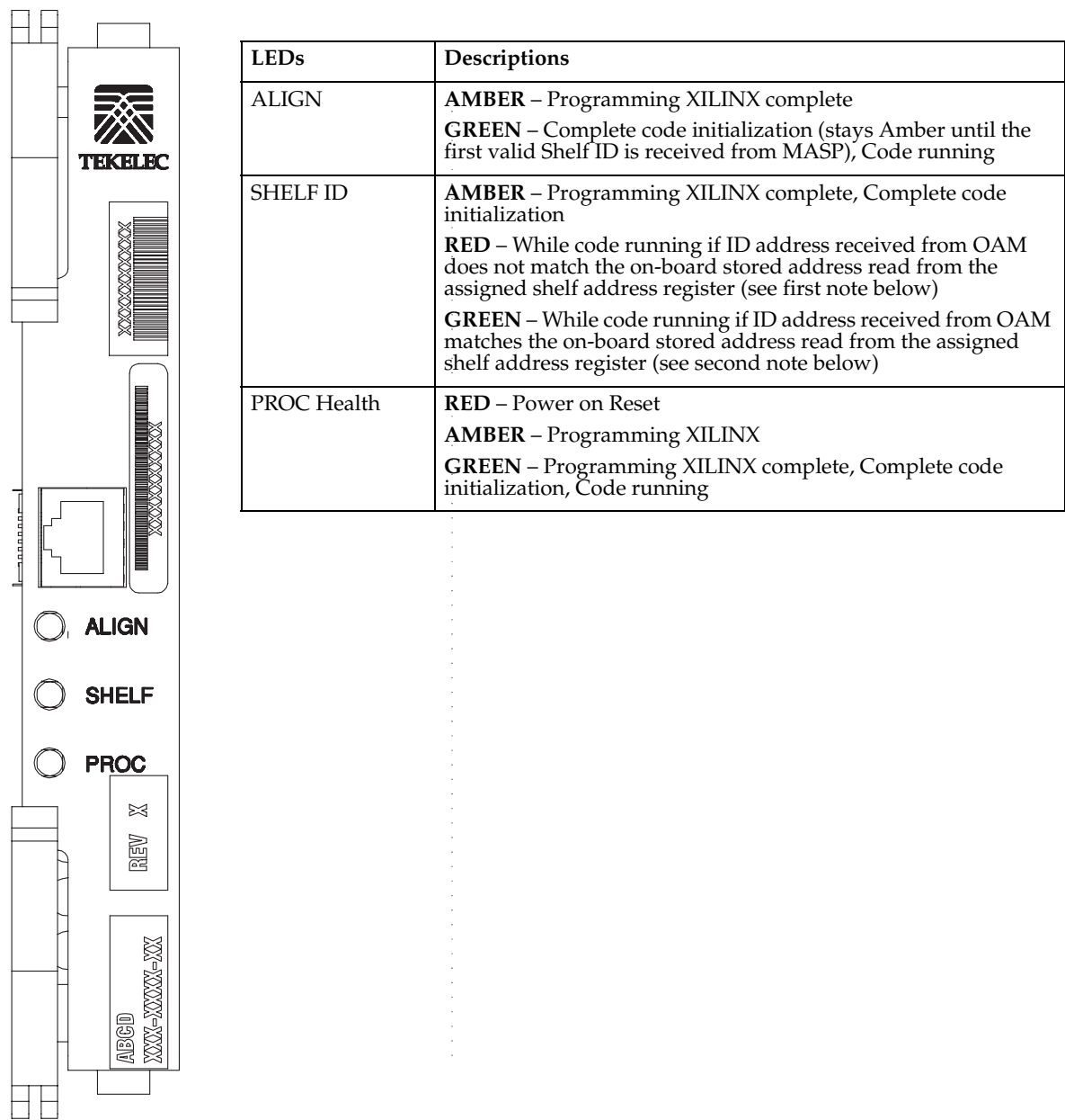
Figure A-3.HIPR LEDs
