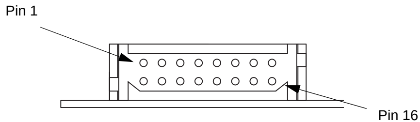
Figure 2-5. Diode Board Edge Connector J1.
