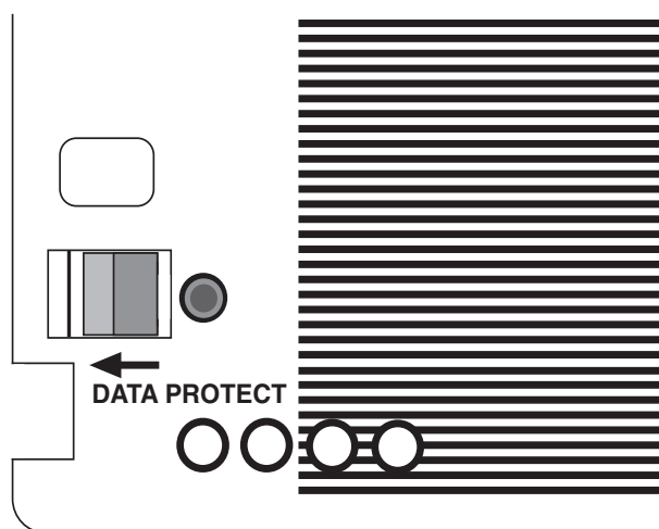
Figure 2-9.2.3 Gbyte Write Enabled Removable Cartridge
