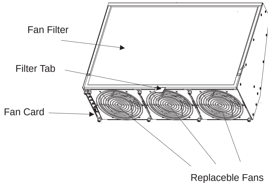
Figure 2-13.Fan Assembly
