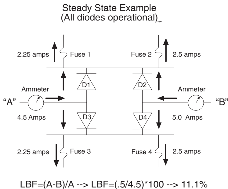
Figure 2-12.Steady State Example
