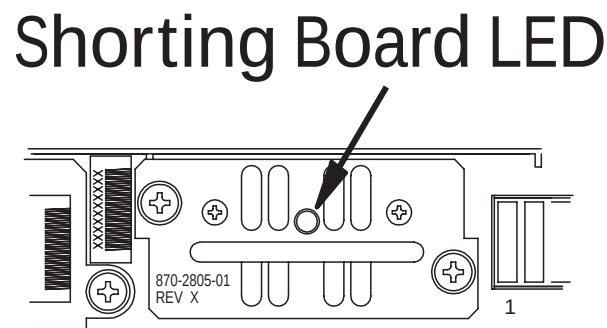
Figure 2-2. Shorting Board Faceplate, Operational Mode
