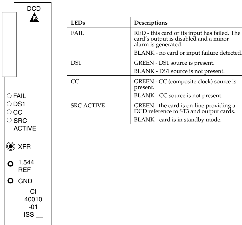
Figure A-19. Holdover Clock CI Card LEDs
