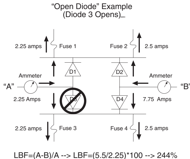
Figure 2-11. Open Diode Example
