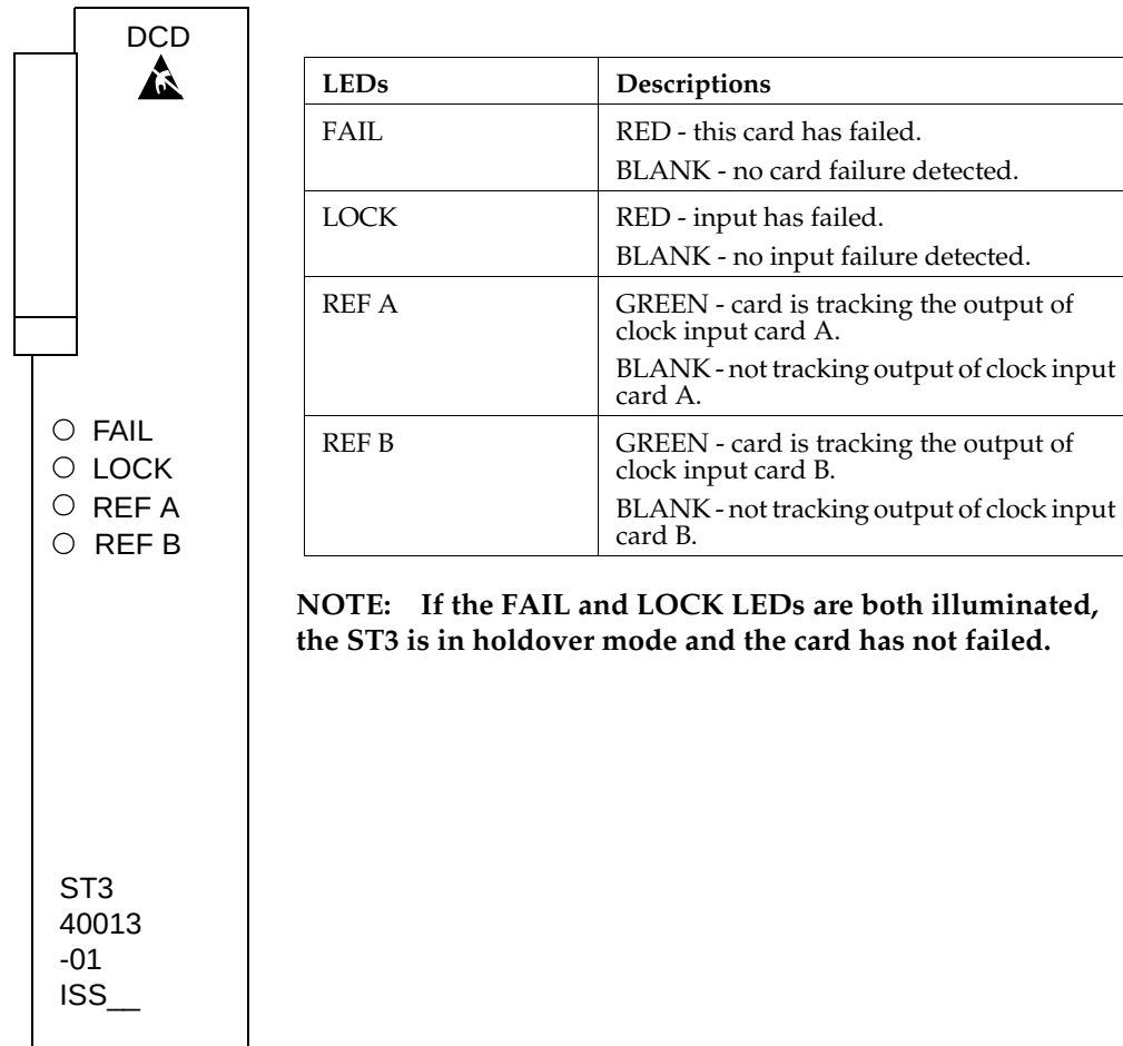
Figure A-20. Holdover clock ST3 card LEDs
