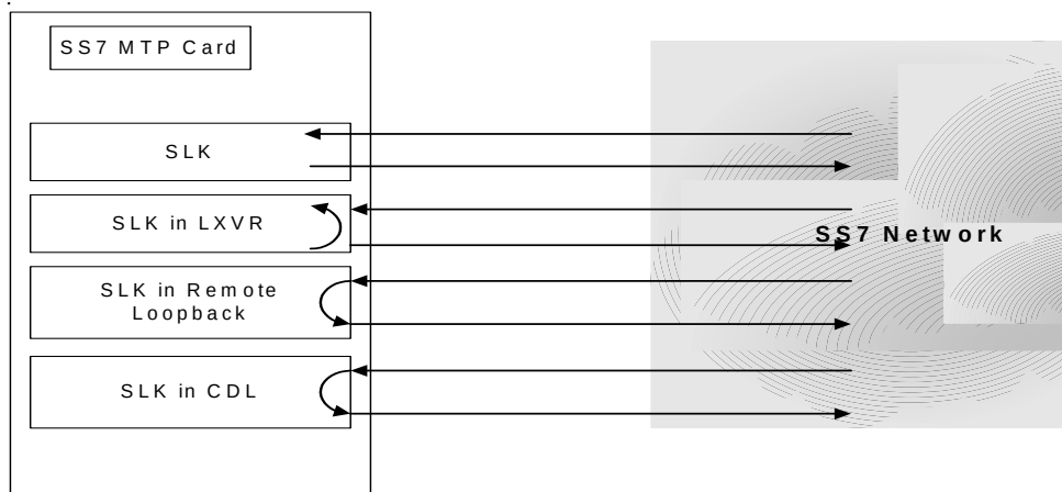
Figure 3-10. Signaling Link Network Connections
