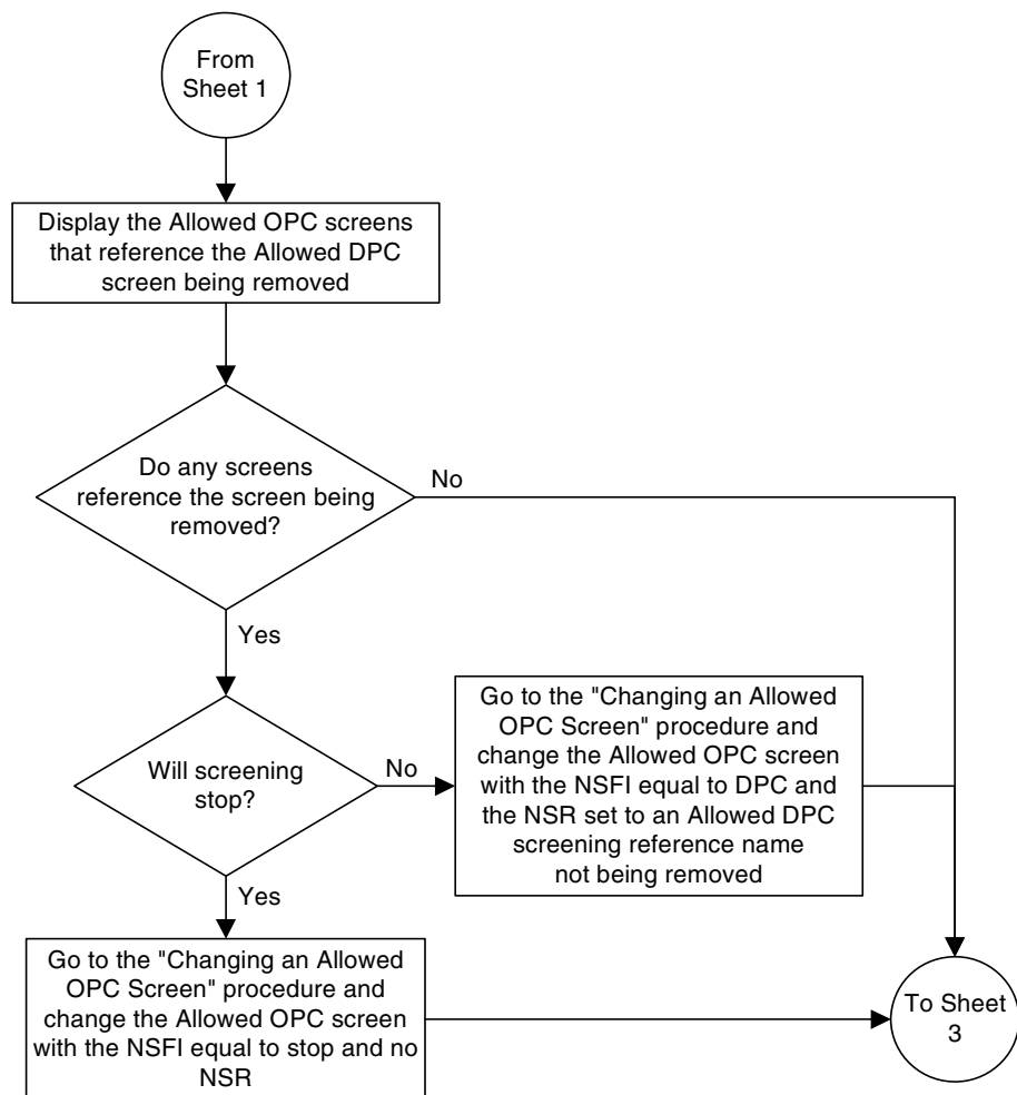
Flowchart 5-20. Removing an Allowed DPC Screen from the SEAS Terminal (Sheet 2 of 4)
