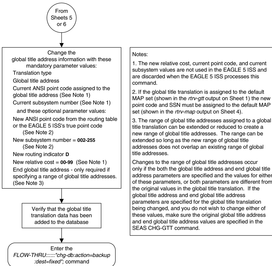
Flowchart 4-6. Changing a Global Title Translation (Sheet 7 of 7)
