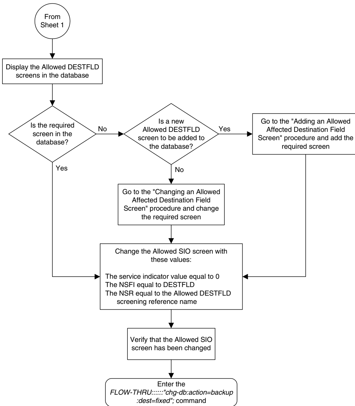
Flowchart 5-24. Changing an Allowed SIO Screen from the SEAS Terminal (Sheet 4 of 7)
