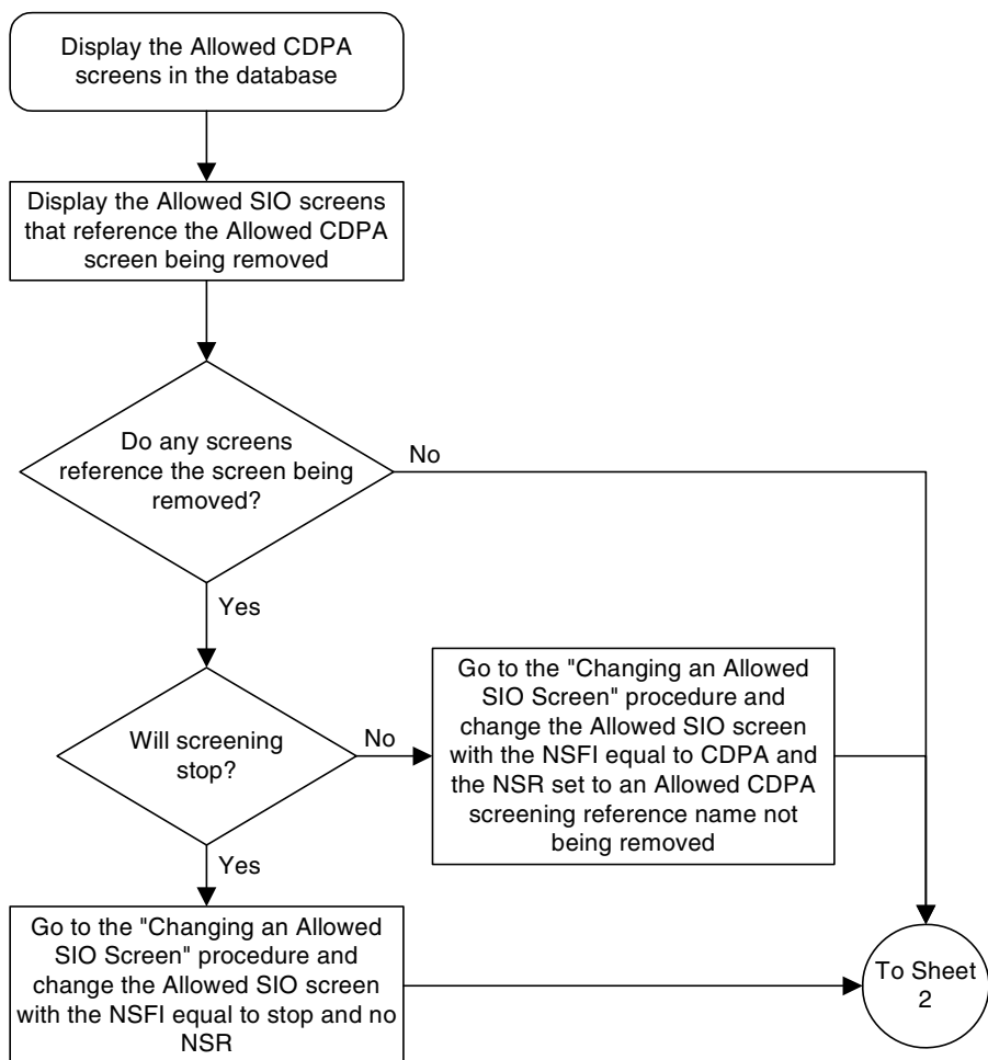
Flowchart 5-5. Removing an Allowed Called Party Address Screen from the SEAS Terminal (Sheet 1 of 3)
