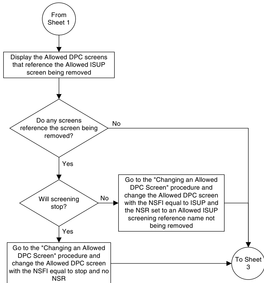
Flowchart 5-37. Removing an Allowed ISUP Message Type Screen from the SEAS Terminal (Sheet 2 of 3)
