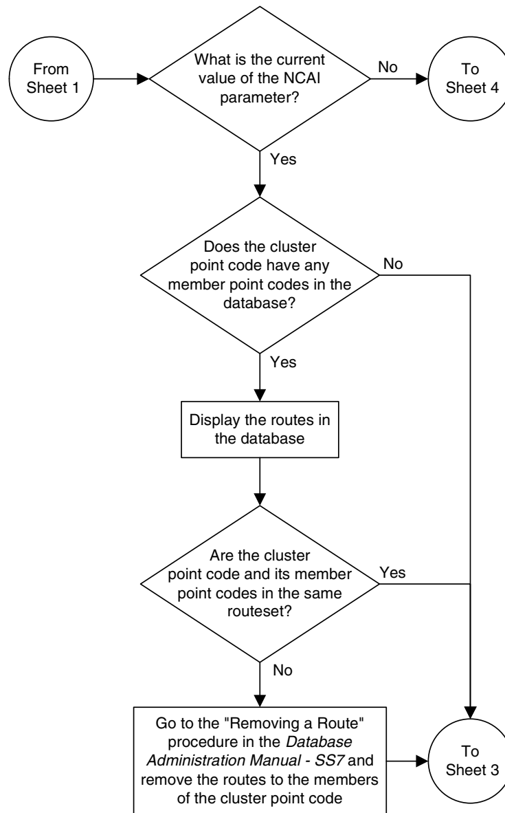
Flowchart 2-2. Changing the Attributes of a Cluster Point Code from the SEAS Terminal (Sheet 2 of 4)
