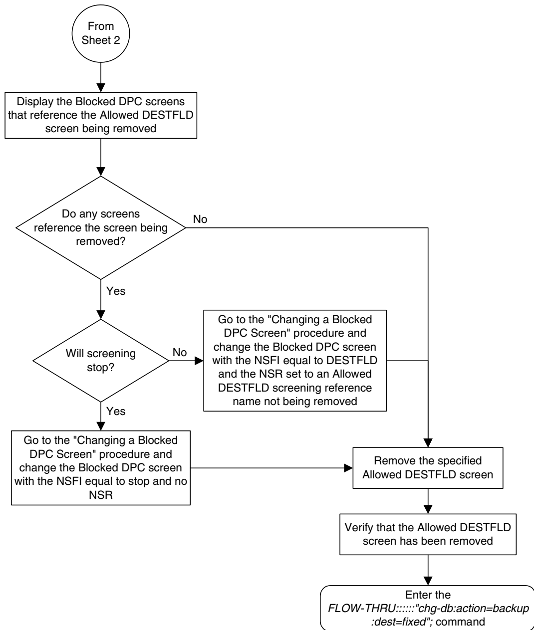
Flowchart 5-14. Removing an Allowed Affected Destination Screen from the SEAS Terminal (Sheet 3 of 3)
