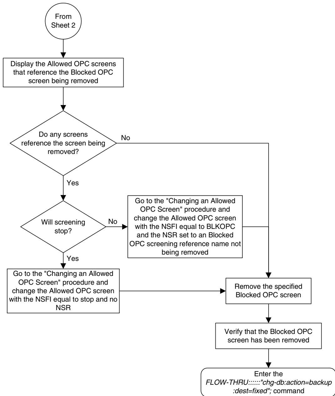
Flowchart 5-26. Removing a Blocked OPC Screen from the SEAS Terminal (Sheet 2 of 2)
