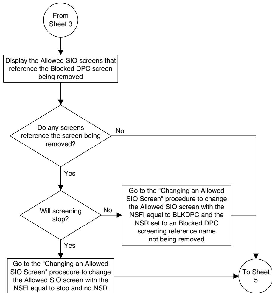
Flowchart 5-17. Removing a Blocked DPC Screen from the SEAS Terminal (Sheet 4 of 5)
