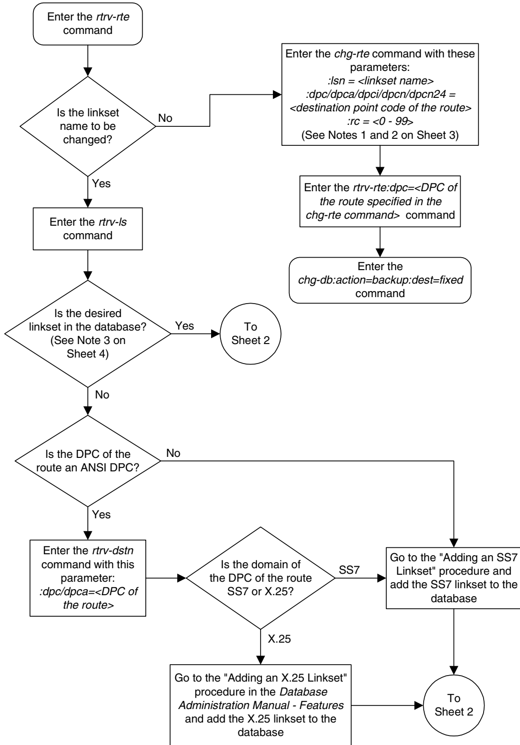
Flowchart 3-13. Changing a Route (Sheet 1 of 4)
