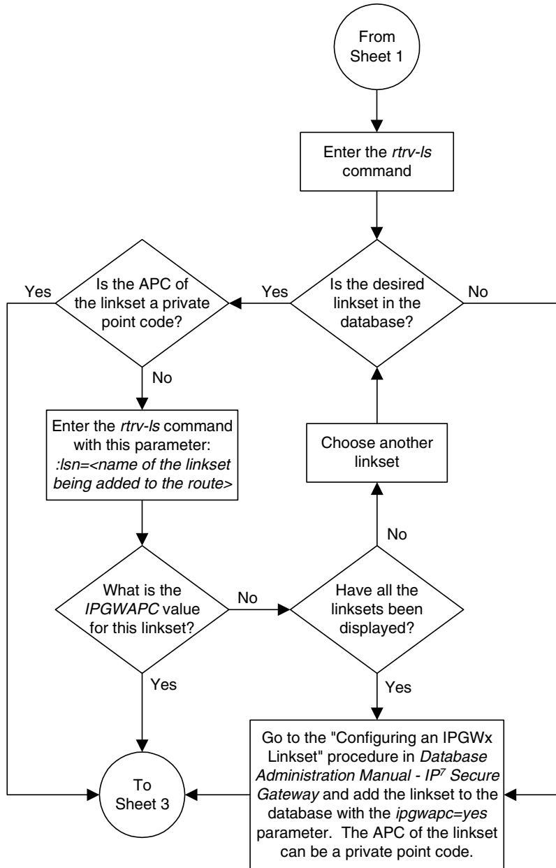
Flowchart 3-10. Adding a Route Containing an IPGWx Linkset (Sheet 2 of 3)
