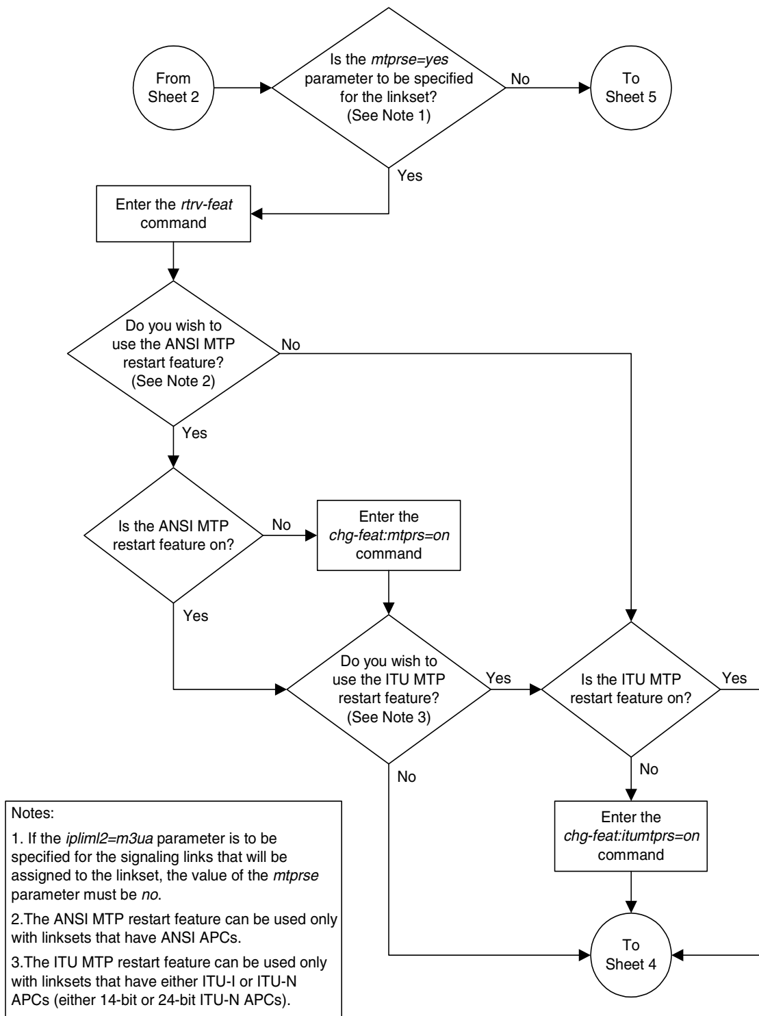
Flowchart 3-2. Adding an SS7 Linkset (Sheet 3 of 11)
