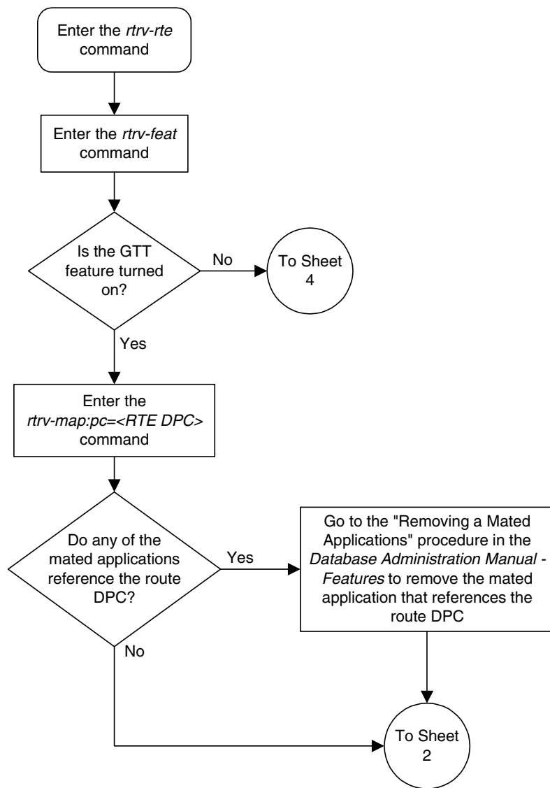
Flowchart 3-12. Removing a Route (Sheet 1 of 7)
