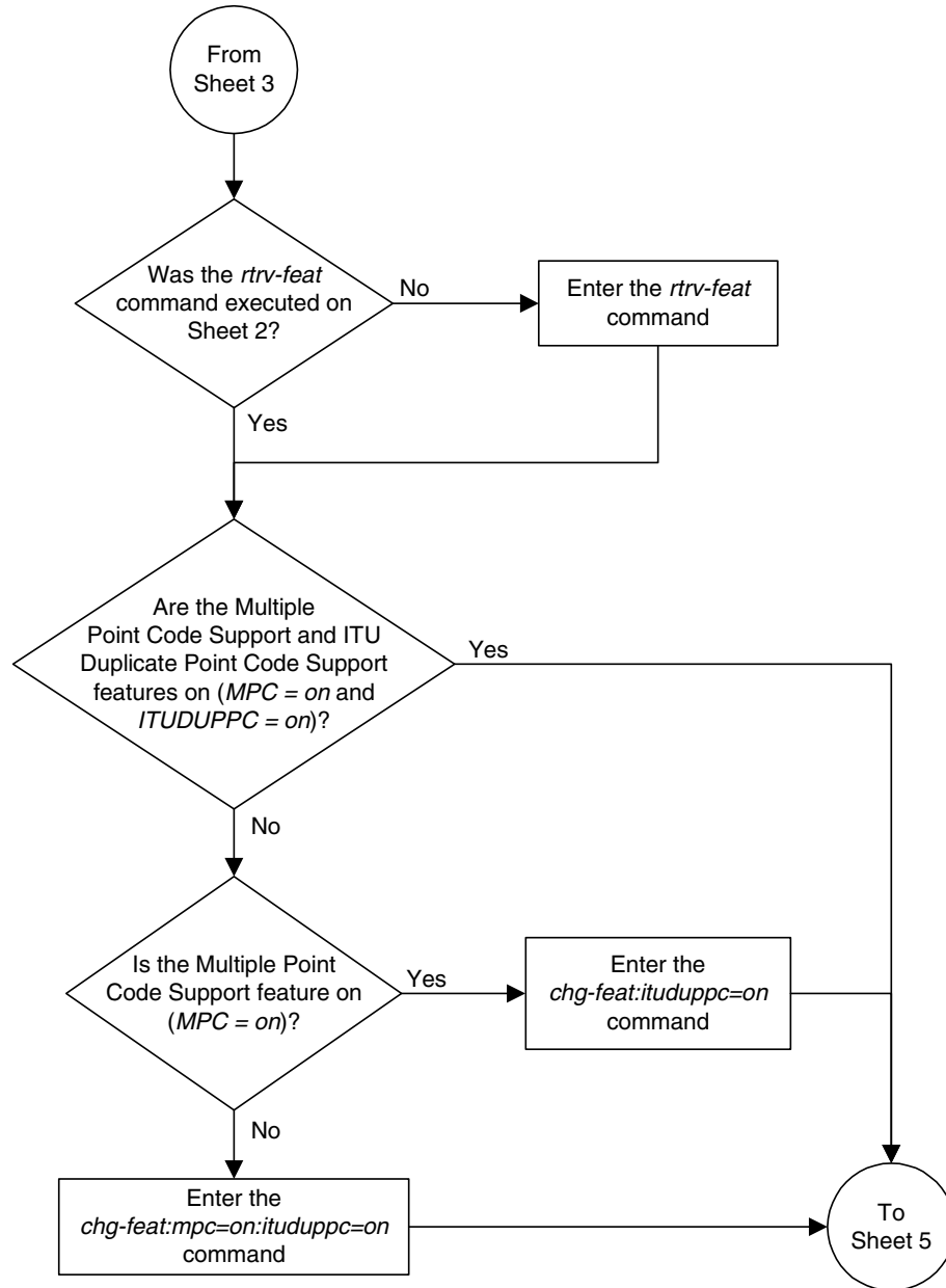
Flowchart 2-7. Changing the Self-Identification of the System (Sheet 4 of 11)
