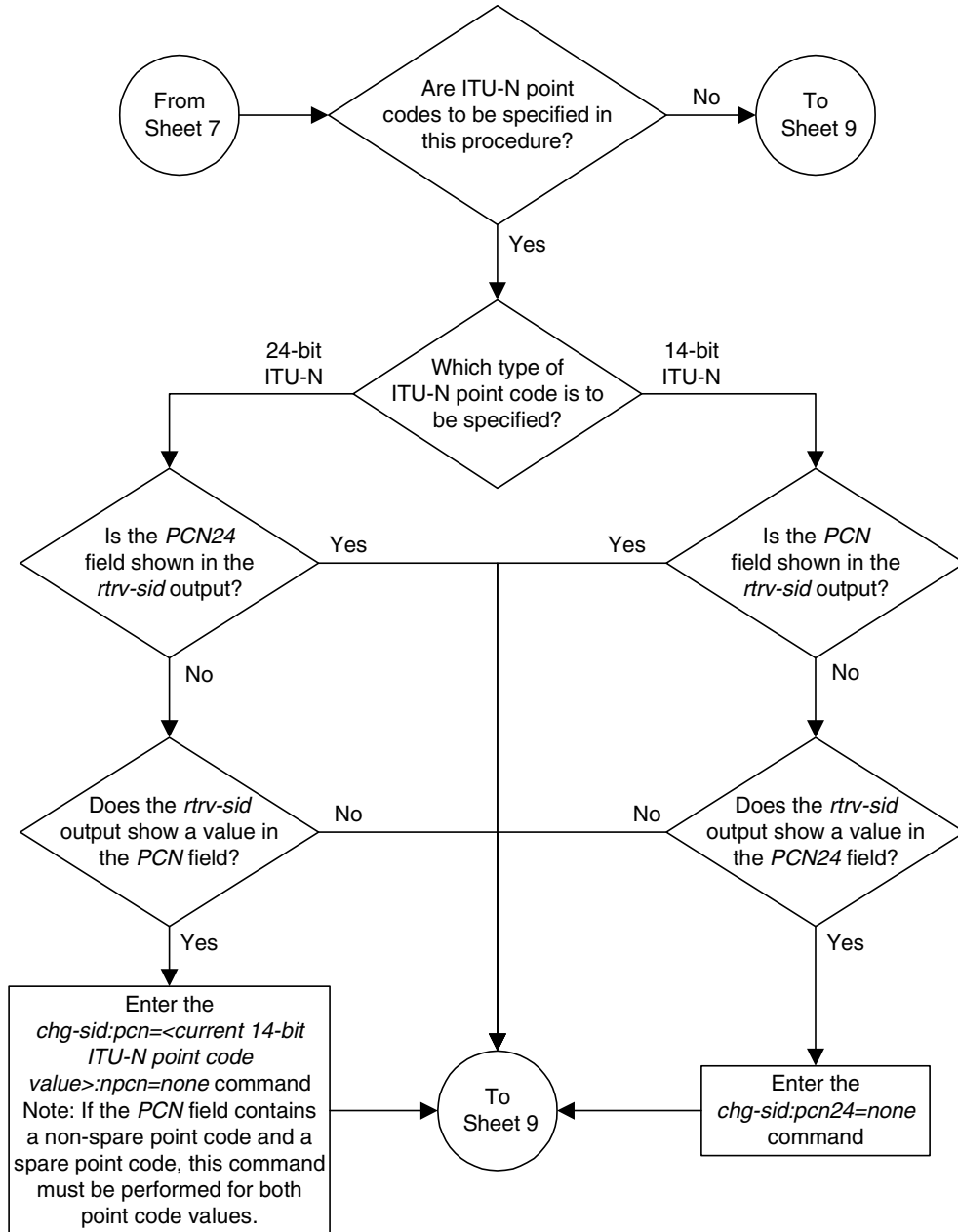
Flowchart 2-7. Changing the Self-Identification of the System (Sheet 8 of 11)
