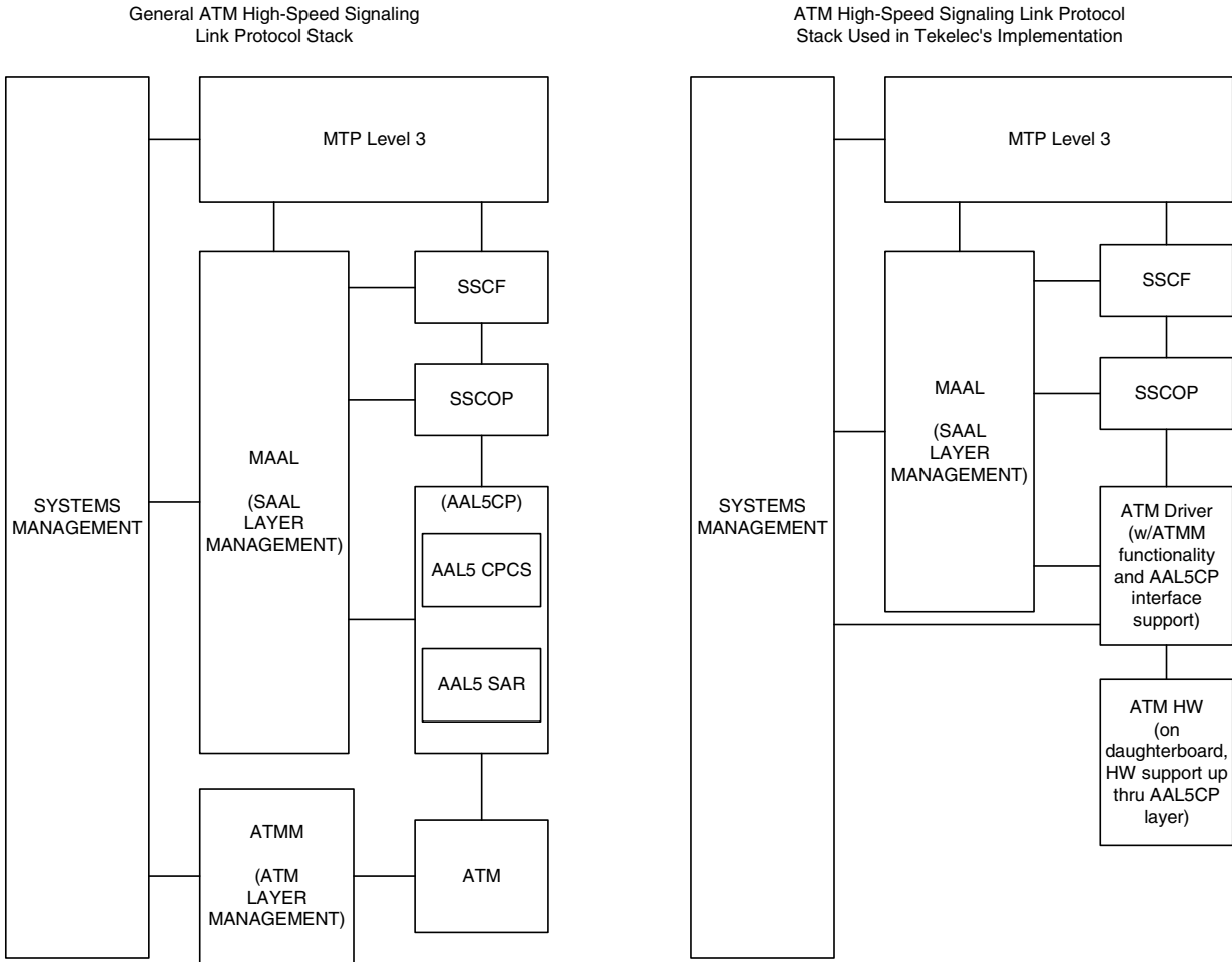
Figure C-2. ATM High-Speed Signaling Link Protocol Stack vs. Tekelec Implementation in the EAGLE 5 SAS
