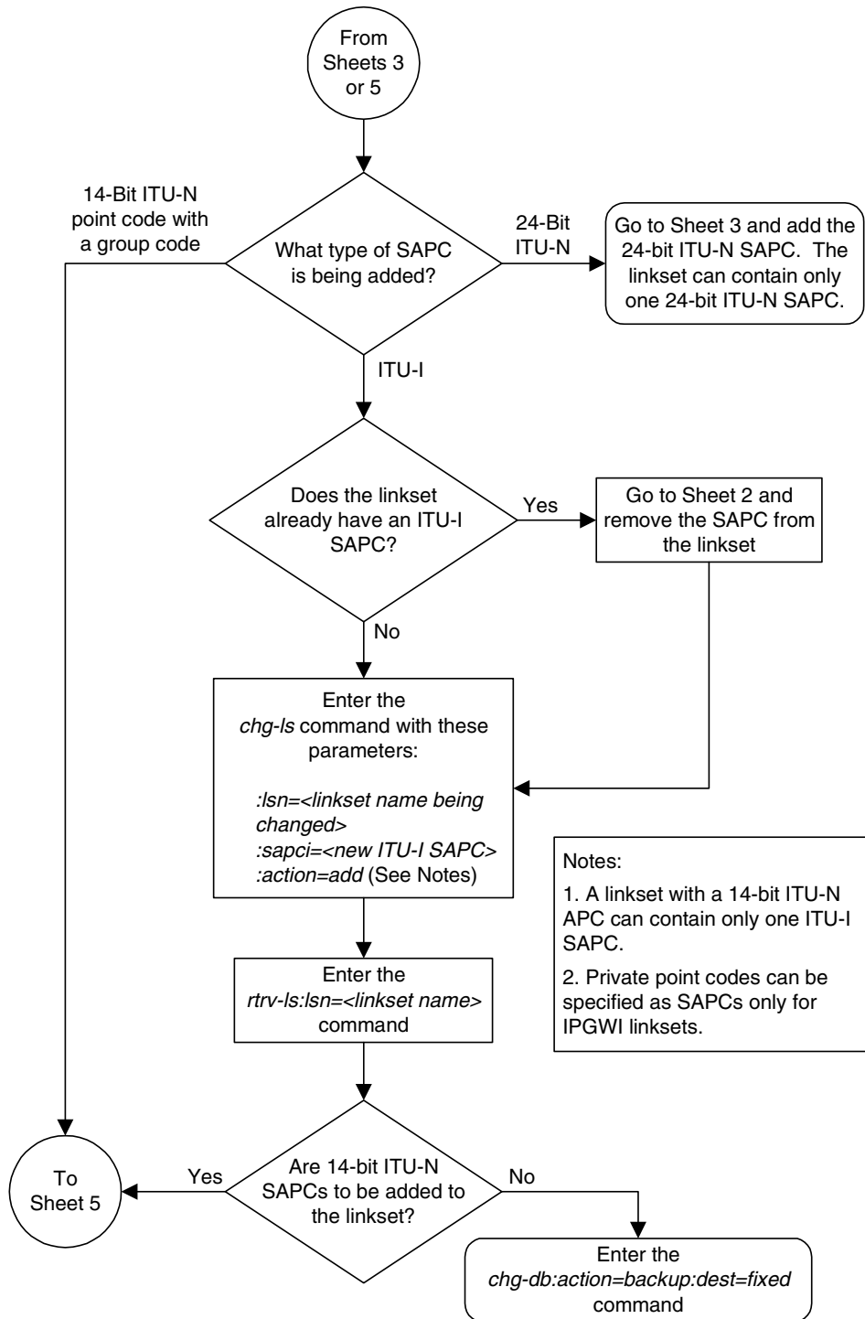
Flowchart 3-5. Configuring an ITU Linkset with a Secondary Adjacent Point Code (SAPC) (Sheet 4 of 5)
