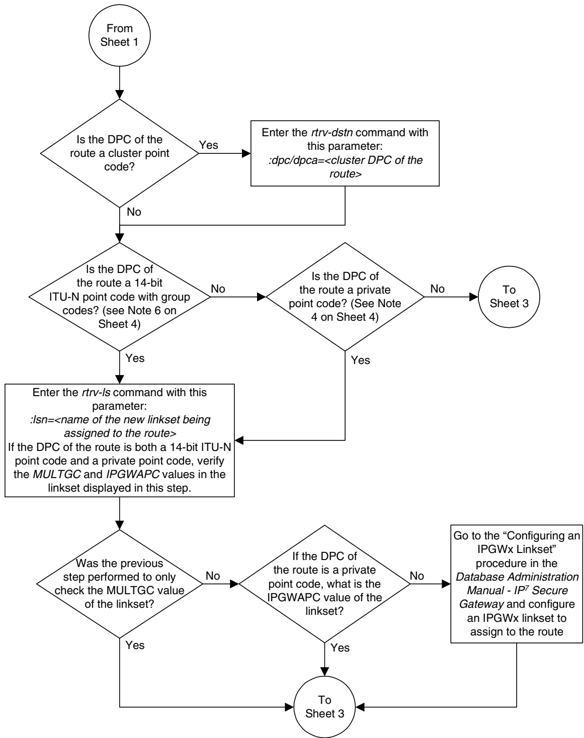
Flowchart 3-13. Changing a Route (Sheet 2 of 4)
