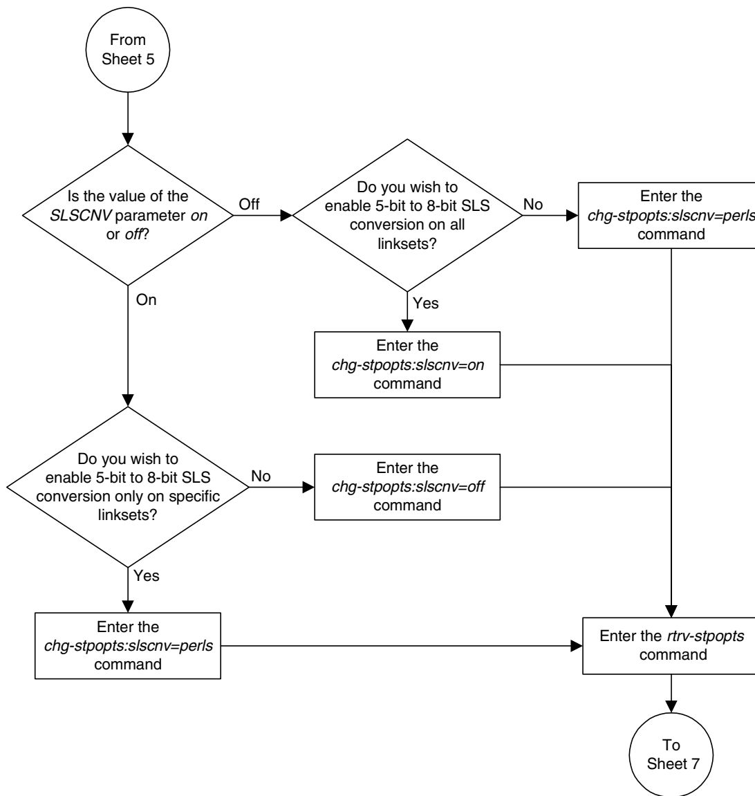
Flowchart 3-4. Changing an SS7 Linkset (Sheet 6 of 14)
