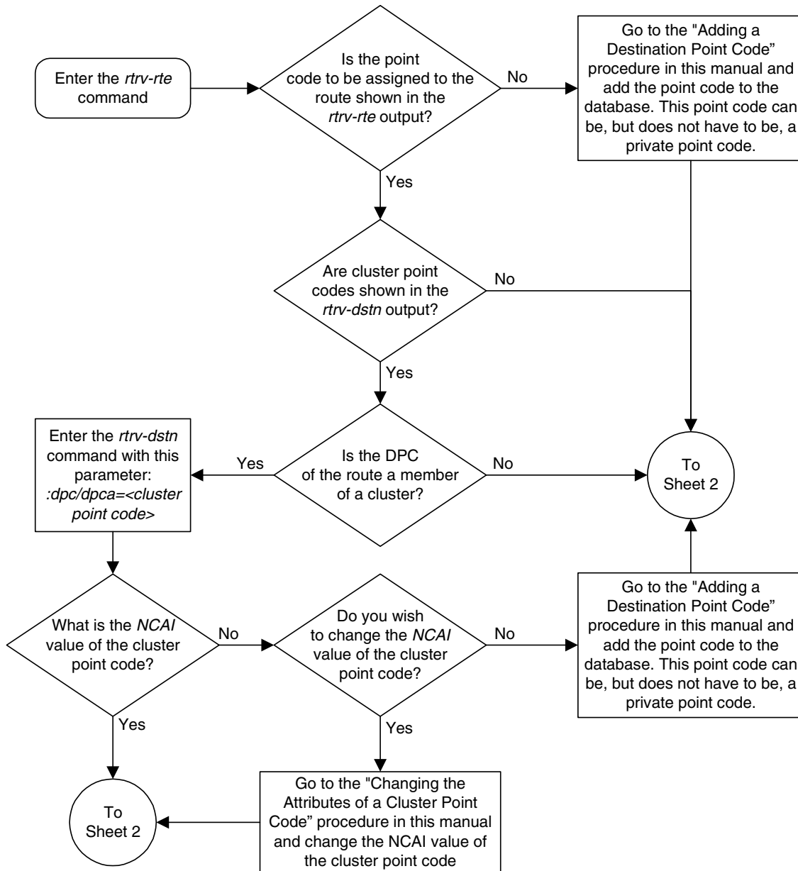
Flowchart 3-10. Adding a Route Containing an IPGWx Linkset (Sheet 1 of 3)
