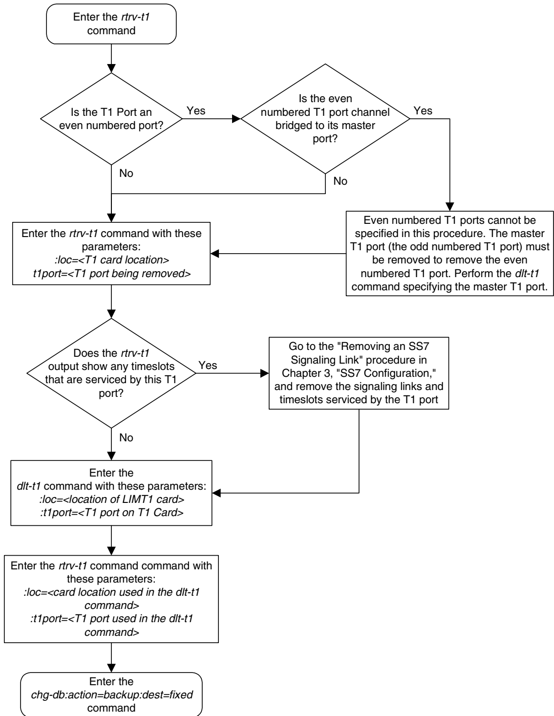
Flowchart B-4. Removing the T1 Interface Parameters
