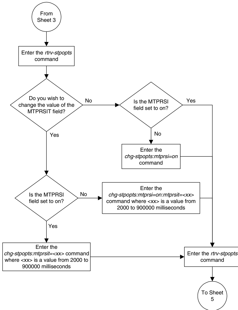
Flowchart 3-2. Adding an SS7 Linkset (Sheet 4 of 11)
