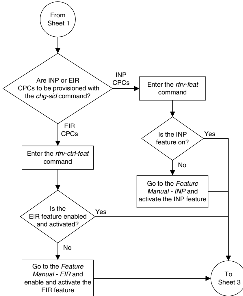
Flowchart 2-7. Changing the Self-Identification of the System (Sheet 2 of 11)
