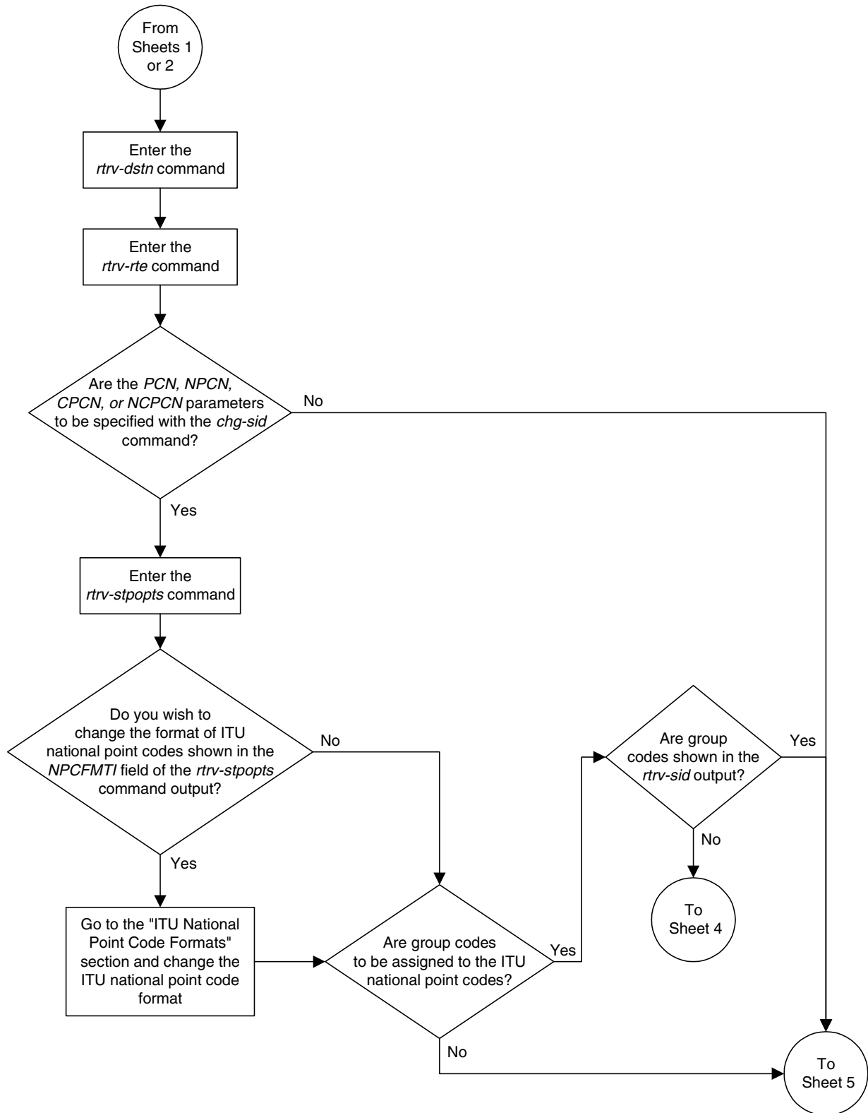
Flowchart 2-7. Changing the Self-Identification of the System (Sheet 3 of 11)
