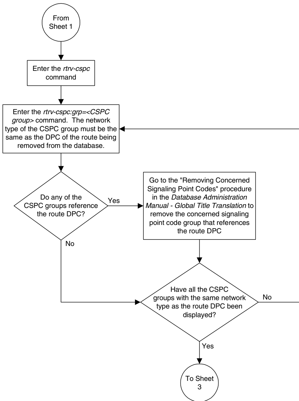
Flowchart 3-12. Removing a Route (Sheet 2 of 7)
