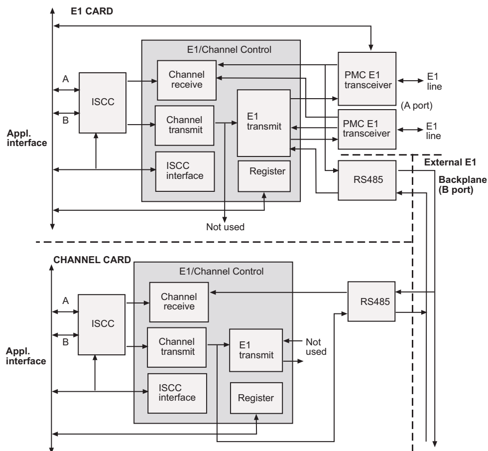
Figure A-1. LIM-E1 Block Diagram
