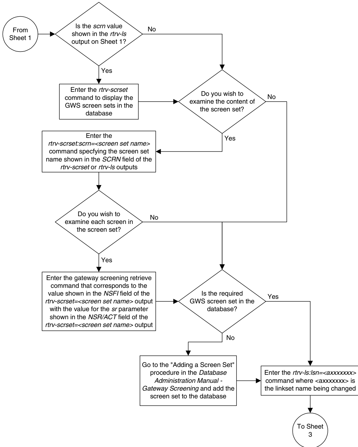
Flowchart 3-4. Changing an SS7 Linkset (Sheet 2 of 14)
