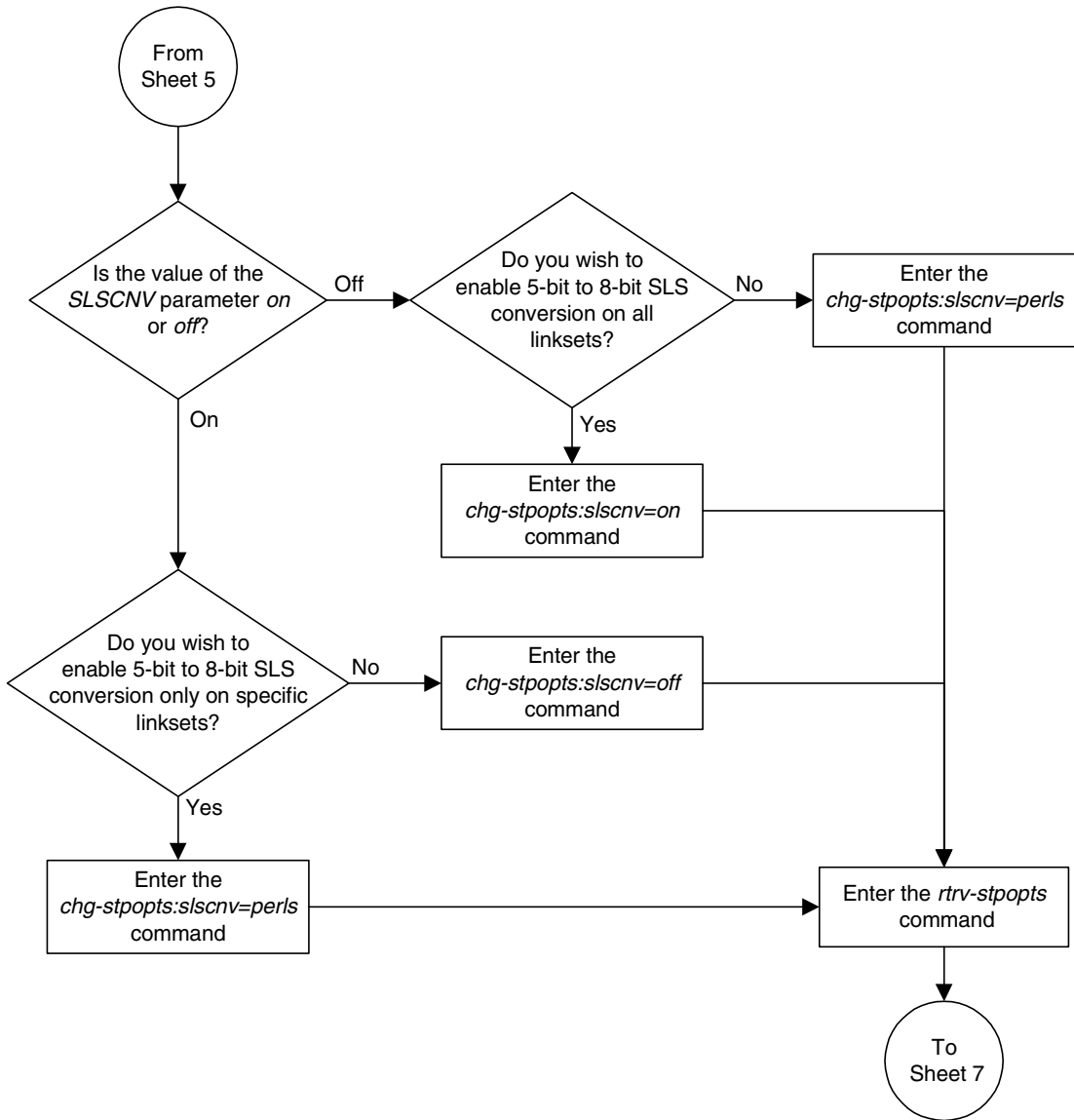
Flowchart 3-2. Adding an SS7 Linkset (Sheet 6 of 11)
