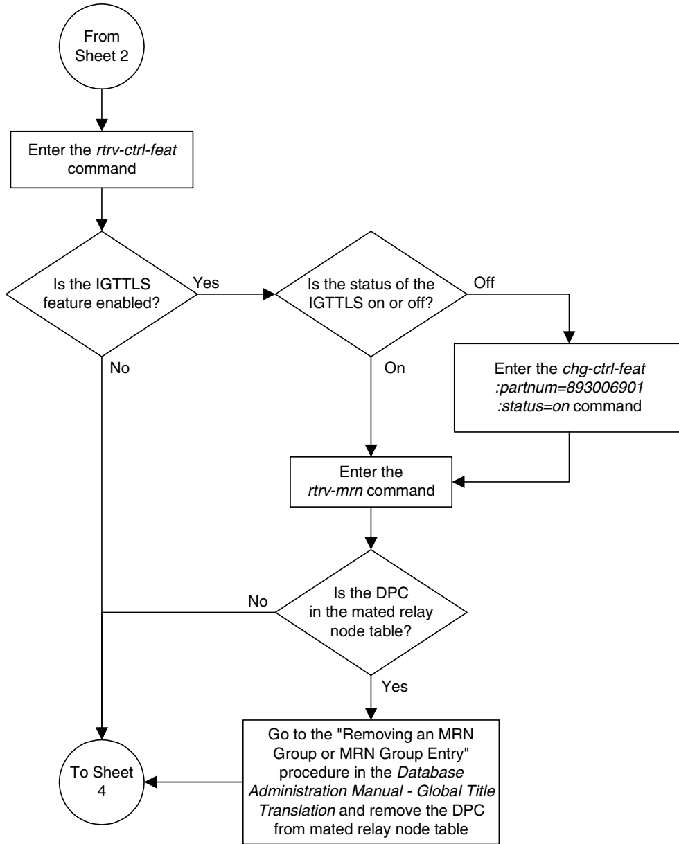
Flowchart 3-12. Removing a Route (Sheet 3 of 7)
