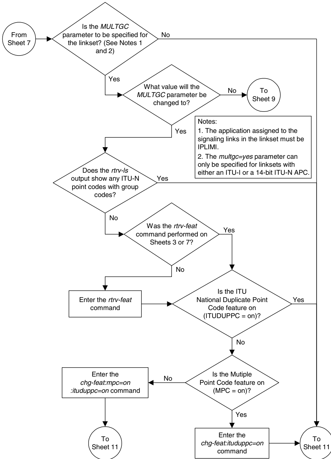
Flowchart 3-4. Changing an SS7 Linkset (Sheet 8 of 14)
