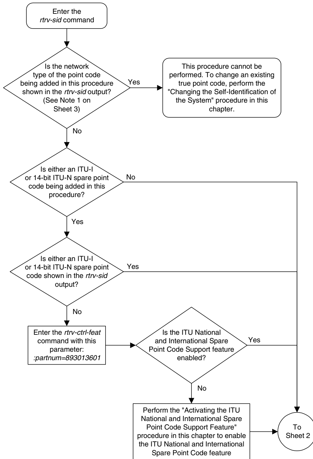
Flowchart 2-6. Adding a Point Code to the Self-Identification of the EAGLE 5 SAS (Sheet 1 of 3)
