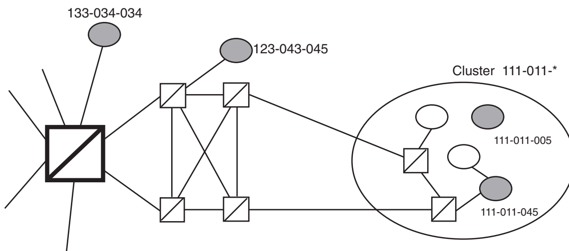
Figure 2-8. Cluster Routing and Management Diversity
