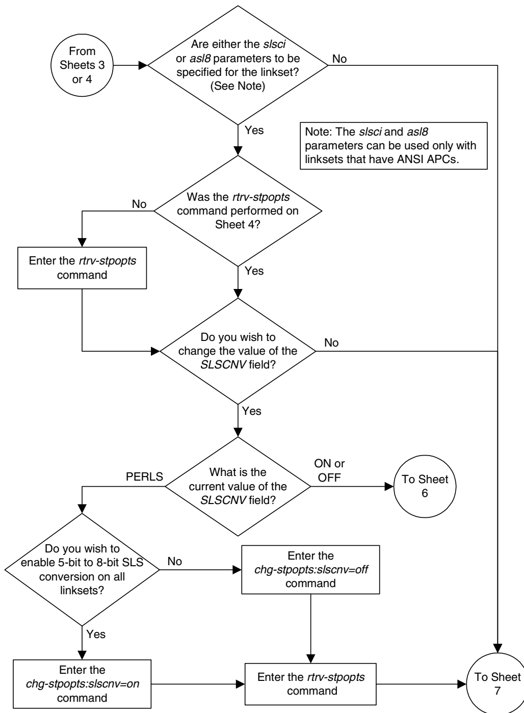
Flowchart 3-2. Adding an SS7 Linkset (Sheet 5 of 11)
