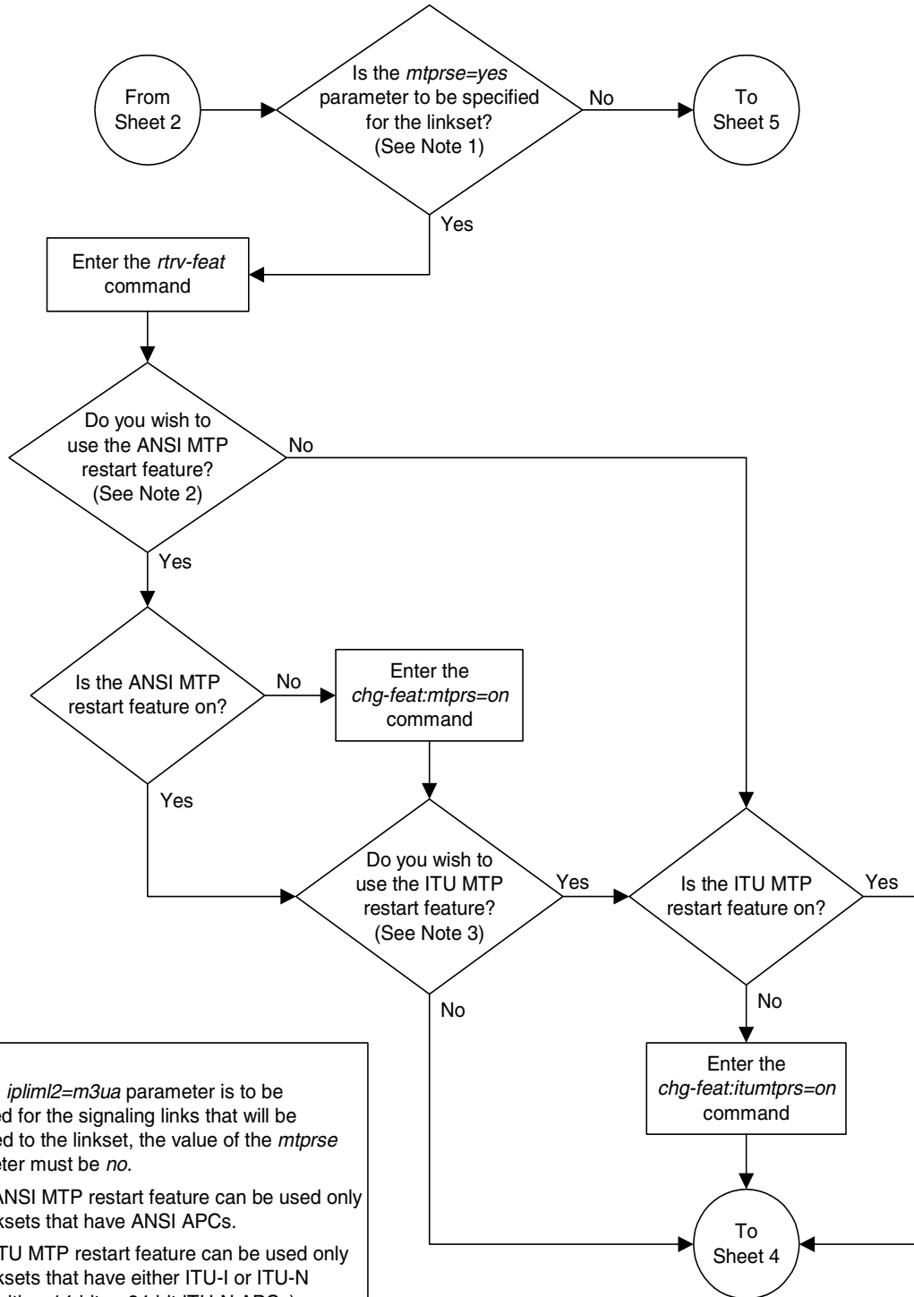
Flowchart 3-4. Changing an SS7 Linkset (Sheet 3 of 14)
