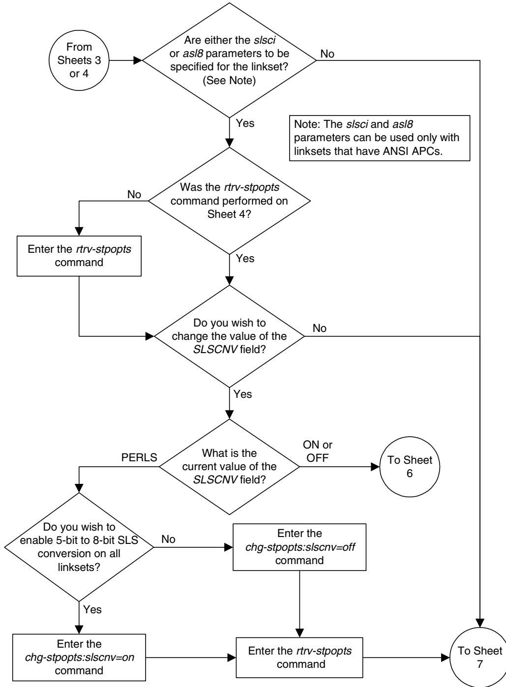
Flowchart 3-4. Changing an SS7 Linkset (Sheet 5 of 14)
