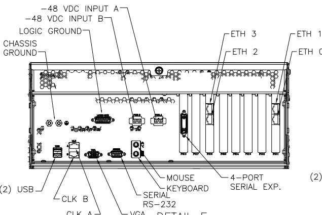
DETAIL F SERVER A REAR VIEW 870-2640-01 W/ PCI CARDS: SLOT 1 -870-2706-02 SLOT 6 -870-2706-02 SLOT 8 -870-2708-01
