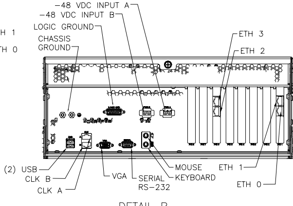
DETAIL B SERVER 1B - 1E (REAR VIEW) 870-2640-01 W/ PCI CARDS: SLOT 1 -870-2706-02 SLOT 6 -870-2706-02
